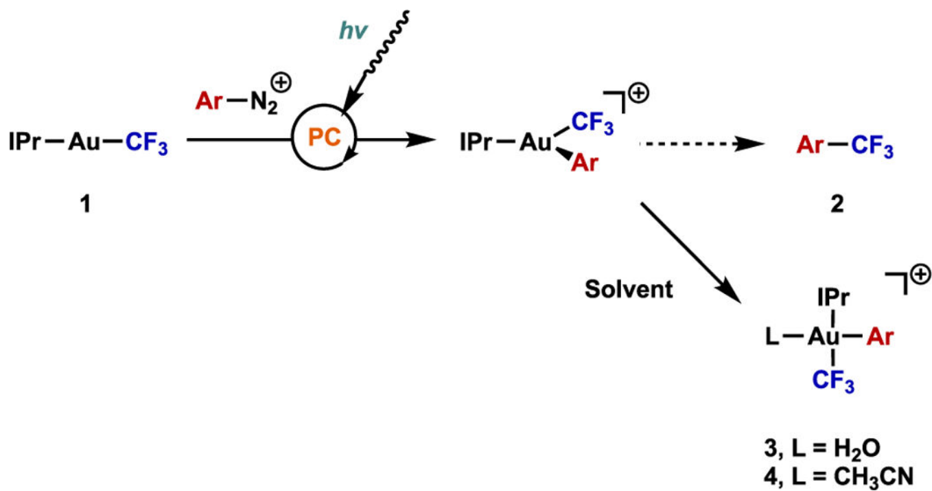
Scheme 2. Intercepted Gold(III)-CF 3 Intermediates a
