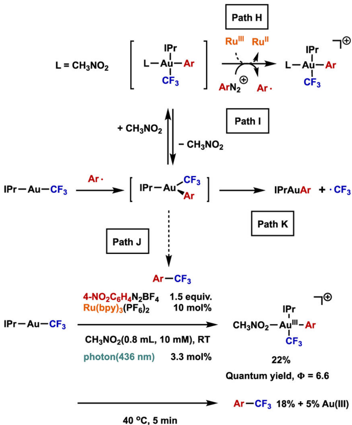
Figure 6. (Top) Revised reaction mechanism of oxidative addition. The major operating pathway is path I. Path J was not observed. (Bottom) Quantum yield and reductive elimination of \text{CH}_3\text{NO}_2 -bound gold(III) intermediate. Yields are reported in triplicate.
