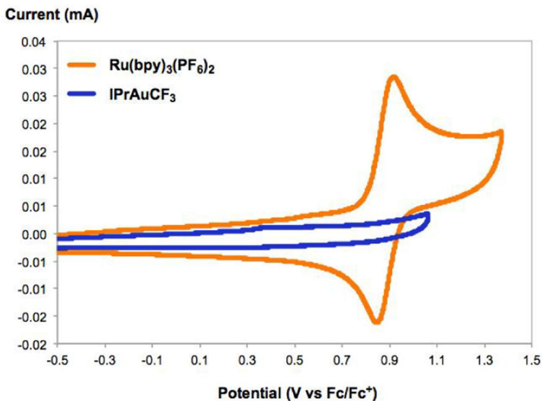
Figure 5. (Top) Two possible reaction mechanisms of oxidative addition. (Bottom) Cyclic voltammogram of Ru(bpy) 3 (PF 6 ) 2 and IPrAuCF 3 , scan rate = 100 mV/s.
