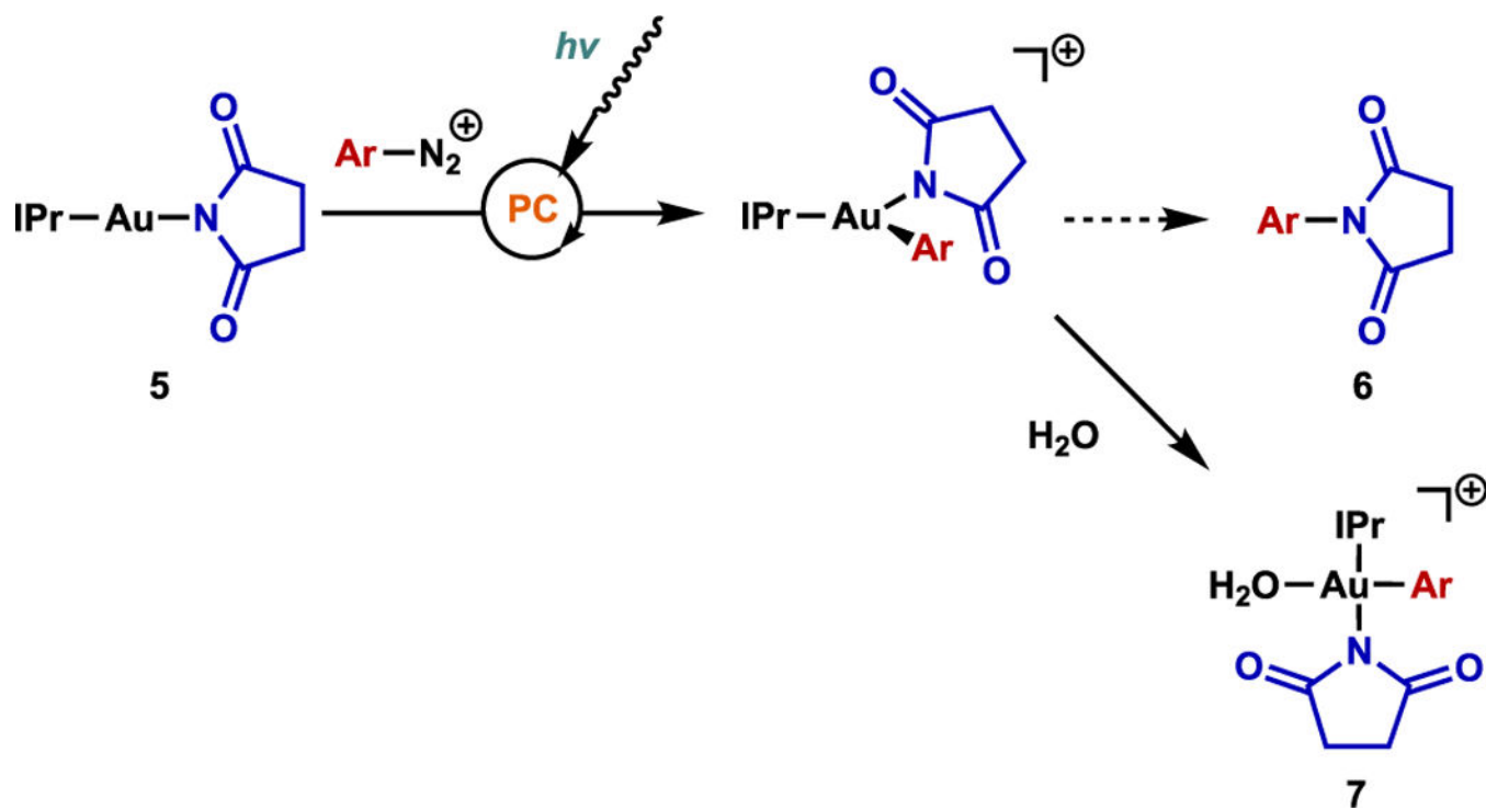
Scheme 5. Intercepted Gold(III)-Succinimide Intermediate a
