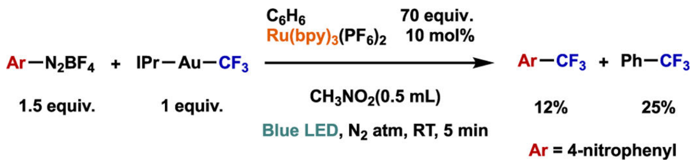
Scheme 3. Radical Trapping Experiment
