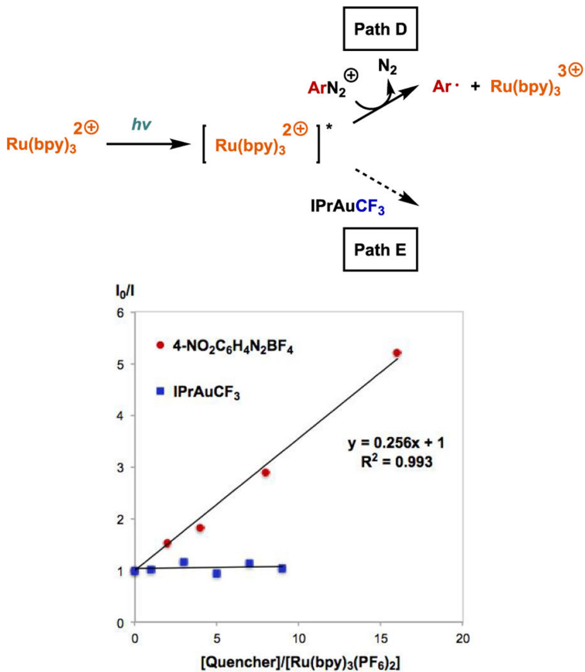
Figure 4. (Top) Two possible modes of photoluminescence quenching. Path E was ruled out. (Bottom) Stern–Volmer relationship. [\text{Ru}(\text{bpy})_3(\text{PF}_6)_2] = 0.05 \text{ mM} in \text{CH}_3\text{NO}_2 .
