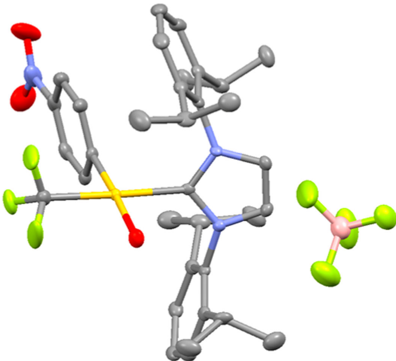
Figure 2. Crystal structure of 3-BF 4 . Thermal ellipsoid plot is drawn at 50% probability. Hydrogen atoms and solvents are omitted for clarity.
