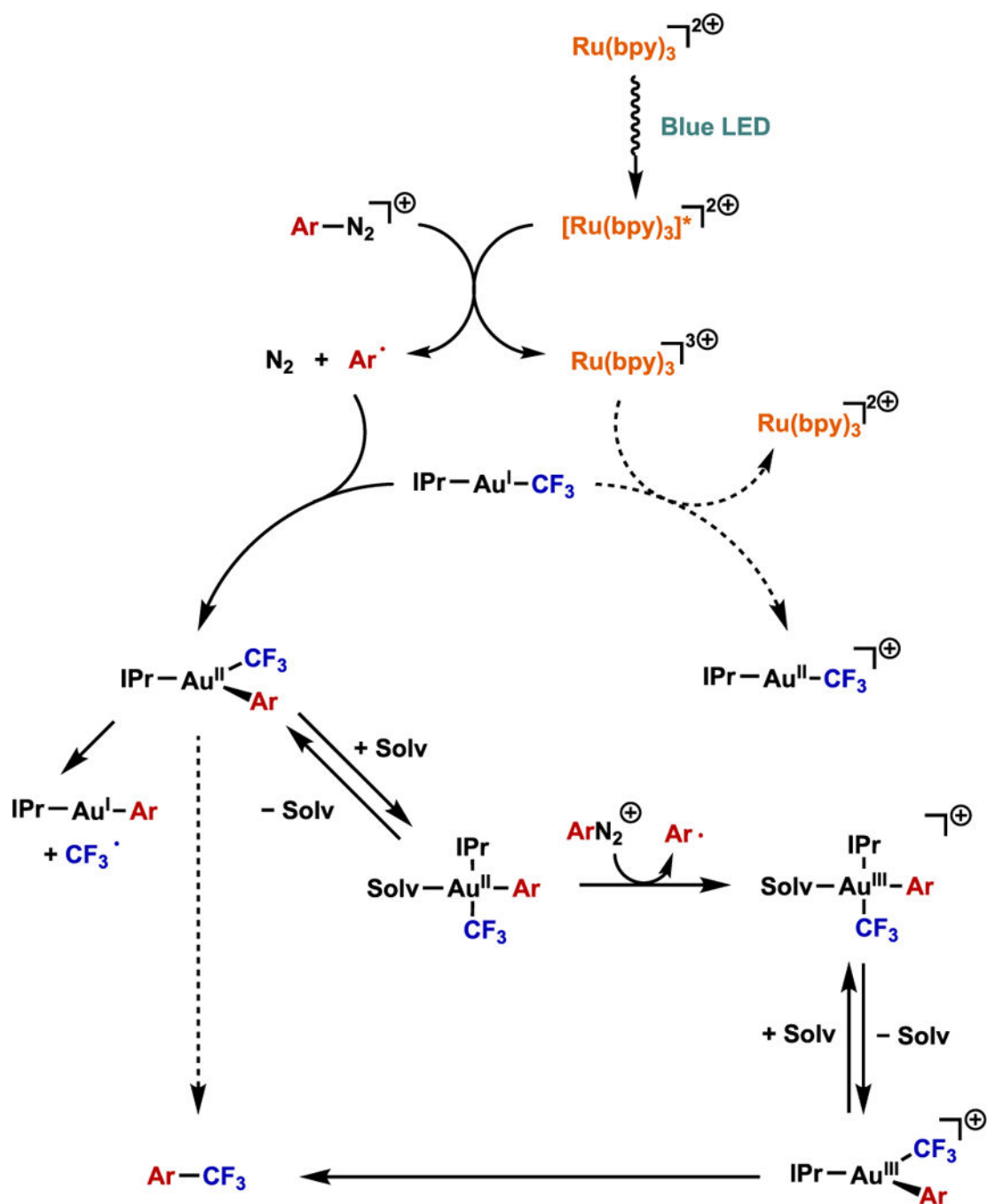
Figure 8. Summary of proposed reaction mechanism, Solv = \text{CH}_3\text{NO}_2 .
