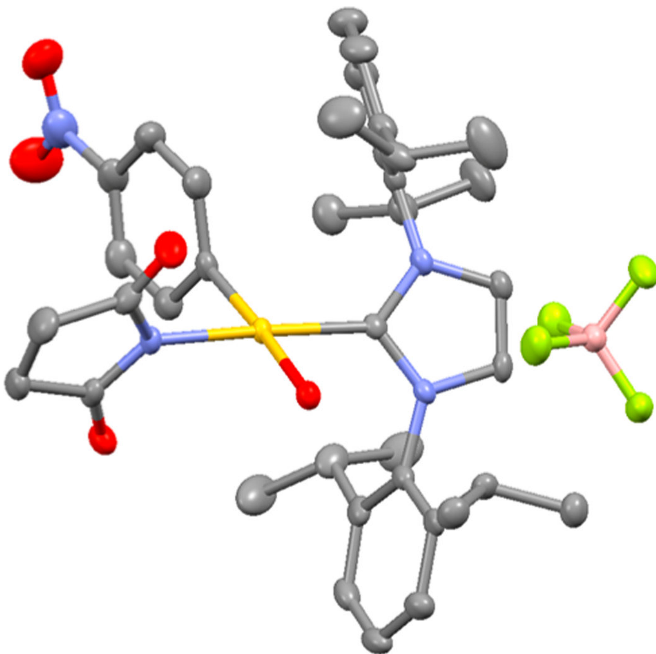
Figure 7. Crystal structure of 7-BF 4 . Thermal ellipsoid plot is drawn at 50% probability. Hydrogen atoms and solvents are omitted for clarity.
