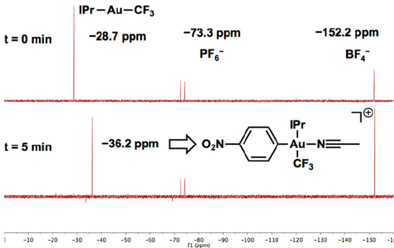
Figure 1. ^{19}\text{F} NMR spectra of gold-mediated \text{C}(\text{sp}^2)-\text{CF}_3 coupling reaction, solvent = \text{CH}_3\text{CN} .
