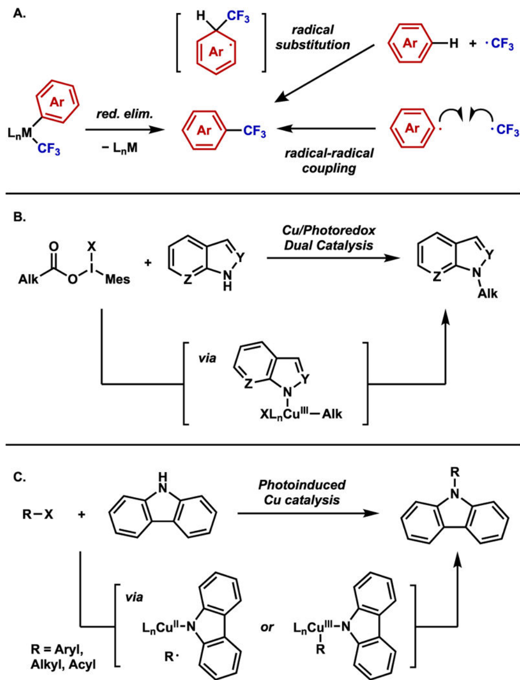
Scheme 1. Potential Bond-Forming Steps of Metallaphotoredox Catalysis (A) Copper(III) Intermediates Proposed for Photochemical C–N Coupling Reactions (B and C)
