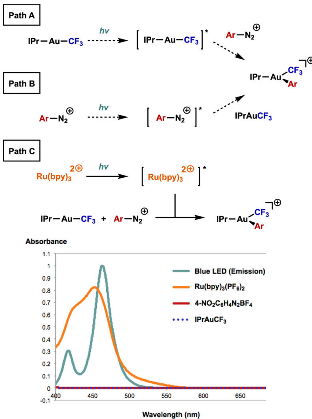
Figure 3. (Top) Three possible modes of sensitization with visible light. Paths A and B were ruled out. (Bottom) UV-vis absorption spectra of all chemicals (concentration = 0.05 mM in \text{CH}_3\text{NO}_2 ) and emission spectrum of the light source, Kessil H150.
