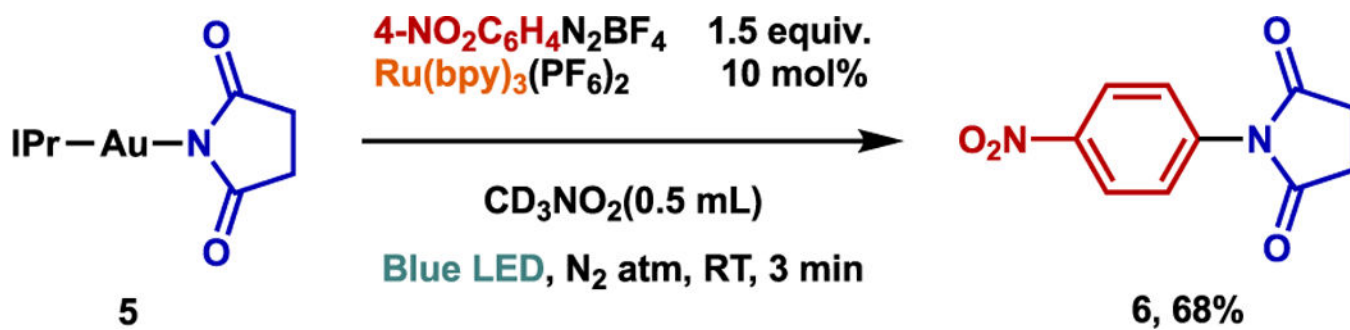
Scheme 4. Photoredox-Initiated Gold-Mediated C(sp 2 )-Succinimide Coupling Reaction a
