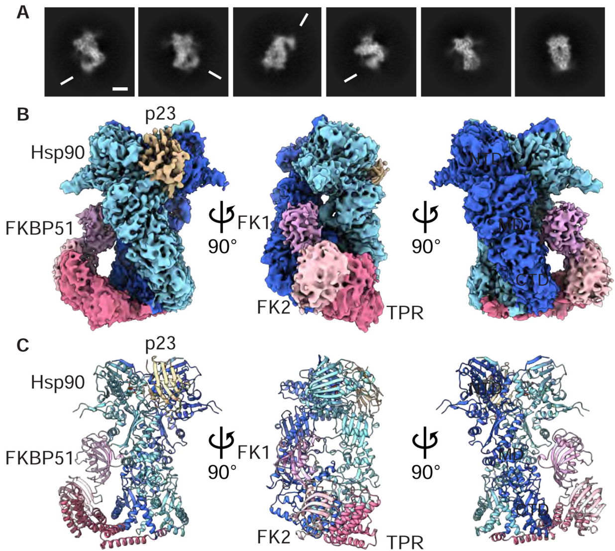
Figure 3. Cryo-EM structure of Hsp90:FKBP51:p23 closed-state complex.
