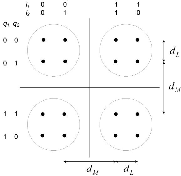
Fig. 1. Hierarchical 16 QAM constellation.
