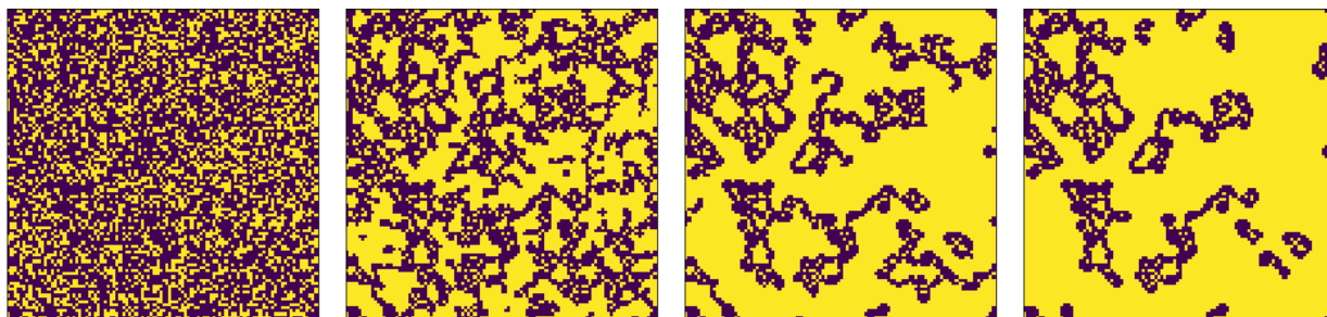
FIGURE 2.1. Bootstrap percolation dynamics with \tau = 4 and initial configuration of 70% probability of populating a cell over a 100 \times 100 lattice with Moore neighborhood and periodic boundary. From left-to-right frames 1, 4, 16 and 64 are presented. Notice that distinct clumps of cells appear to form by iteration 64. The these clumps correspond to cells that are still in 0 state.
