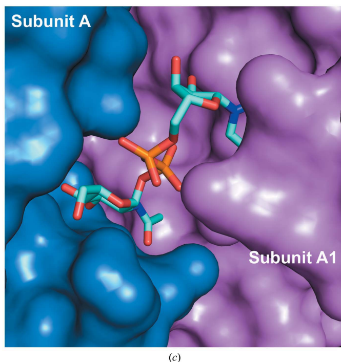
Figure 7 Binding of UDP-GlcNAc at the interface between two monomers within the active trimer. (a) Simulated-annealed OMIT map contoured at 2.5\sigma showing the unbiased positive F_o - F_c electron density around the UDP-GlcNAc substrate. Side chains are omitted for clarity. (b) Amino-acid residues Arg197 and Asn191 from subunit A1 (magenta) of BfLpxA interact with the uracil and diphosphate of UDP-GlcNAc. Amino-acid residues Lys70, His118, Leu69 and Gln154 from subunit A (blue) of BfLpxA interact with the \alpha -phosphate and GlcNAc of UDP-GlcNAc. Also shown are ordered solvent molecules (red spheres) that interact with UDP-GlcNAc, and the acetate ion (ACT). (c) Surface rendering at the interface with UDP-GlcNAc positioned between subunit A and the threefold-related partner subunit A1 of the BfLptA trimer.
