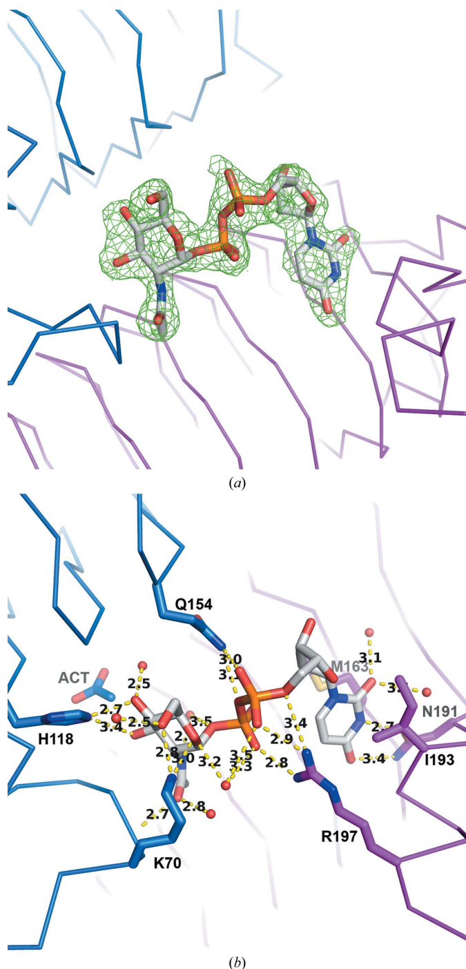
Figure 7 Binding of UDP-GlcNAc at the interface between two monomers within the active trimer. (a) Simulated-annealed OMIT map contoured at 2.5\sigma showing the unbiased positive F_o - F_c electron density around the UDP-GlcNAc substrate. Side chains are omitted for clarity. (b) Amino-acid residues Arg197 and Asn191 from subunit A1 (magenta) of BfLpxA interact with the uracil and diphosphate of UDP-GlcNAc. Amino-acid residues Lys70, His118, Leu69 and Gln154 from subunit A (blue) of BfLpxA interact with the \alpha -phosphate and GlcNAc of UDP-GlcNAc. Also shown are ordered solvent molecules (red spheres) that interact with UDP-GlcNAc, and the acetate ion (ACT). (c) Surface rendering at the interface with UDP-GlcNAc positioned between subunit A and the threefold-related partner subunit A1 of the BfLptA trimer.
