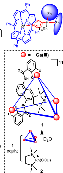
size-selective allylic alcohol isomerization
