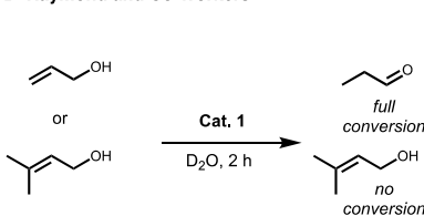
size-selective allylic alcohol isomerization
