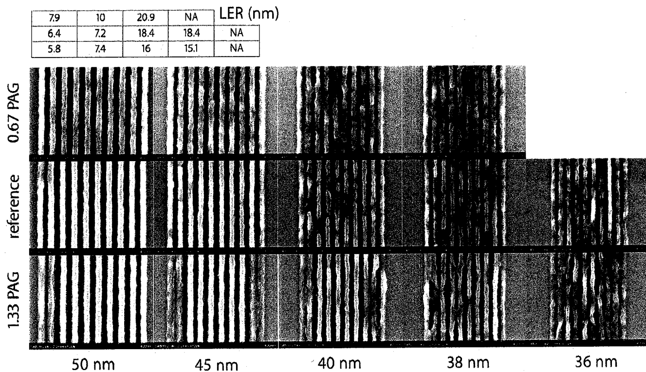
FIG. 2: Photo-acid generator (PAG) study. Through-pitch SEM images of bright field 1:1 lines printed in EH27 resist. Relative PAG weight percents are indicated to the left of each row. Half-pitch coded feature sizes are indicated at the bottom of each column. LER information for each SEM image is indicated in the table.
