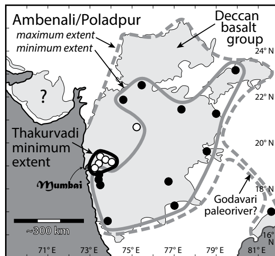
Figure 2. Map of the minimum (mapped) and maximum (inferred) areal extent of the Ambenali and/or Poladpur Formations. Solid circles indicate field locations (Vanderkluysen et al., 2011) in which Ambenali and/or Poladpur have been found; open circles are locations where these formations have not been found. The limited mapped occurrences of thick Thakurvadi Formation are enclosed by thick black line. Gray stippled area gives the areal extent of the Deccan Flood Basalt Group.
