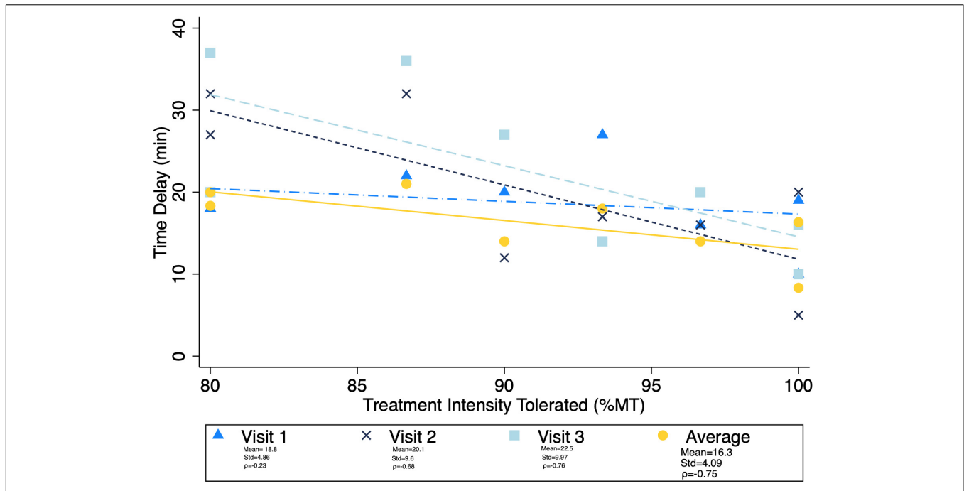
FIGURE 7 | Correlation between average maximum treatment intensity tolerated (noted as a percent of resting motor threshold) and time delay from exposure to TMS. Mean time delay, standard deviation of the delay, and spearman correlation coefficient between treatment intensity and time delay noted for each visit. Pearson correlation was notably lowest at visit 1, and \rho > = 0.7 for all other visits and average delay.
