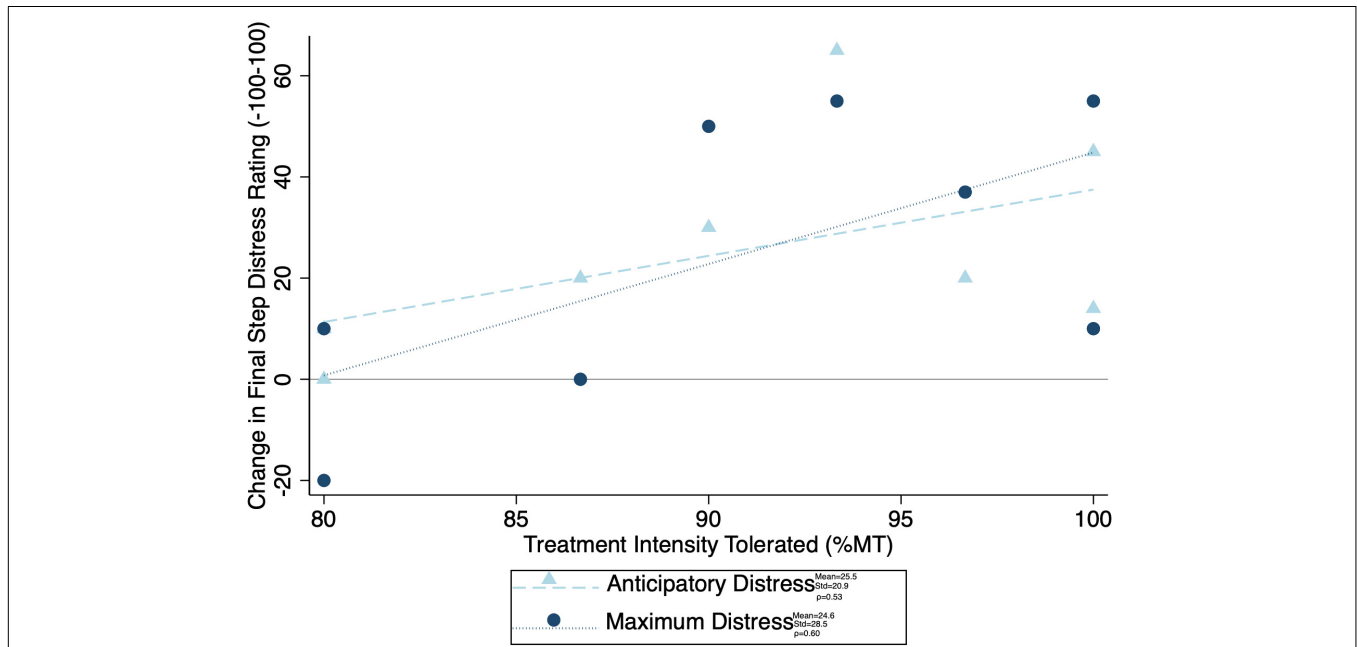
FIGURE 8 | Correlation between maximum treatment intensity tolerated and final common step distress (both anticipatory and maximum experienced distress shown). Change in distress was calculated as pre minus post, with positive values indicating a decrease in distress with treatment. Mean change in distress, standard of deviation of the change in distress, and spearman correlation coefficient ( \rho ) for both anticipatory and maximum distress shown.
