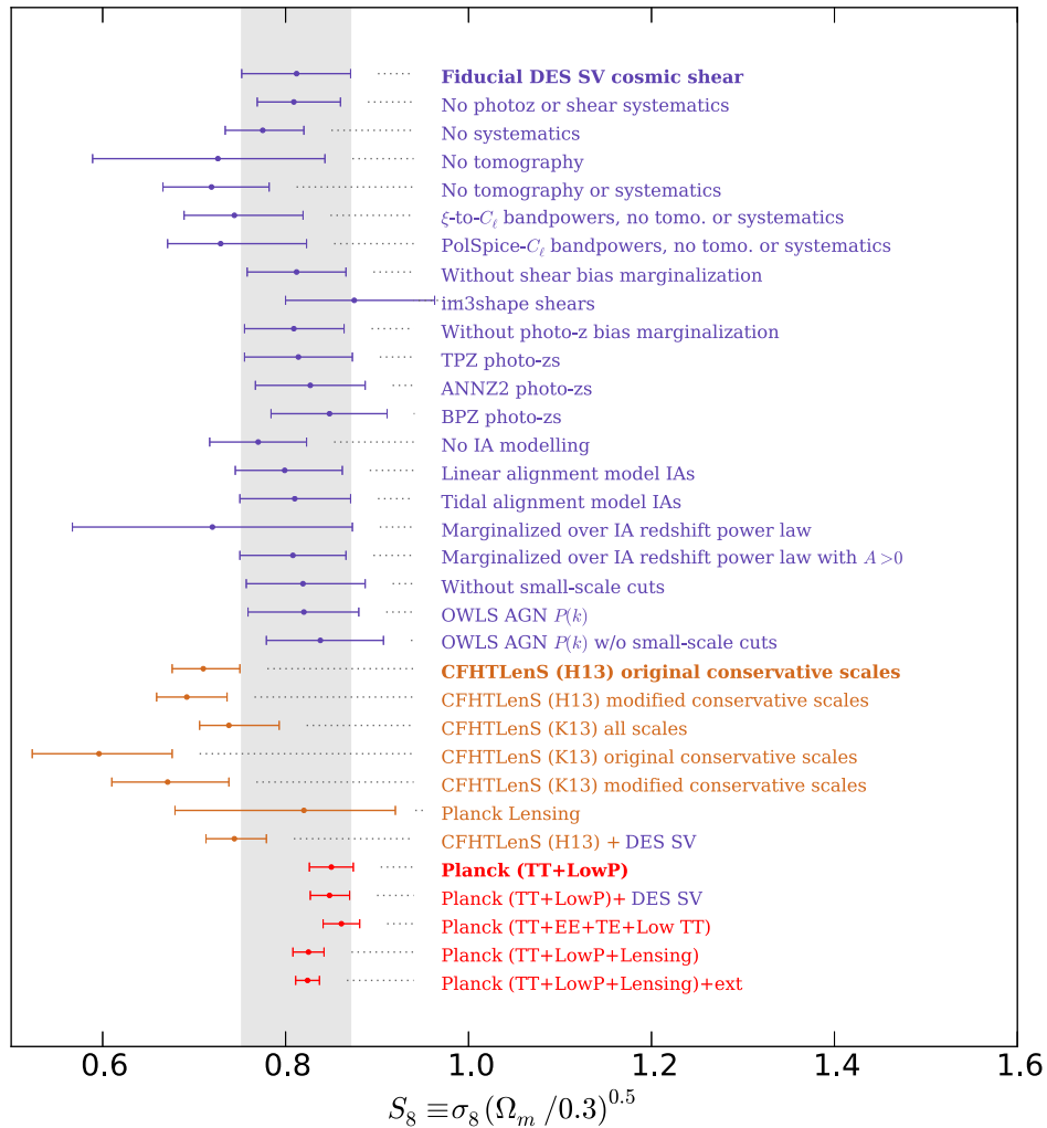
FIG. 3. Graphical illustration of the 68% confidence limits on S_8 \equiv \sigma_8 (\Omega_m / 0.3)^{0.5} values given in Table I, showing the robustness of our results (purple) and comparing with the CFHTLenS and Planck lensing results (orange) and Planck (red). The grey vertical band aligns with the fiducial constraints at the top of the plot. Note that Planck lensing in particular, and other non-DES lensing measurements optimally constrain a different quantity than shown above e.g. see the second and third columns of Table I.
