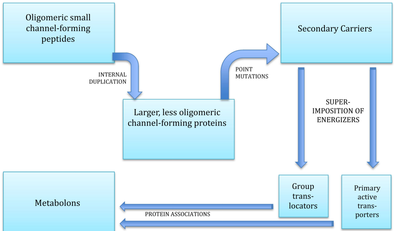
Figure 6. Schematic depiction of the proposed pathway for the evolution of transport proteins including different types of channel-forming proteins and secondary carriers. We further propose that primary active transport carriers and group translocators arose by the superimposition of energy coupling enzymes such as ATPases. Finally, the integration of these systems into metabolic pathways resulted in the physical construction of complex but coordinated metabolons.
