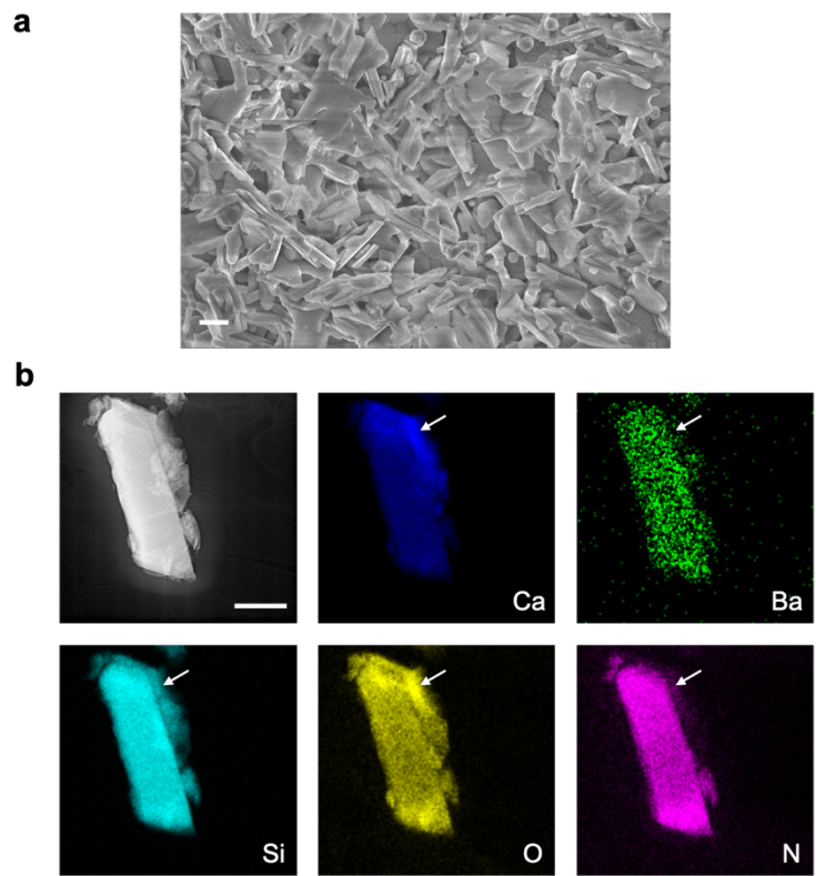
Figure 7. (a) Cross-sectional SEM image of the as-synthesized CBSON pellet. Scale bar: 2 \mu\text{m} . (b) HAADF image of CBSON particle after re-sintering at 1400 °C for 5 h and corresponding EDS mapping acquired from STEM. Scale bar, 400 nm.
