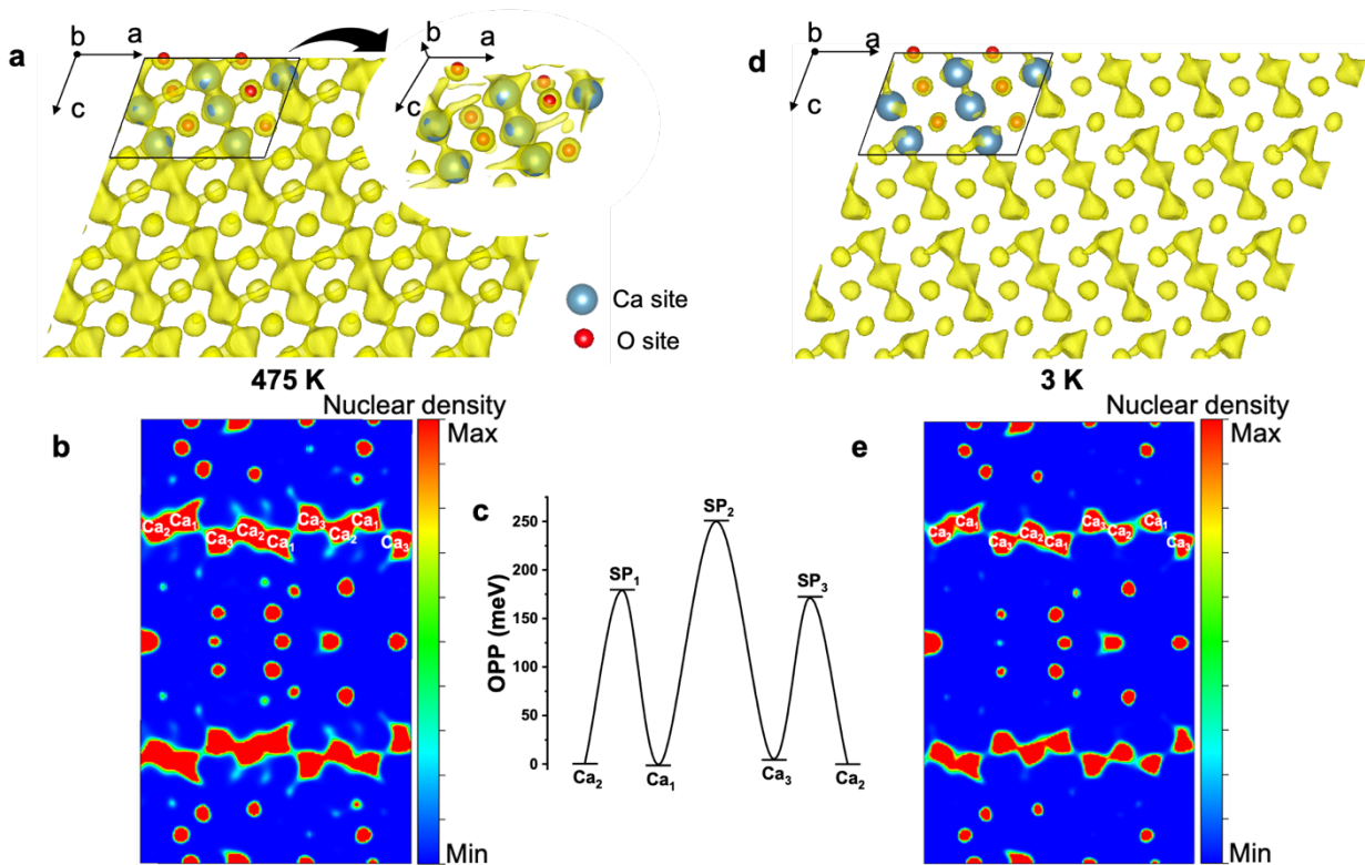
Figure 2. (a) Nuclear density iso-surface plot obtained by a MEM analysis on the NPD data at 475 K shown in the Ca layer down the [010] direction (surface threshold, 0.03 \text{ fm}/\text{\AA}^3 ). In the unit cell, Ca and O sites are shown as blue and red balls, respectively. The inset presents a slightly tilted iso-surface view of the Ca layer. (b) Nuclear density map at 475 K sliced in the (232.11, 1, -110.309) plane with a distance from the origin of 2.47616 \text{ \AA} . (c) Effective one-particle potential profile along the 1D diffusion path, which is calculated from the nuclear density map at 475 K by assuming validity of Boltzmann statistics. (d) Nuclear density iso-surface plot at 3 K in Ca layer down the [010] direction (surface threshold, 0.03 \text{ fm}/\text{\AA}^3 ). (e) Nuclear density map at 3 K sliced in the (232.11, 1 -110.309) plane with a distance from the origin of 2.47616 \text{ \AA} . The scale is the same as in (b).
