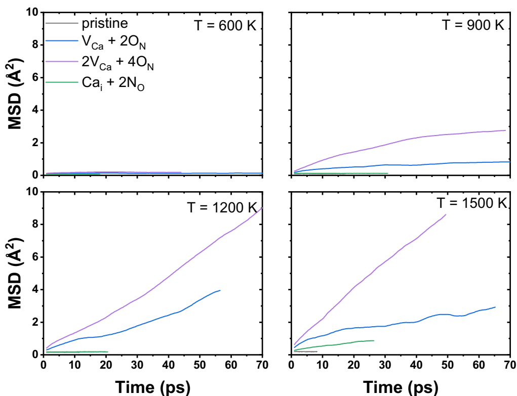
Figure 4. Mean square displacement (MSD) of Ca ion during AIMD simulation at 600 K, 900 K, 1200 K, and 1500 K. The pristine CBSON supercell and supercells with additional 1/12 V_{Ca} , 1/6 V_{Ca} , and 1/12 Ca_i are shown as grey, blue, purple, and green lines, respectively. Note that configurations exhibiting effectively zero Ca mobility were cut short to reduce computational cost.
