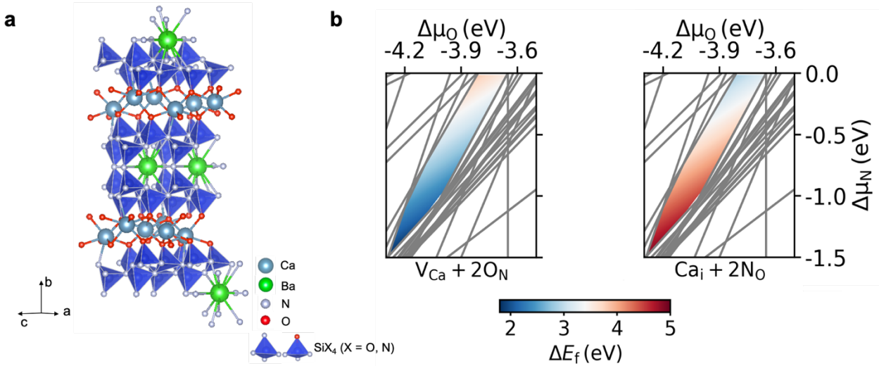
Figure 3. (a) The lowest energy ordered CBSON structure in a 1 \times 1 \times 2 supercell from DFT calculation. (b) Formation energies of Ca vacancies (left) and Ca (right) interstitials in CBSON. \Delta\mu_i is the chemical potential of species i relative to its elemental state, and values close to 0 indicate an i -rich atmosphere. Each grey line represents a stable competing compound in the Ca–Ba–Si–O–N chemical space. The colored region corresponds to the range of chemical potentials where CBSON is stable. The defect concentrations are 1/12 V_{\text{Ca}} , 1/24 \text{O}_{\text{N}} in left and 1/12 \text{Ca}_i , 1/12 \text{N}_o in right. The complete chemical potential triangle is shown in Figure S6.
