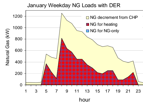
Figure 36: Hospital January Natural Gas Load Provision with CHP
