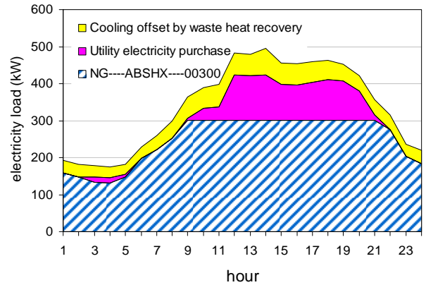
July Weekday Electric Loads with DER
