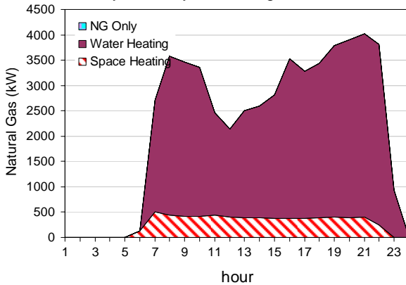
Figure 59: Sports Facility January Natural Gas Loads
