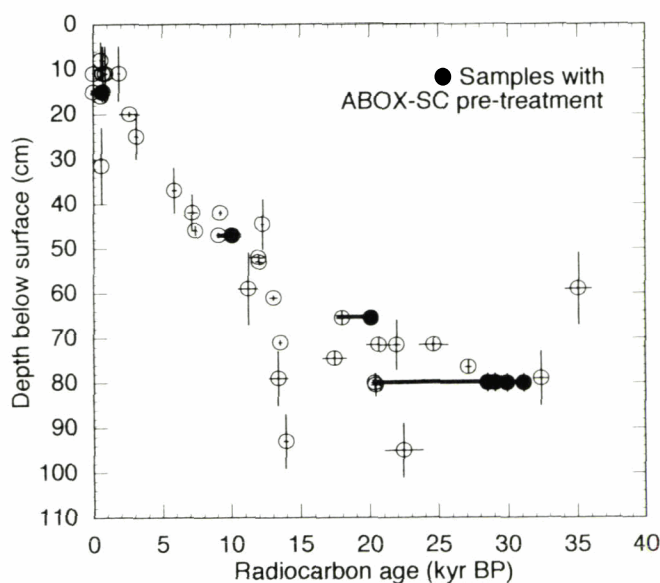
Figure 1 Age-depth curve for radiocarbon determinations from Puritjarra rock shelter showing the impact of ABOX-SC pre-treatment on apparent radiocarbon age for selected charcoal samples.
