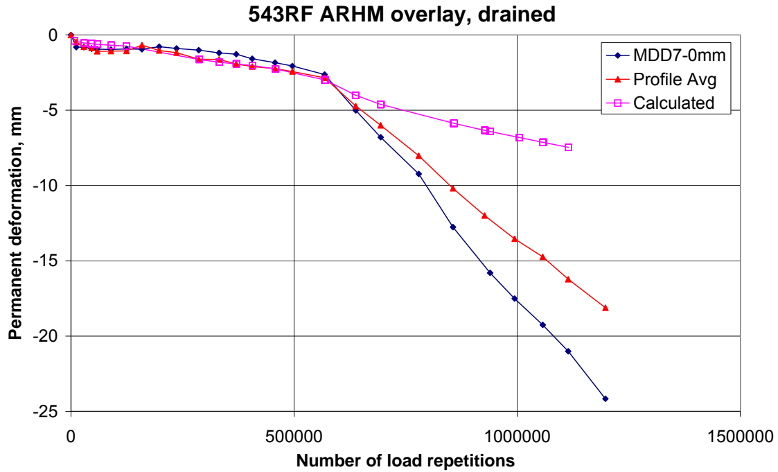
Figure 190. Section 543RF permanent deformation at pavement surface.
