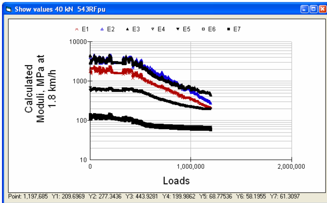
Figure 191. Section 543RF calculated layer moduli, at 40 kN and actual temperatures.
