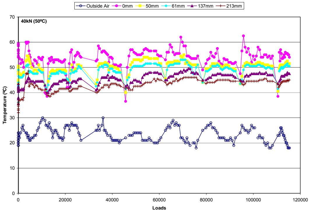
Figure 152. Section 508RF temperatures during testing.
