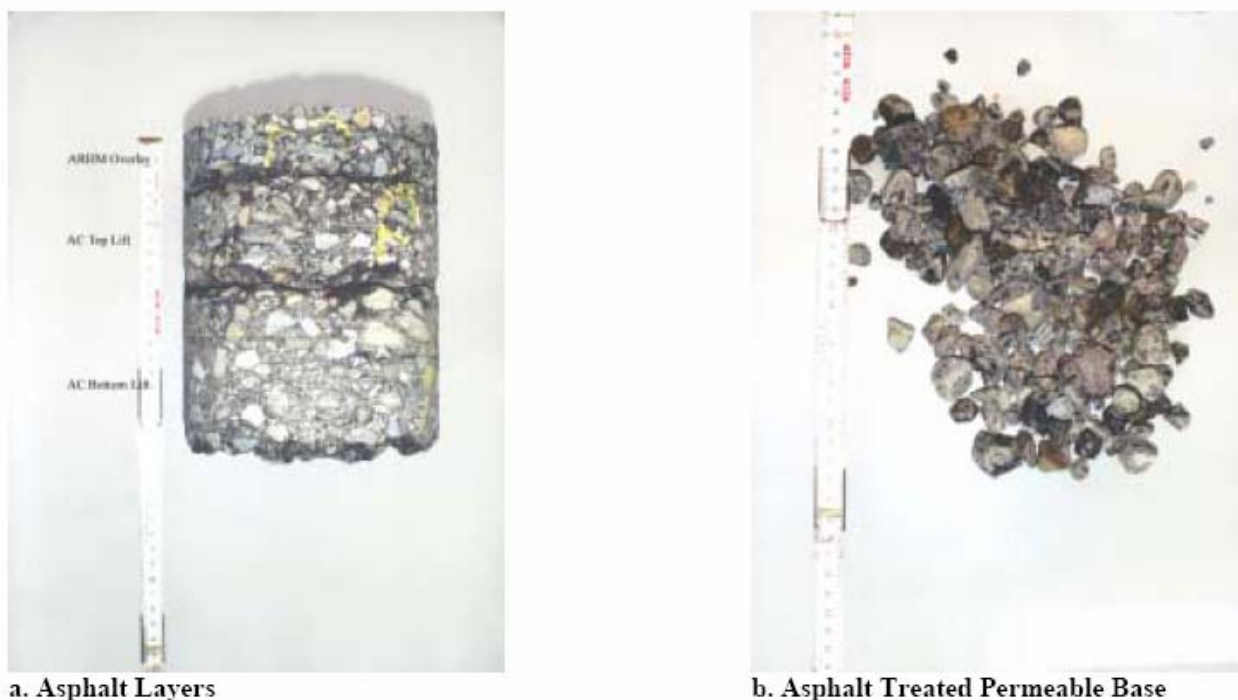
Figure 174. Cores from trafficked area of Section 543RF after HVS loading show stripping and disintegration of ATPB, as well as signs of moisture damage between the the three lifts of asphalt concrete (Bejarano et al. 2003).
