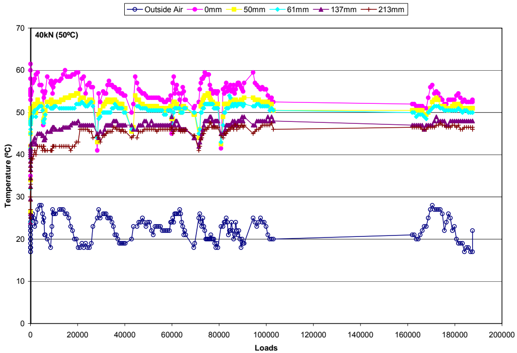
Figure 156. Section 509RF temperatures during testing.
