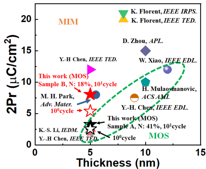
Figure 7. Benchmark of 2Pr for \text{HfO}_2 -based ferroelectric capacitors with different structures and film thicknesses [12–20].
