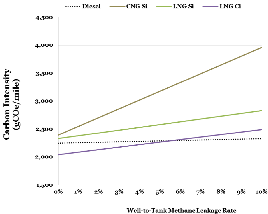
Figure 30. 100-year carbon intensity (gCO 2 e/mile) of C8 diesel and natural gas under different leakages rate. Dashed line represents diesel, brown line is CNG on a Si
