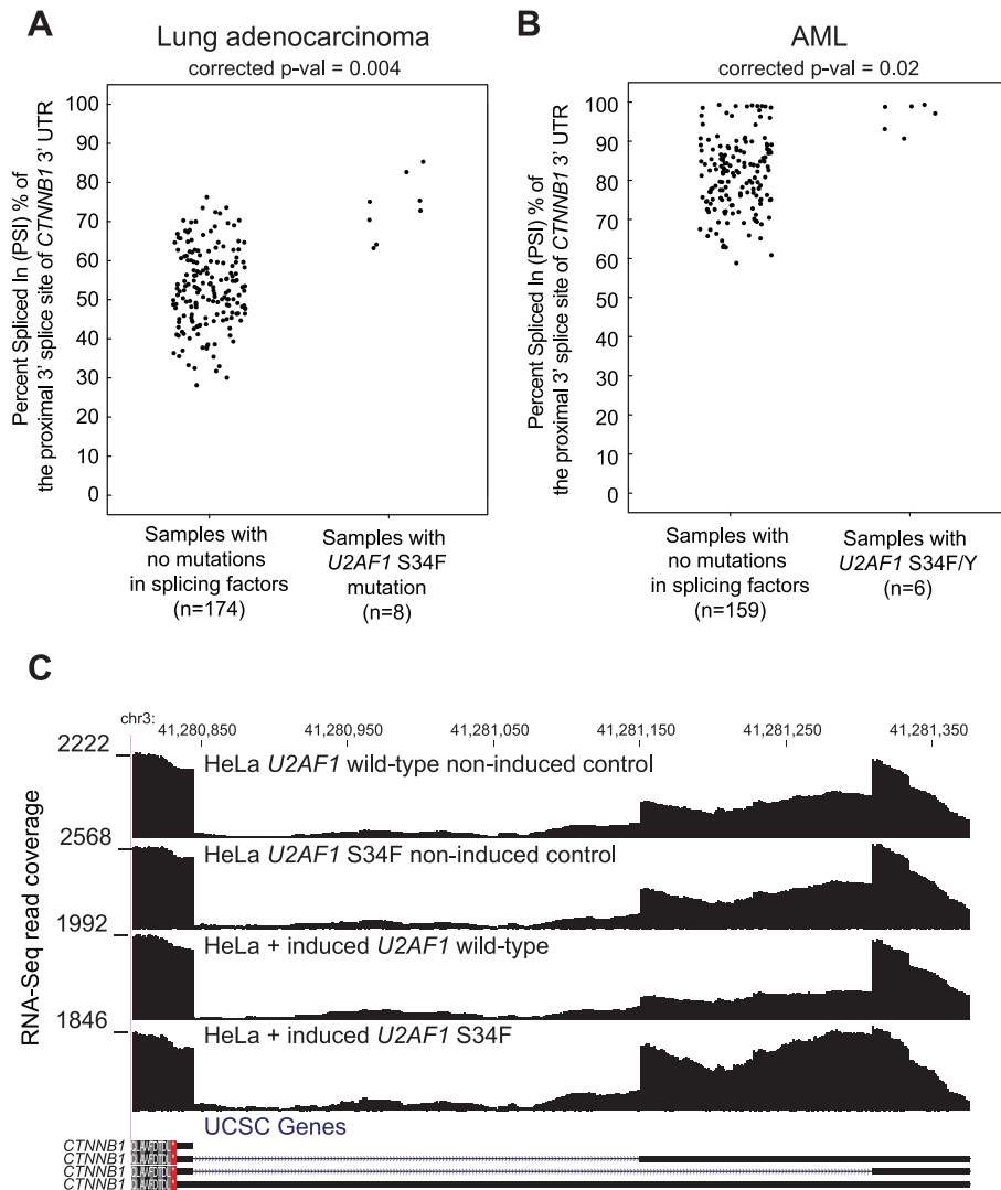
Figure 4. CTNNB1 3' UTR splicing associated with U2AF1 S34F/Y mutation in lung adenocarcinoma and AML. “Percent spliced in” (PSI) values of the proximal 3' splice site of the CTNNB1 3' UTR splice event in (A) lung adenocarcinoma and (B) AML. (C) RNA-Seq read coverage of the 3' UTR event in HeLa cells with two U2AF1 non-induced controls, induction of U2AF1 wild-type, and induction of U2AF1 S34F. doi:10.1371/journal.pone.0087361.g004
