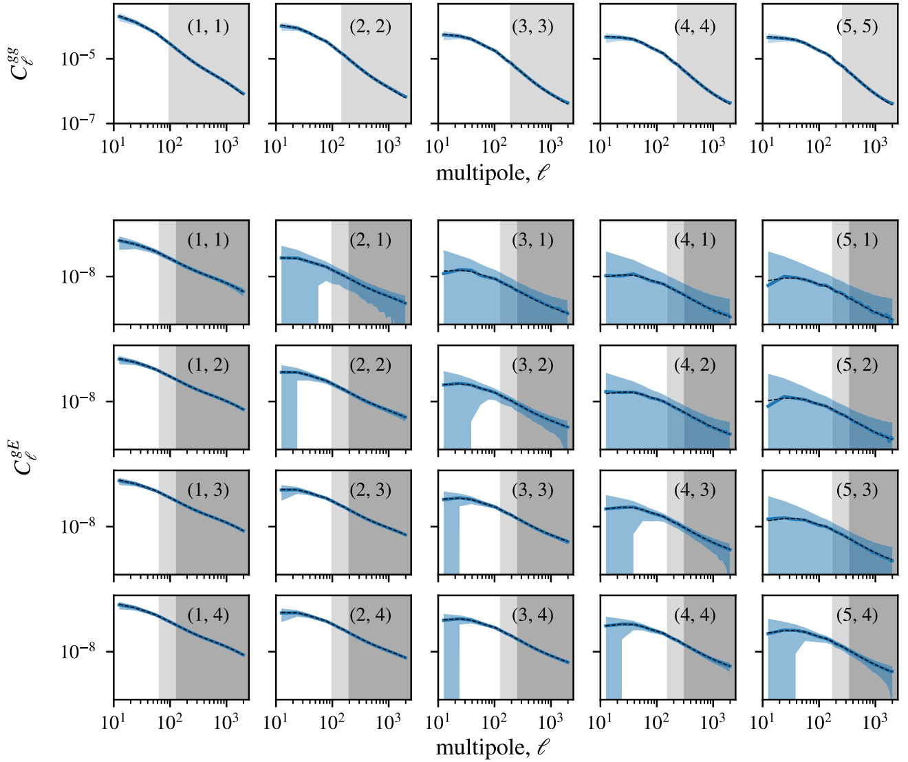
Figure B1. The angular power spectrum measurements for the set of 1800 log-normal realizations. Top panel: average of the galaxy clustering measurements C_{\ell}^{\text{gg}} (solid line) and their standard deviation (blue, shaded area). The grey shaded area represents the scale cut based on the minimum physical scale R_{\text{min}}^{\text{gl}} = 8 \text{ Mpc } h^{-1} . Bottom panel: average of the GGL measurements C_{\ell}^{\text{gE}} (solid line) and their standard deviation (blue, shaded area). The grey shaded area represents the scale cuts based on the minimum physical scale R_{\text{min}}^{\text{gl}} = 6 \text{ Mpc } h^{-1} (light grey) and R_{\text{min}}^{\text{gl}} = 12 \text{ Mpc } h^{-1} (dark grey). The indexes (z_i, z_j) in each subplot indicate the redshift bin combination. For GGL, z_i and z_j refer to the bin of the lens and source, respectively. The black dashed curves show the input power spectra used to generate the log-normal realizations.
