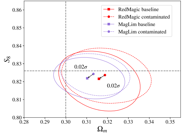
Figure 5. 2D posterior of S_8 and \Omega_m for REDMAGiC and MAGLIM baseline and contaminated data vectors under the extended (8, 6) Mpc h^{-1} scale cut, both analysed with linear bias and HALOFIT model. The ellipses represent 0.3\sigma_{2D} contours around their best-fitting values marked in the centre. The arrows and numbers show the distance between the best fit of baseline and contaminated chains.
