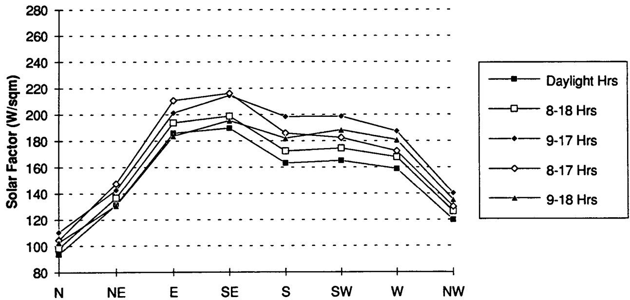
Figure 3-7a. Bangkok Solar Factor by Averaging Hours
