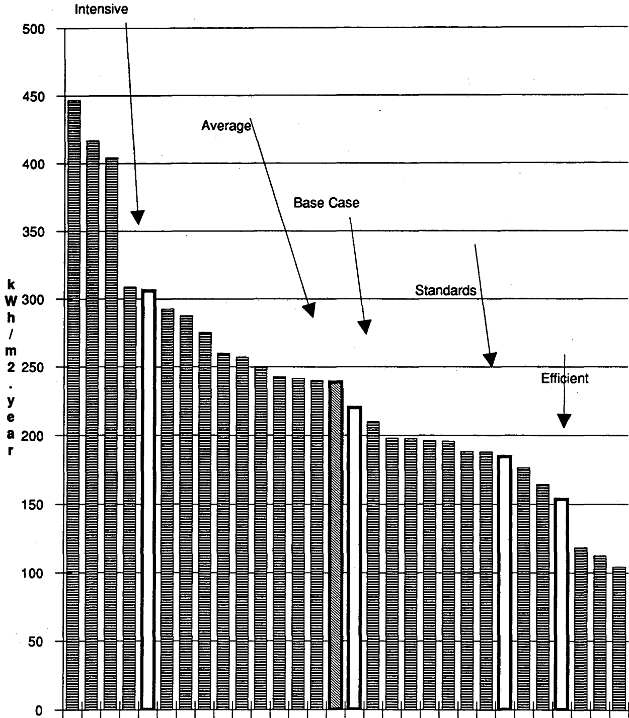
Figure 4-1. Comparison of Large Office Illustrative Cases with Office Building Survey Sample in Philippines
