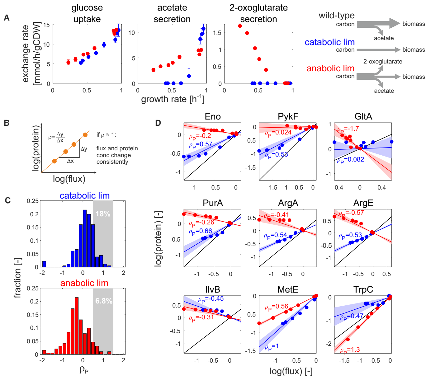
Figure 2. Regulation analysis of flux–protein relationship in nutrient limitations.
