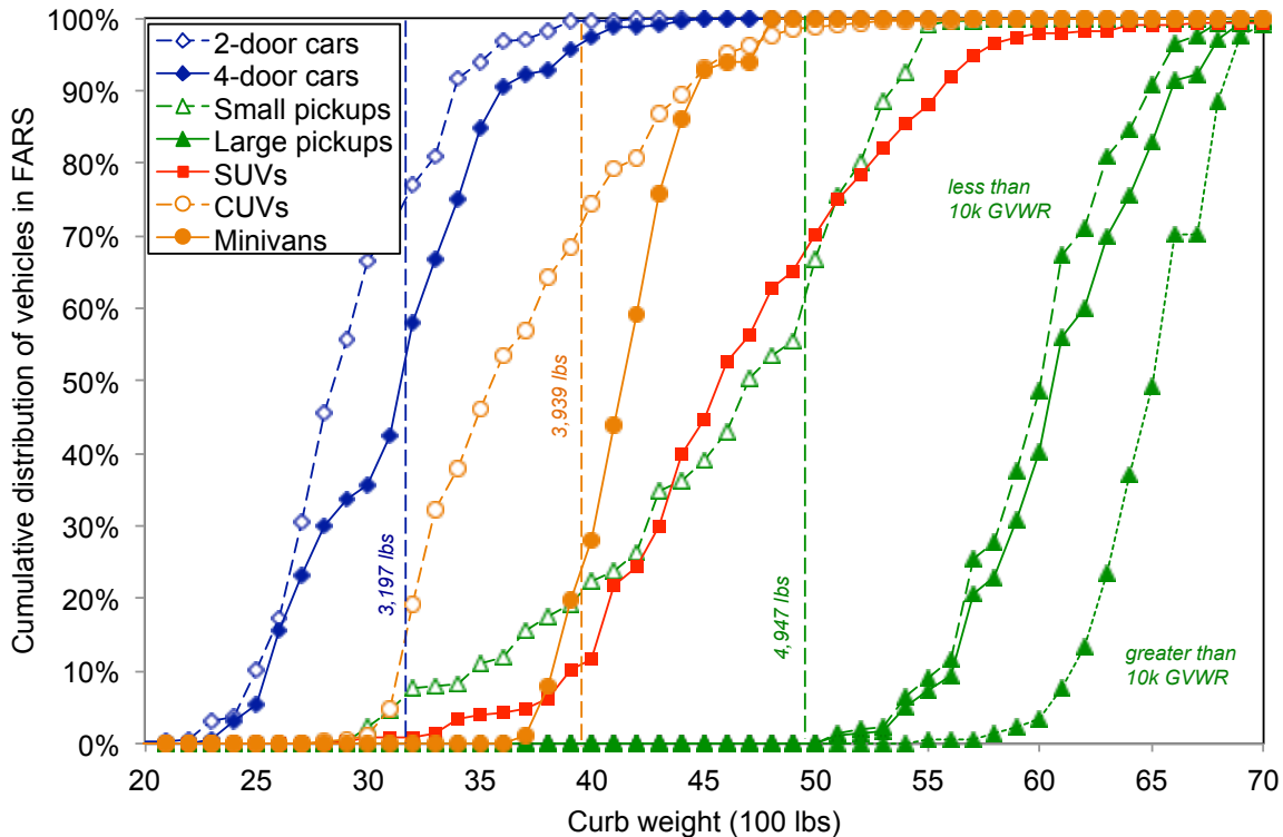
Figure 5.16. Cumulative distribution of vehicle curb weight, by vehicle type, including large pickups under and over 10,000 GVWR
