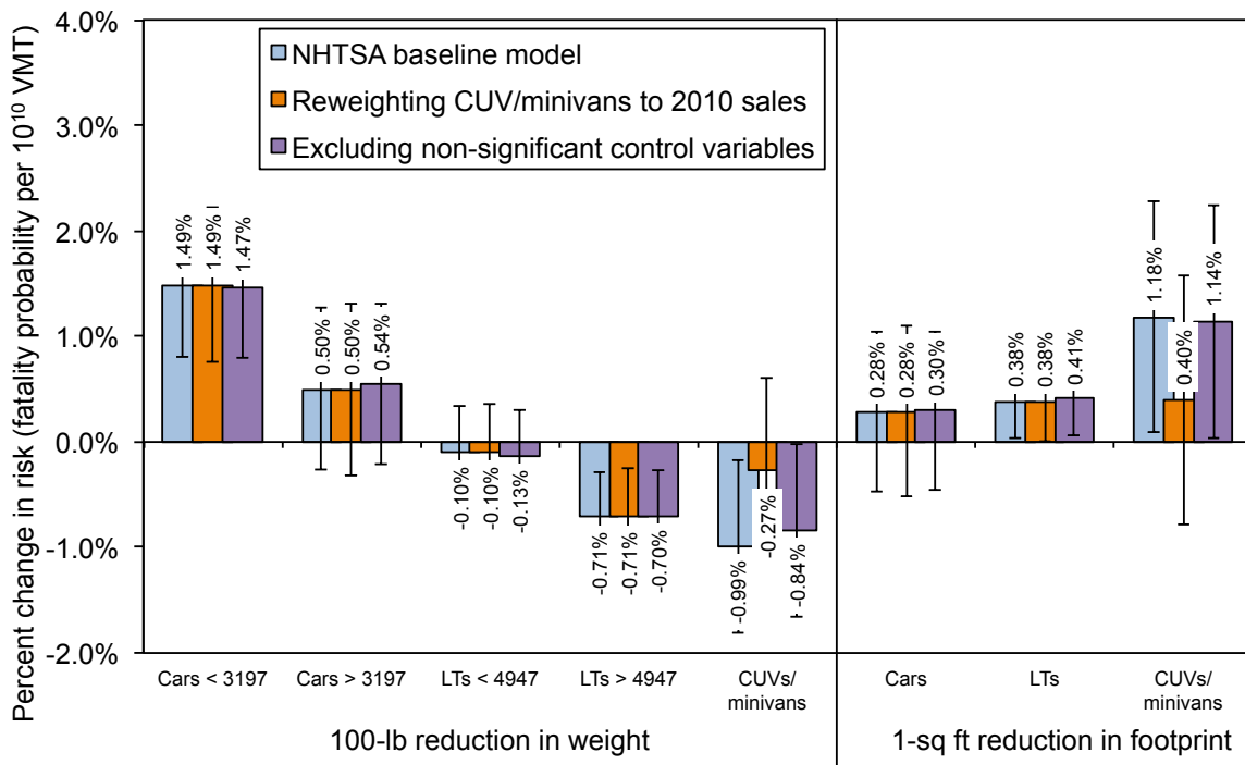
Figure 5.14. Estimated effect of mass and footprint reduction on US fatality risk per VMT, after reweighting CUV/minivan fatalities to 2010 sales and excluding non-significant control variables, by vehicle type
