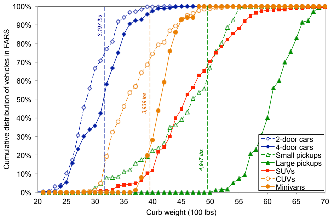
Figure 5.15. Cumulative distribution of vehicle curb weight, by vehicle type
