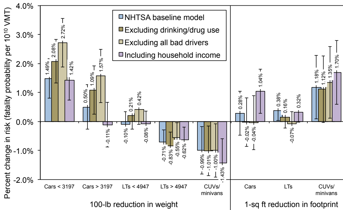
Figure 5.12. Estimated effect of mass or footprint reduction on US fatalities per VMT, after excluding case vehicles whose driver was drinking, using drugs or exhibited bad driving behavior, or controlling for median household income, by vehicle type
