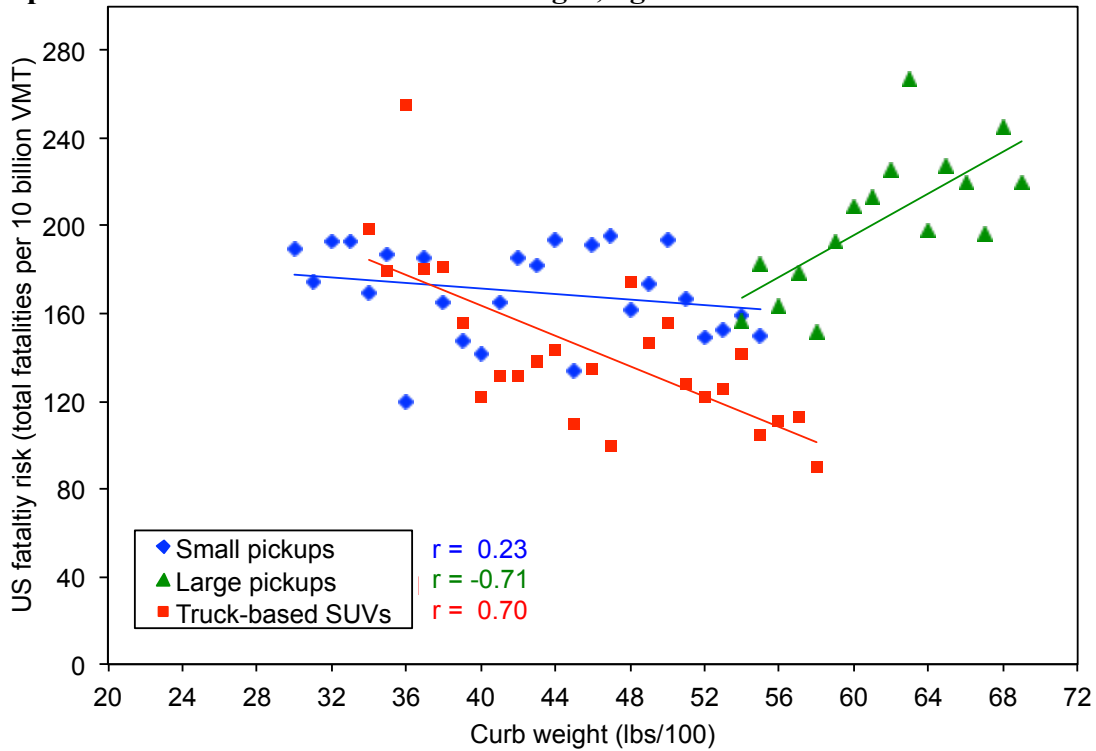
Figure 4.3. Relationship between US societal fatality risk and curb weight, with vehicles grouped into 100-lb increments of curb weight, light trucks
