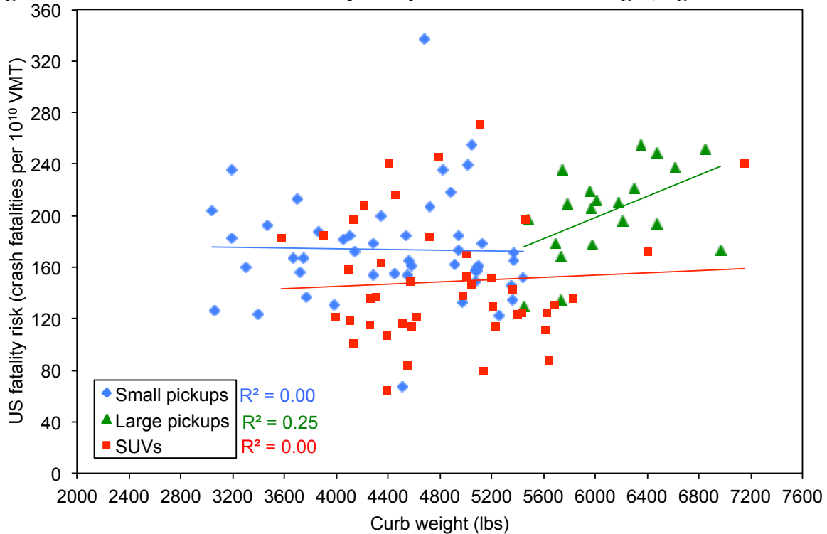
Figure 4.10. Actual US societal fatality risk per VMT vs. curb weight, light truck models
