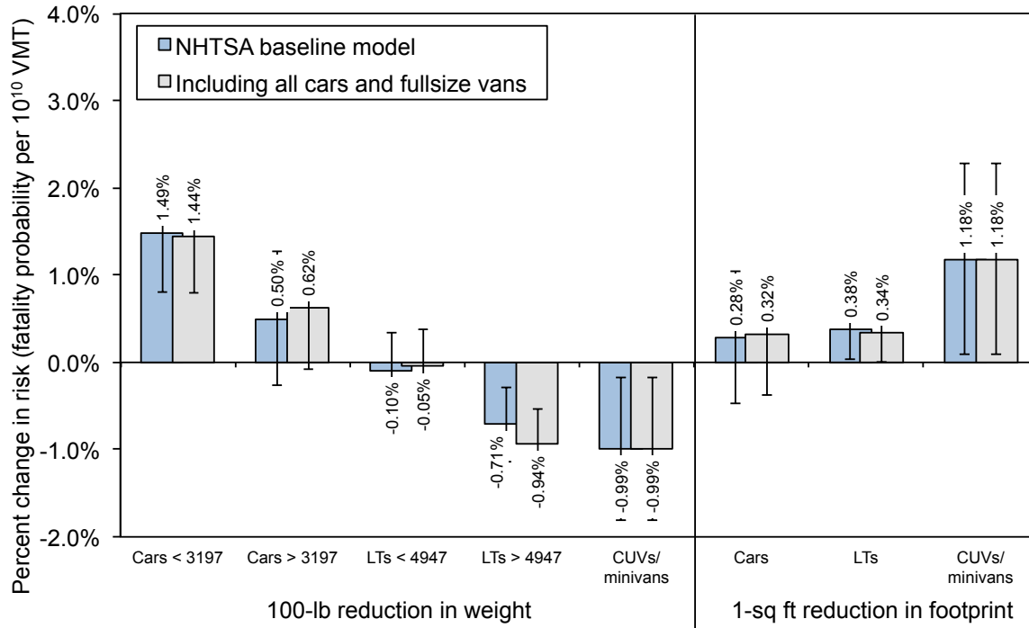
Figure 5.13. Estimated effect of mass and footprint reduction on US fatality risk per VMT, after including sports, police, and all-wheel drive cars, and fullsize passenger and cargo vans, by vehicle type
