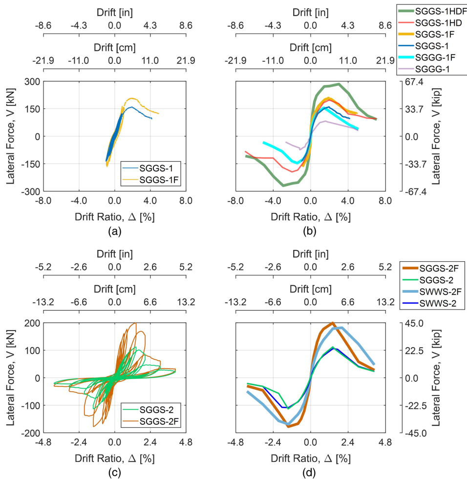
Fig. 3. Effect of finish application: (a) force-displacement response for Type I specimens; (b) backbone curve comparison for Type I specimens; (c) force-displacement response for Type II specimens; and (d) backbone curve comparison for Type II specimens.
