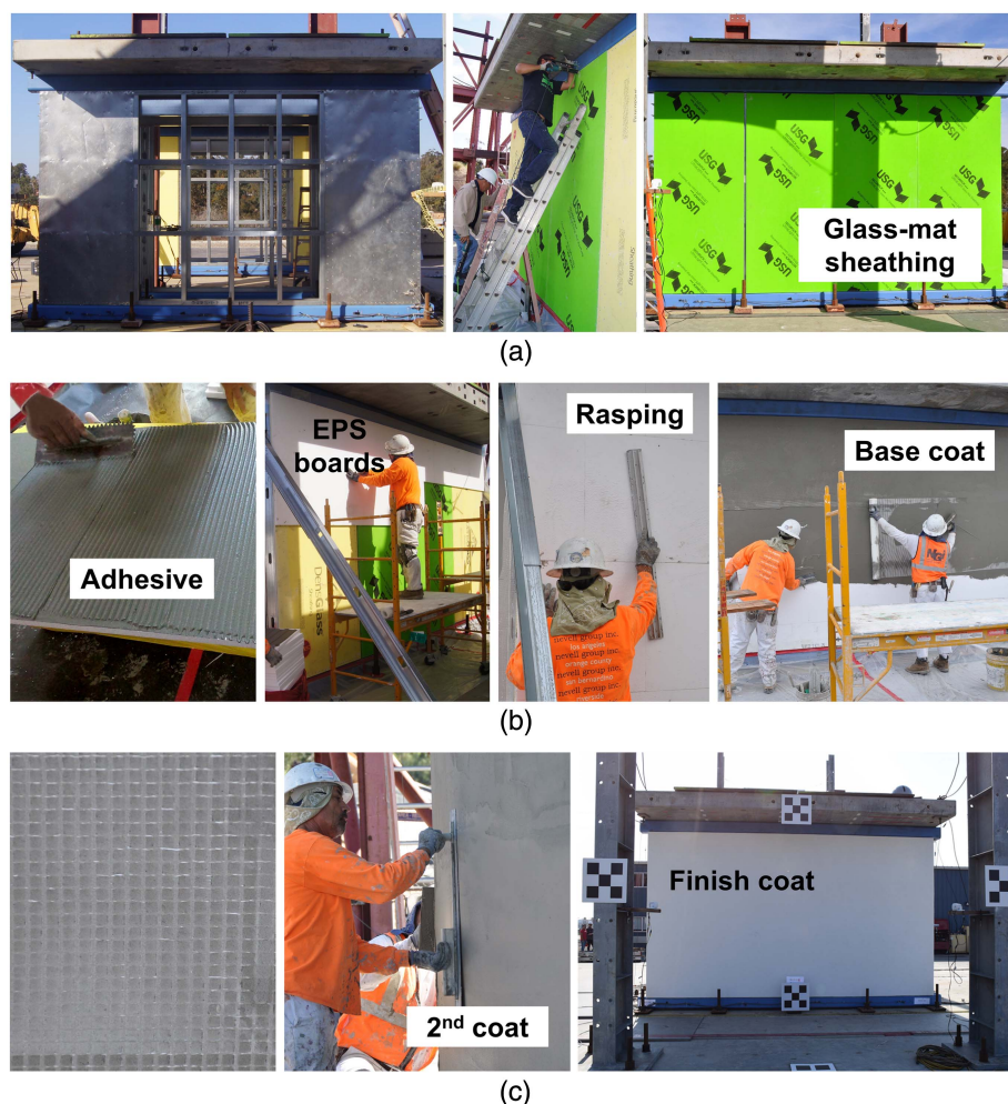
Fig. 2. Steps involved in exterior face finish application: (a) installation of glass-mat sheathing panels; (b) application of EPS foam boards using adhesive onto panel substrate followed by rasing of foam boards and application of base coat; and (c) embedded reinforcing mesh in base coat and application of second layer and finish coat.
