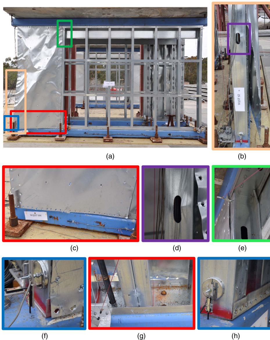
Fig. 13. (a-h) Physical damage to Specimen SGGG-1 following the dynamic testing sequence, \Delta_{\max} = 5.1\% and \Delta_{\text{res}} = 0.26\% .
