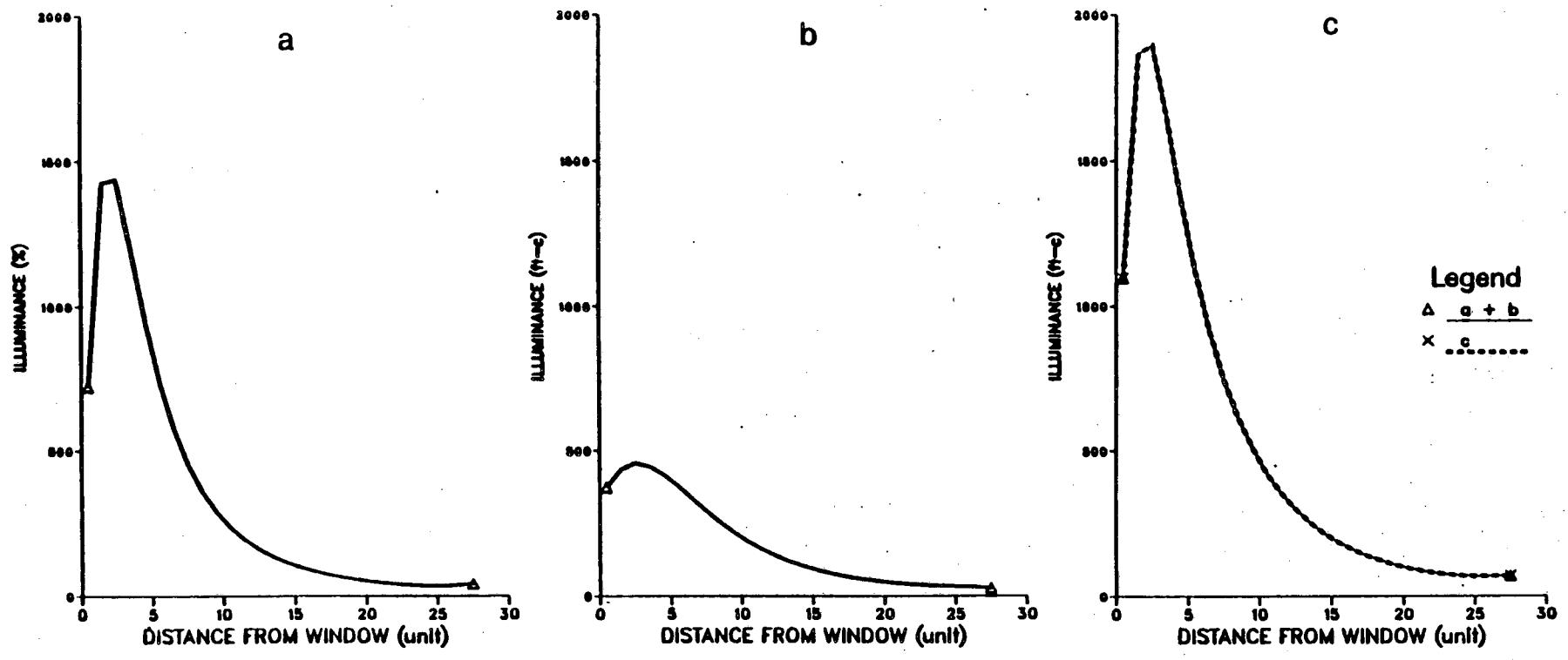
Figure 4. Parts a, b, and c show calculated indoor illuminance levels using the complementary candlepower distributions shown in Figure 3a, b, and c, respectively.
