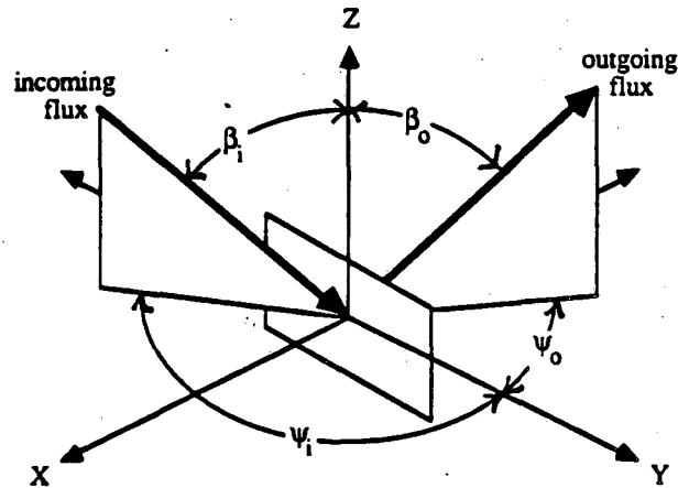
Figure 1. The angles \beta_i, \psi_i and \beta_o, \psi_o , which describe the directions of the incoming and outgoing radiation.
