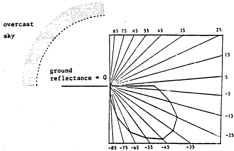
a) Candlepower distribution of clear glass window under overcast sky
