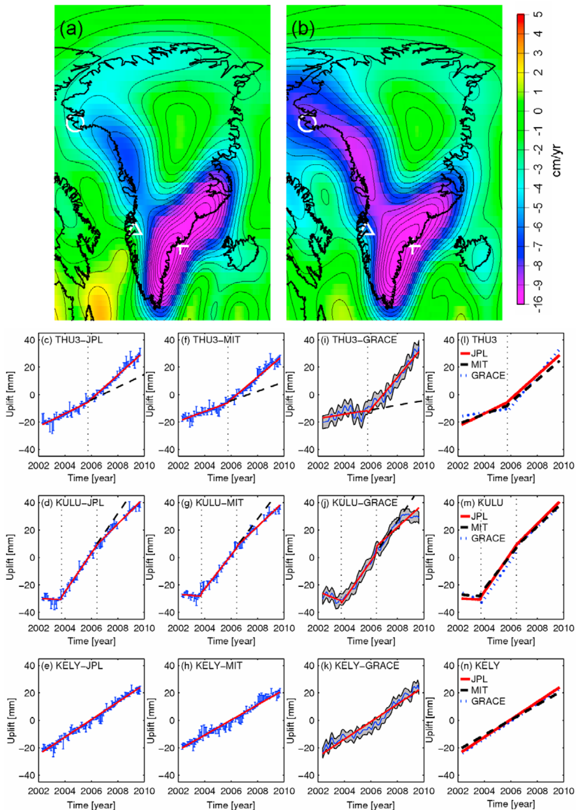
Figure 1. The rate of mass loss, in cm/yr water equivalent thickness, determined from monthly GRACE gravity field solutions. (a) The rate averaged between February 2003 and February 2007. (b) The rate averaged between February 2003 and June 2009. The symbols show the locations of the GPS sites: THU3 (circle), KELY (triangle), KULU (plus sign). 30-day vertical GPS averages obtained using JPL products at (c) THU3, (d) KULU, and (e) KELY. 30-day vertical GPS averages obtained using MIT products at (f) THU3, (g) KULU, and (h) KELY. Predicted uplift using monthly GRACE solutions at (i) THU3, (j) KULU, and (k) KELY. The areas marked with grey (Figures 1i–1k) represent upper and lower bounds due to scaling uncertainty. Best fitting linear terms to the JPL and MIT solutions and the scaled predicted uplift from GRACE at (l) THU3, (m) KULU, and (n) KELY.
