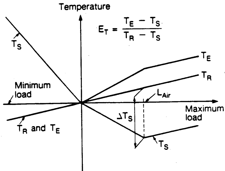
Figure 2. Control strategy of displacement ventilation with constant air flow. E_T = temperature efficiency. L_{AIR} = maximum cooling by air, \Delta T_S = maximum temperature difference between room and supply air, T_E = exhaust temperature, T_S = supply temperature, T_R = room temperature at height 2.6 ft (0.8 m)
