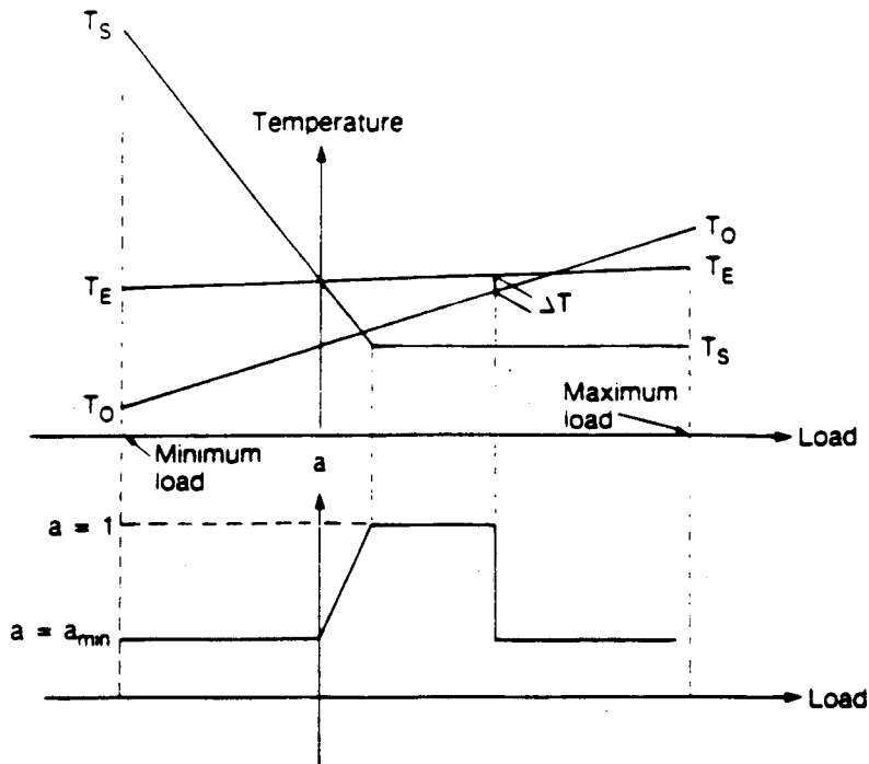
Figure 5. Control strategy of economizer cycle. Outdoor air ratio "a" ( Q_o/Q_s ) depends on the temperatures in the system and preset temperature difference \Delta T between outdoor air and exhaust air. Its minimum value a_{min} depends on minimum outdoor air flow rate. T_E = exhaust temperature, T_S = supply temperature, T_O = outdoor air temperature.
