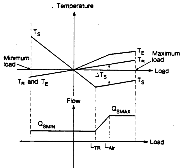
Figure 6. Control strategy of displacement ventilation system with variable air flow and terminal reheat. L_{TR} = the cooling load which still can be met with minimum supply air flow, L_{AIR} = maximum cooling by air, Q_{SMIN} = minimum supply air flow, Q_{SMAX} = maximum supply air flow \Delta T_S = maximum temperature difference between room and supply air, T_E = exhaust temperature, T_S = supply temperature, T_R = room temperature at height 2.6 ft (0.8 m).
