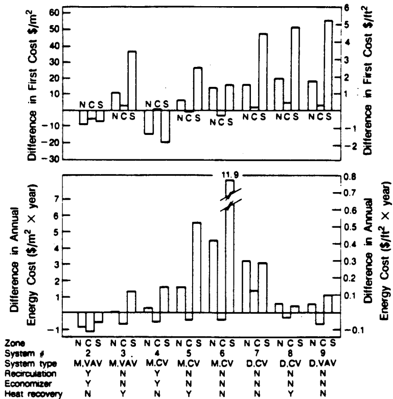
Figure 11. Comparison of first cost and annual energy cost of Systems 2 - 9 to the same costs for System 1 in the Minneapolis climate. The assumed costs of electricity and natural gas are 5.7 cents/kWh and 1.3 cents/kWh, respectively.
