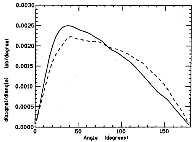
Figure 4. The angles between the two jets (solid) and between the fast jet and the electron. Masses as in Fig. 3.
