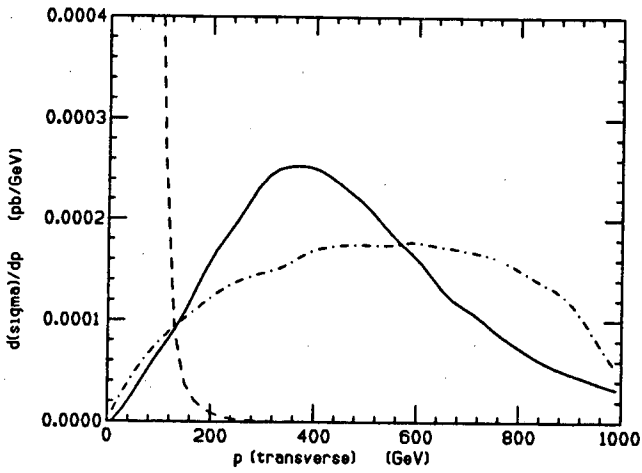
Figure 1. The distributions from \tilde{w}\tilde{g} production of transverse momentum for the fast jet (solid), the slow jet (dashed) and the electron (indistinguishable from solid curve). The dot-dash curve is the missing transverse energy. M(\tilde{w}) = m(\tilde{q}) = 950 GeV and m(\tilde{g}) = 1000 GeV.
