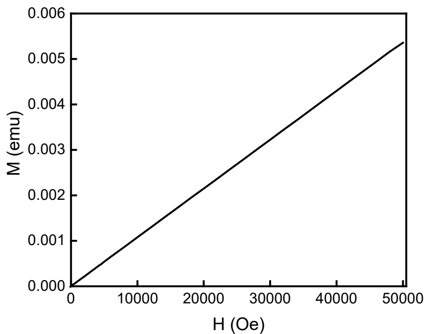
Figure D14. Plot of M versus H at 300 K for (\text{thiofan}^*)\text{YbCl}(\text{THF})_n .
