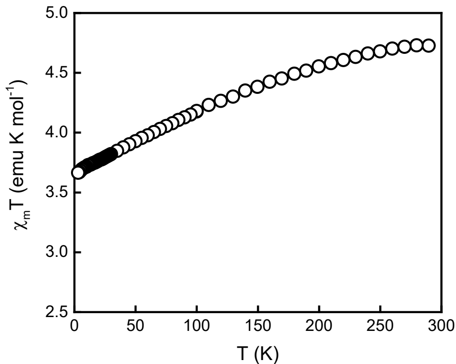
Figure 5.9. Plot of \chi_m T versus T for [(\text{thiolfan})\text{YbCl}]_2 under a 1000 Oe dc field in the temperature range 2-290 K.
