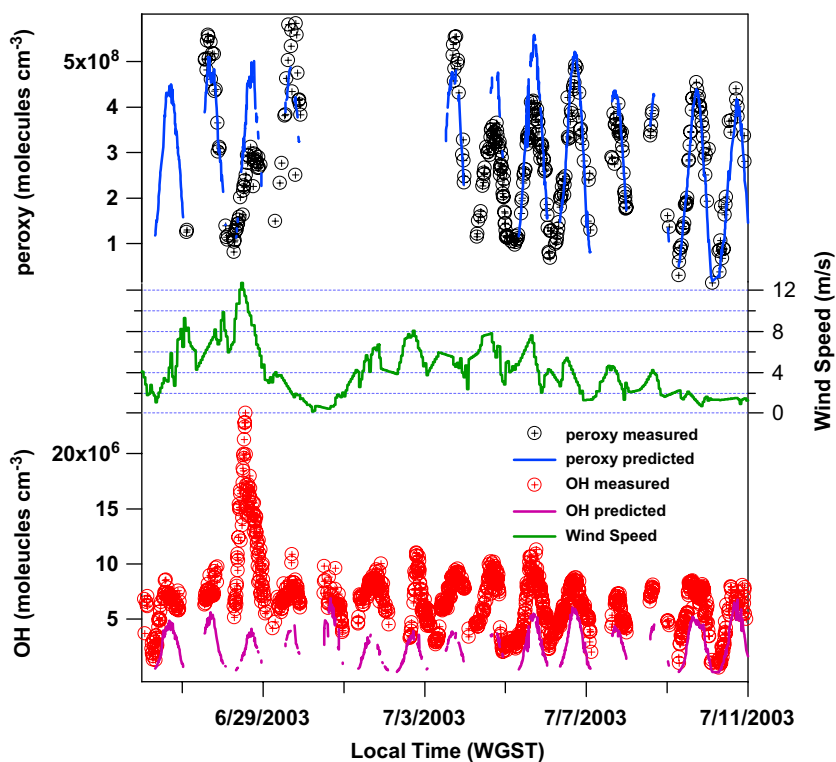
Fig. 5. Time series of hydroxyl and peroxy radical measurements and wind speed. The black circles and the solid blue line represent measured and modeled peroxy concentrations. The red circles and solid purple line represent measured and modeled hydroxyl concentrations. The green line indicates wind speed. Note that the gap in peroxy radical measurement was due to removal of the NO addition. This was done to make sure that a possible NO leak in the sample tube did not lead to high measurements of hydroxyl radicals.
