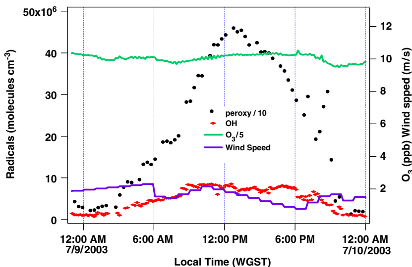
Fig. 10. Measured values for radicals, ozone and wind speed on 9 July. Black dots = peroxy radicals (number density/10), red diamonds = OH (number density), green line = ozone (ppbv/5) and blue Line = wind speed ( \text{m s}^{-1} ).
