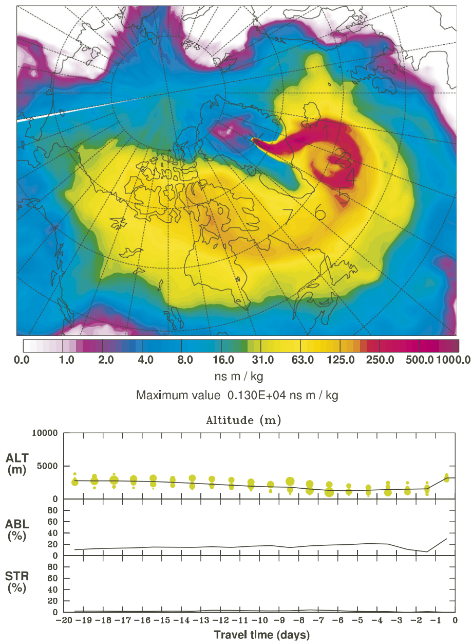
Fig. 13. FLEXPART model 20-day back projection for 28 June. The emission sensitivity integrated over the entire atmosphere (at the top) indicates that there was a strong flow of marine air to Summit from a low pressure system in the North Atlantic. Numbers mark the average position of the air mass at daily intervals back in time and show that the air was already south of Iceland one day previously. A marine boundary layer origin is also suggested by the low average altitude of the tracked particles (lower panel) and the significant percentage of atmospheric boundary layer air (ABL). Plots of the emission sensitivity for the lowest 100 m of the atmosphere (not shown) also reveal high values over the North Atlantic Ocean.
