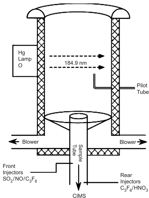
Fig. 2. CIMS inlet configuration. The residence time of the air sample in the inlet is 50 ms.
