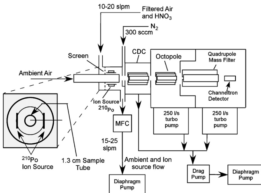
Fig. 1. Schematic of the CIMS used during the Summit 2003 field campaign.
