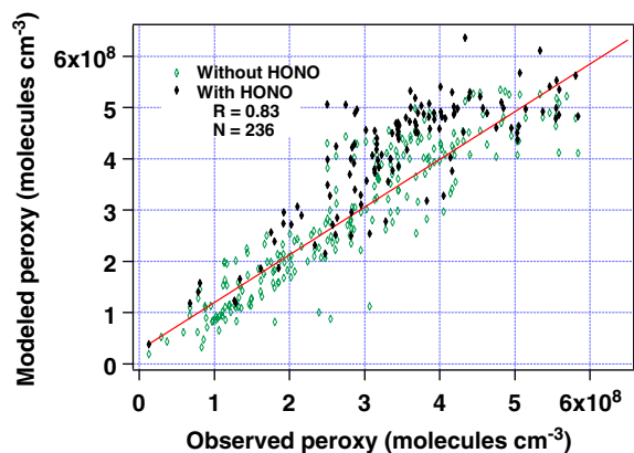
Fig. 6. Scatter plot of predicted versus measured \text{HO}_2 + \text{RO}_2 radicals. Model results without HONO are represented by open green diamonds and results with HONO are indicated by solid black diamonds. The linear regression is fit to model results without HONO.
