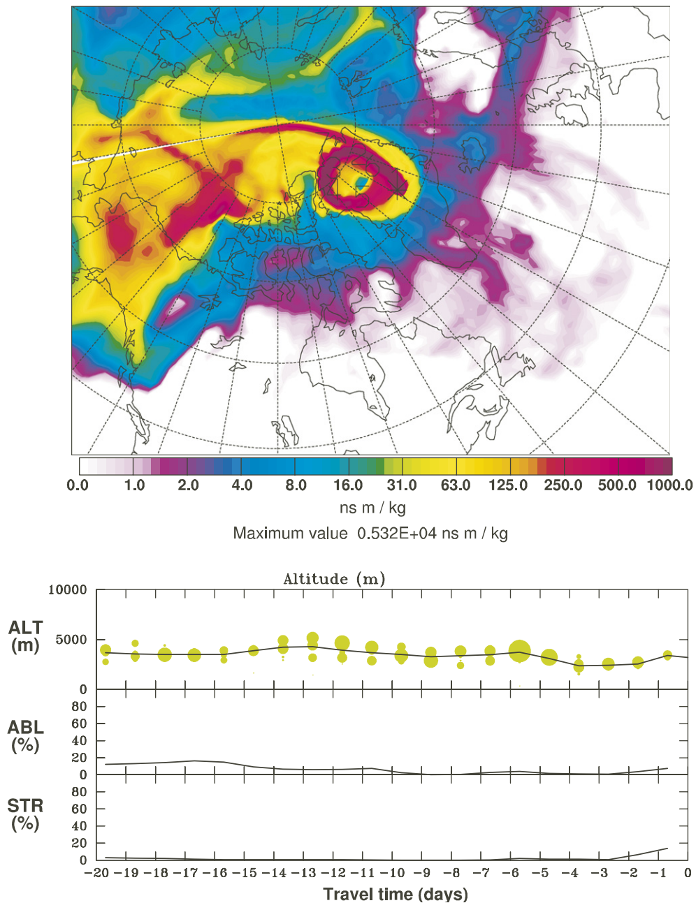
Fig. 11. FLEXPART 20-day model back projection for 9 July. The emission sensitivity integrated over the entire atmospheric column (at the top) indicates that the majority of the air sampled at Summit was from the surrounding Greenland Ice cap. The altitude profile reinforces this conclusion and indicates that the air spent little time in the boundary layer. This was confirmed by low values of the emission sensitivity for the lowest 100 m of the atmosphere (not shown).
