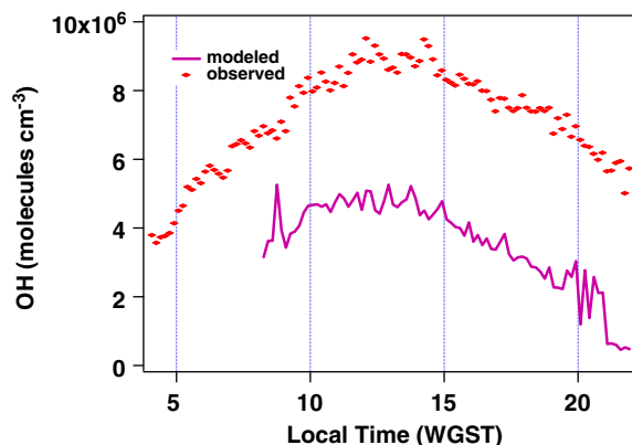
Fig. 9. Composite 24 h measurements and model predictions of OH. Predicted values obtained from NMHC model constrained by \text{H}_2\text{O}_2 , \text{CH}_2\text{O} and HONO.
