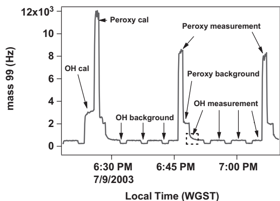
Fig. 4. A typical sequence with measurement, calibration and background periods for hydroxyl and peroxy radicals. The region inside the dashed box is an example of a hydroxyl measurement that is discarded due to lingering NO in the sample tube.
