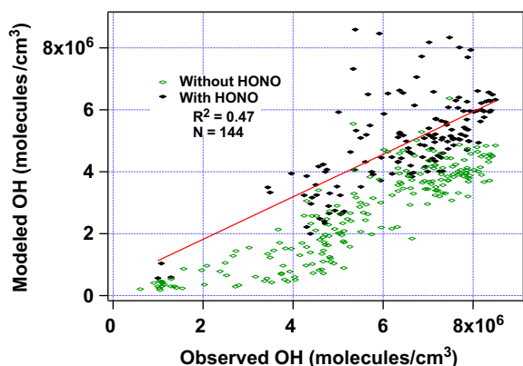
Fig. 8. Scatter plot of predicted versus measured OH radicals for the last four days of the field campaign (7/8–7/11, 2003). Model results without HONO are represented by open green diamonds and results with HONO are indicated by solid black diamonds. The linear regression is fit to model results with HONO.
