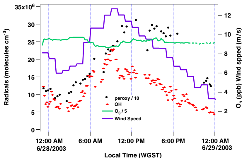
Fig. 12. Measured values for radicals, ozone and wind speed on 28 June. Black dots = peroxy radicals (number density/10), red diamonds = OH (number density), green line = ozone (ppbv/5) and blue line = wind speed ( \text{m s}^{-1} ).
