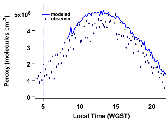
Fig. 7. Composite 24 h measurements and model predictions of peroxy radicals. Predicted values obtained from NMHC model constrained by \text{H}_2\text{O}_2 , \text{CH}_2\text{O} and HONO.
