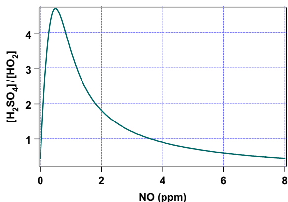
Fig. 3. Predicted yield of sulfuric acid versus nitric oxide mixing ratio at a fixed sulfur dioxide concentration of 32 ppmv. The mixing ratios of NO used during the Summit 2003 field campaign ranged from 3.2 to 6.4 ppmv. The reaction time was 100 ms.
