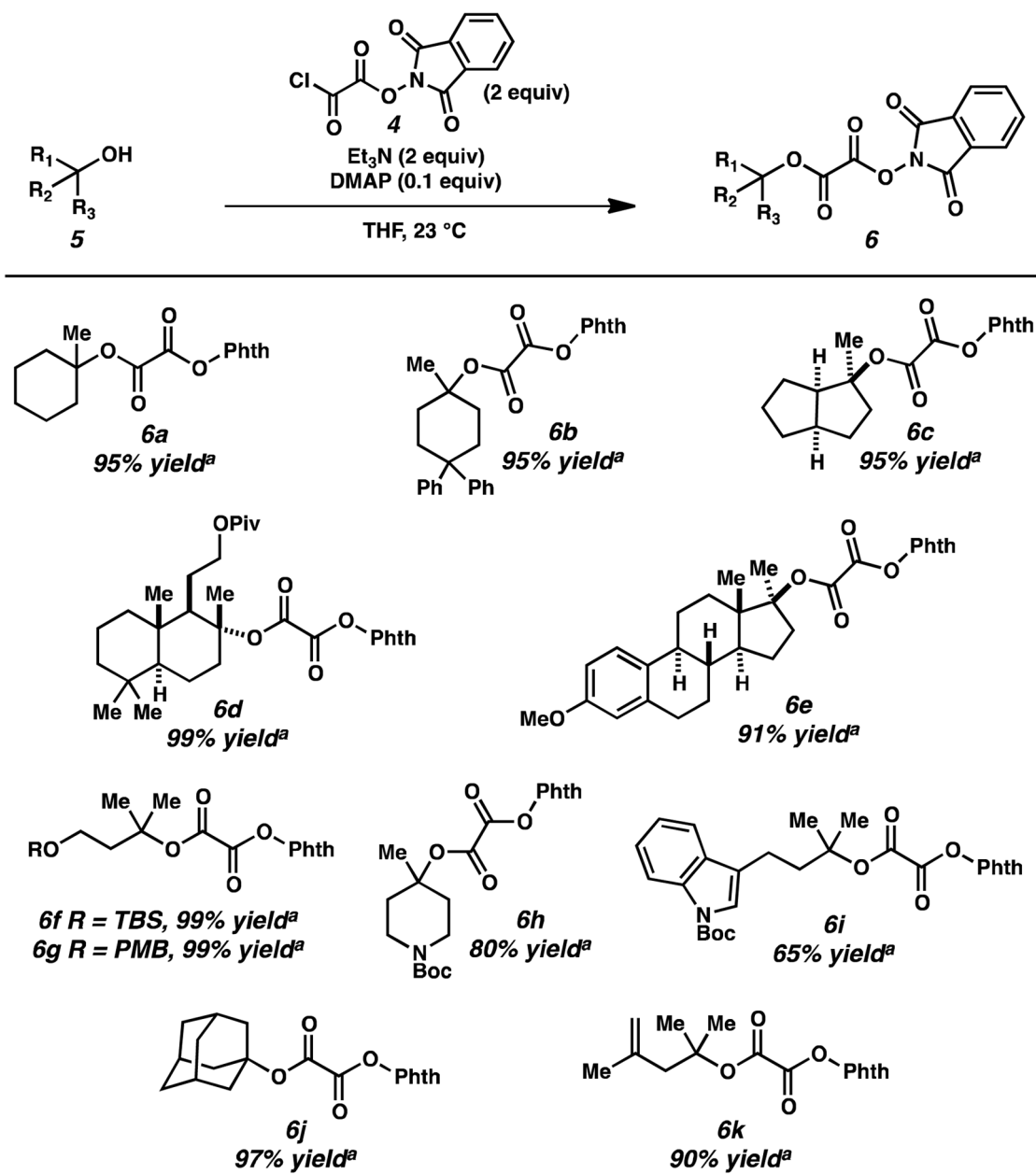
Figure 1. Synthesis of tert -alkyl N -phthalimidoyl oxalates
