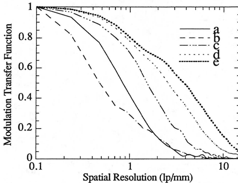
Fig.5.13 MTF calculated from LSF in Fig.5.12
