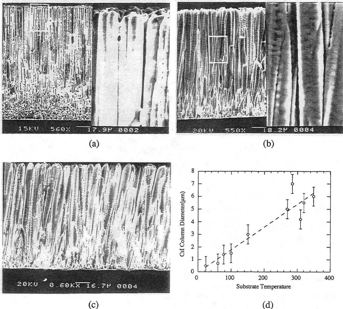
Fig.4.5 The dependence of the CsI column diameter on the substrate temperature. (a) T=100^{\circ}\text{C} ; (b) T=150^{\circ}\text{C} ; (c) T=200^{\circ}\text{C} ; and (d) diameter vs. Temperature.
