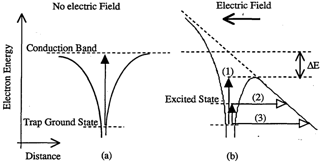
Fig. 2.9 Mechanisms of electron generation from recombination centers (a) Simple thermal generation, (b) Three effects of strong electric field; (1) Poole-Frenkel barrier lowering, (2) phonon assisted tunneling and (3) direct tunneling. Arrow \uparrow represents a thermal emission process and \rightarrow represents a field emission process.
