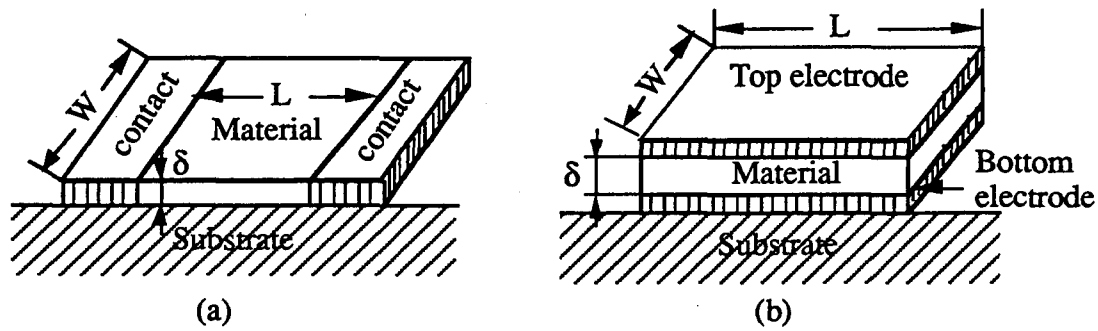
Fig.3.3 Photoconductor configuration: (a)coplanar structure; (b)sandwich structure.
