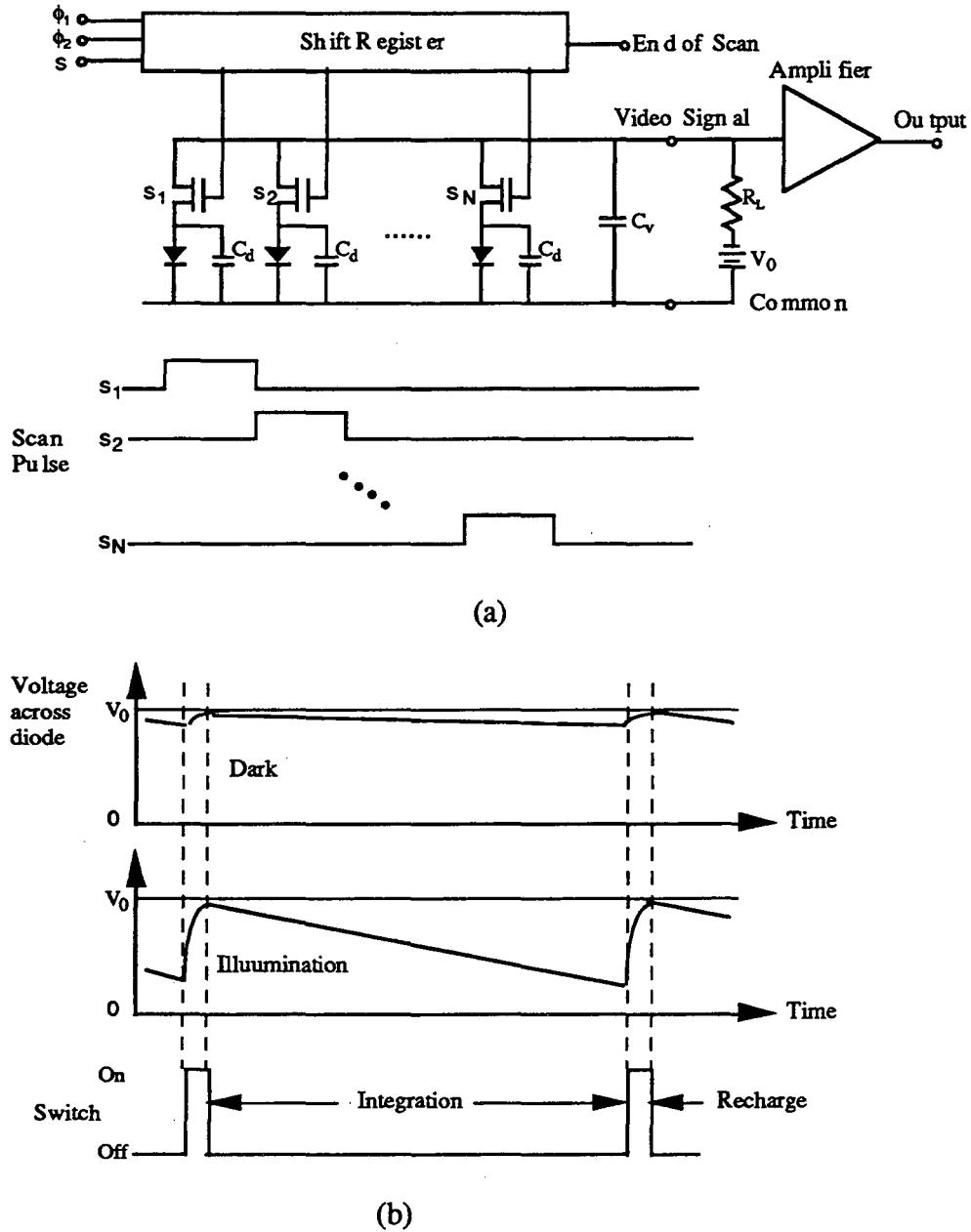
Fig.2.14 Operational model for the charge storage mode: (a) linear array of photodiodes connected to transfer switches(TFT); (b) storage and readout of the charge generated in a photodiode.
