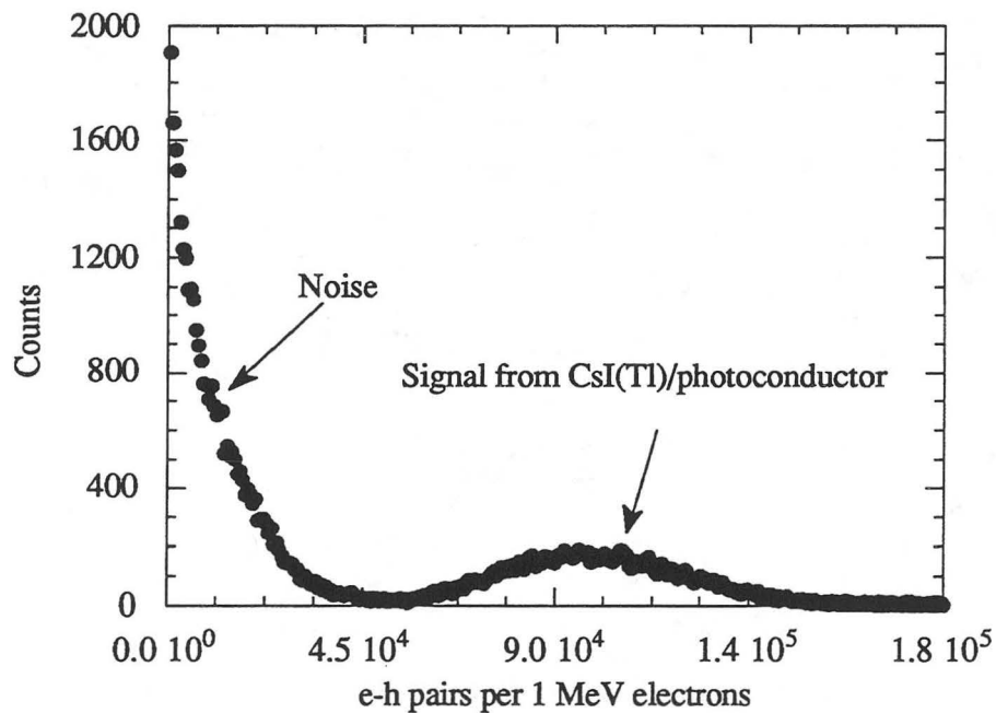
Fig.5.5 The detection of \beta particles from \text{Sr}^{90} by a CsI layer coupled to photoconductor with shaping time 2 \mu\text{s} .
