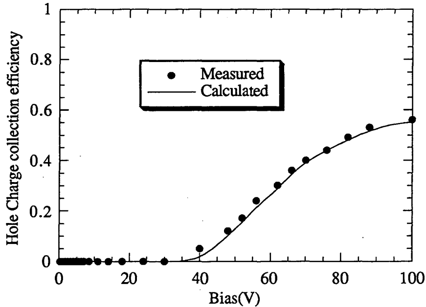
Fig. 2.3 Collection efficiency of holes in the cases of surface generation for a 10 \mu\text{m} thick sample. Dots are measured data from 560 nm light and lines are calculation results.
