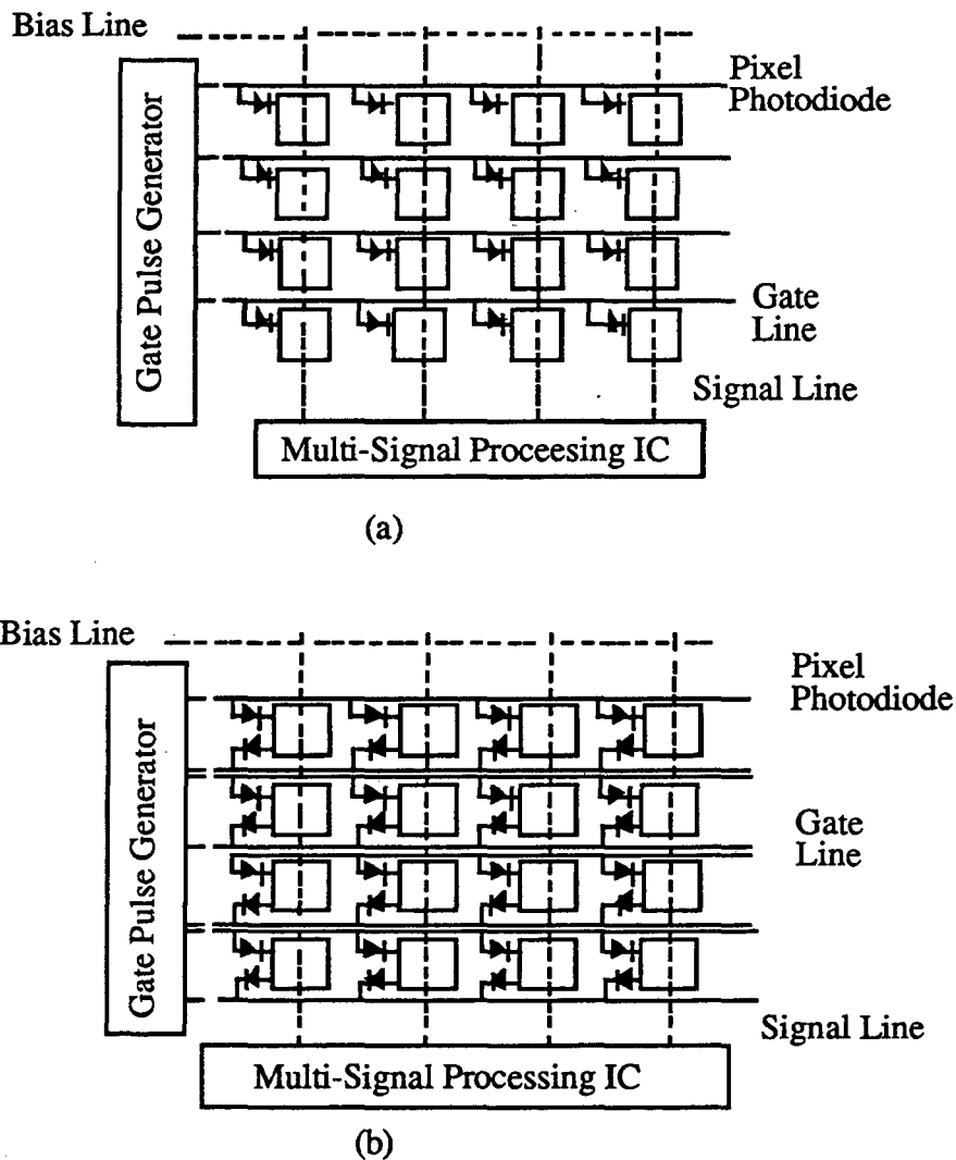
Fig.2.16 Diode readout schemes (a) single diode (b) two diode switches
