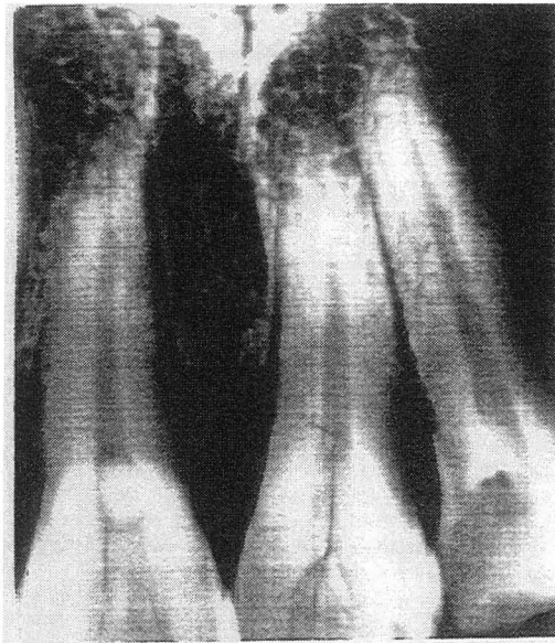
Fig.5.15 The tooth radiograph obtained with the CsI(Tl)/photosensor array imager.
