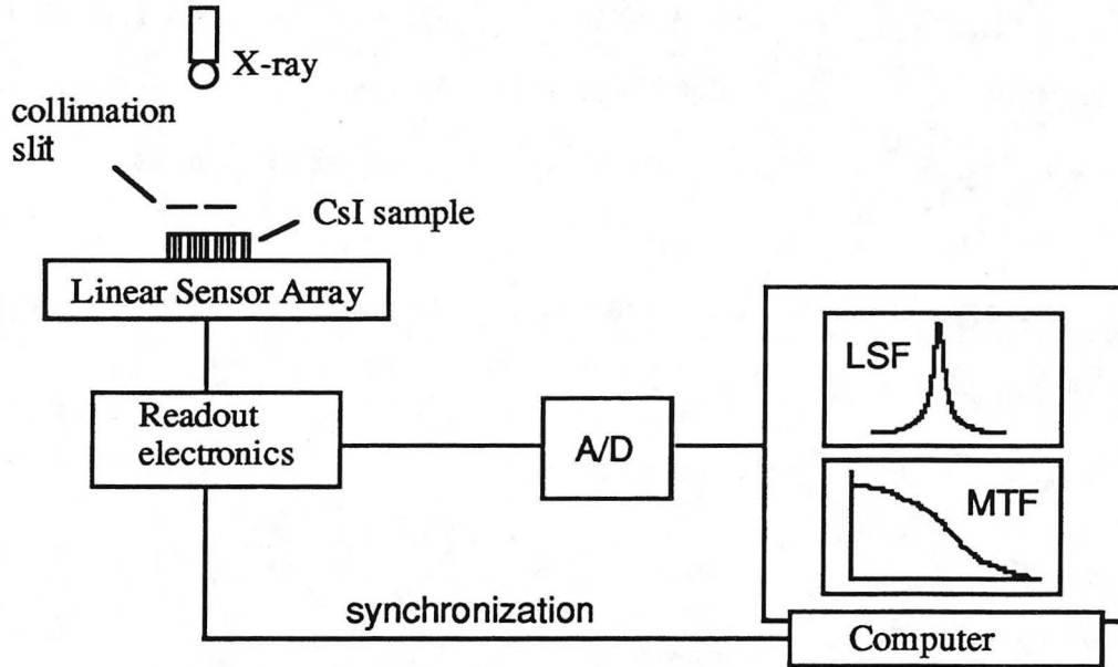
Fig.5.9 Schematic of LSF and MTF measurement setup.
