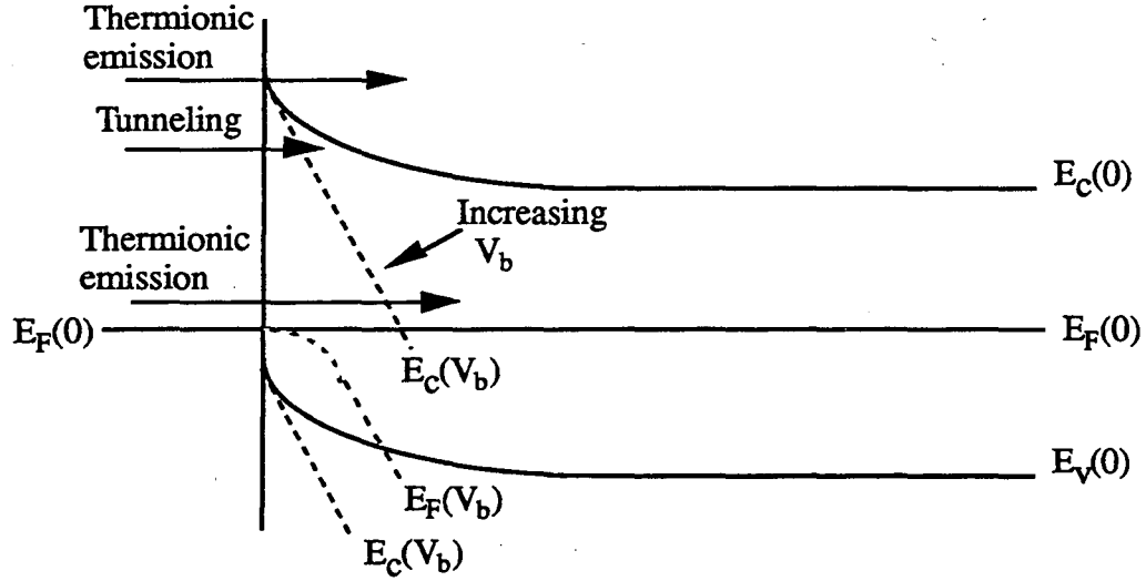
Fig.2.7 The three main mechanisms of electronic transport across the barrier. The dashed lines represent the change in potential profile when a reverse bias V_b is applied.
