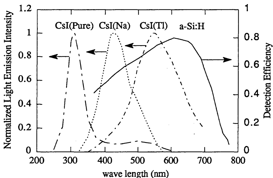
Fig.1.5 Scintillation light spectra of CsI(Tl) and CsI(Na) and detection efficiency of a-Si:H photodiodes.
