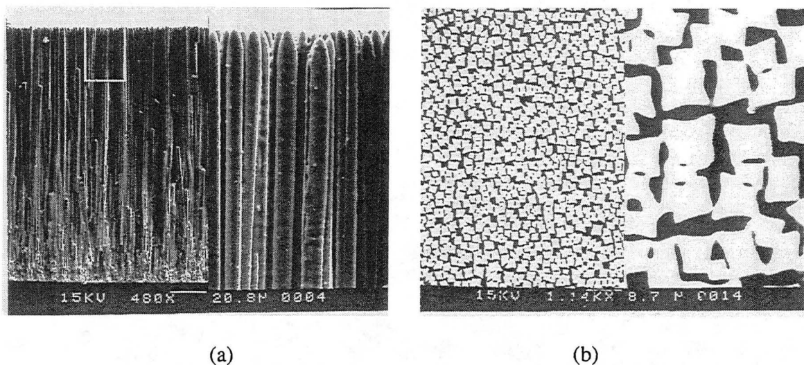
Fig.4.20 (a) Columnar structure CsI deposited on a flat substrate with elevated inert gas pressure. (b) Top of view of the layer.
