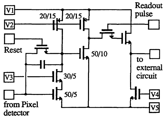
Fig.2.19 Polysilicon TFT charge sensitive amplifier
