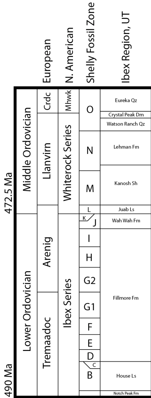
Figure 10. Stratigraphy of the Ibex Region, the study area. This study examined the Wah Wah formation, Juab formation, Kanosh shale and Lehman formation, which span the Ibexian/Whiterockian boundary. Shelly fossil zones are designated by Hintze (1952).
