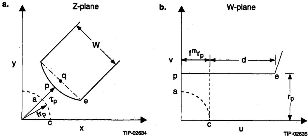
Figure 3. (a) Multipole Geometry ( x -Plane) and (b) Multipole Transformed to Dipole ( w -Plane).
