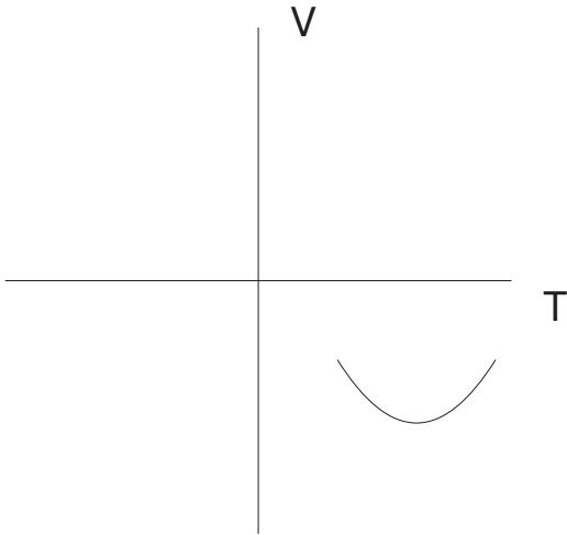
Figure 2: Tachyon at minimum of its potential
