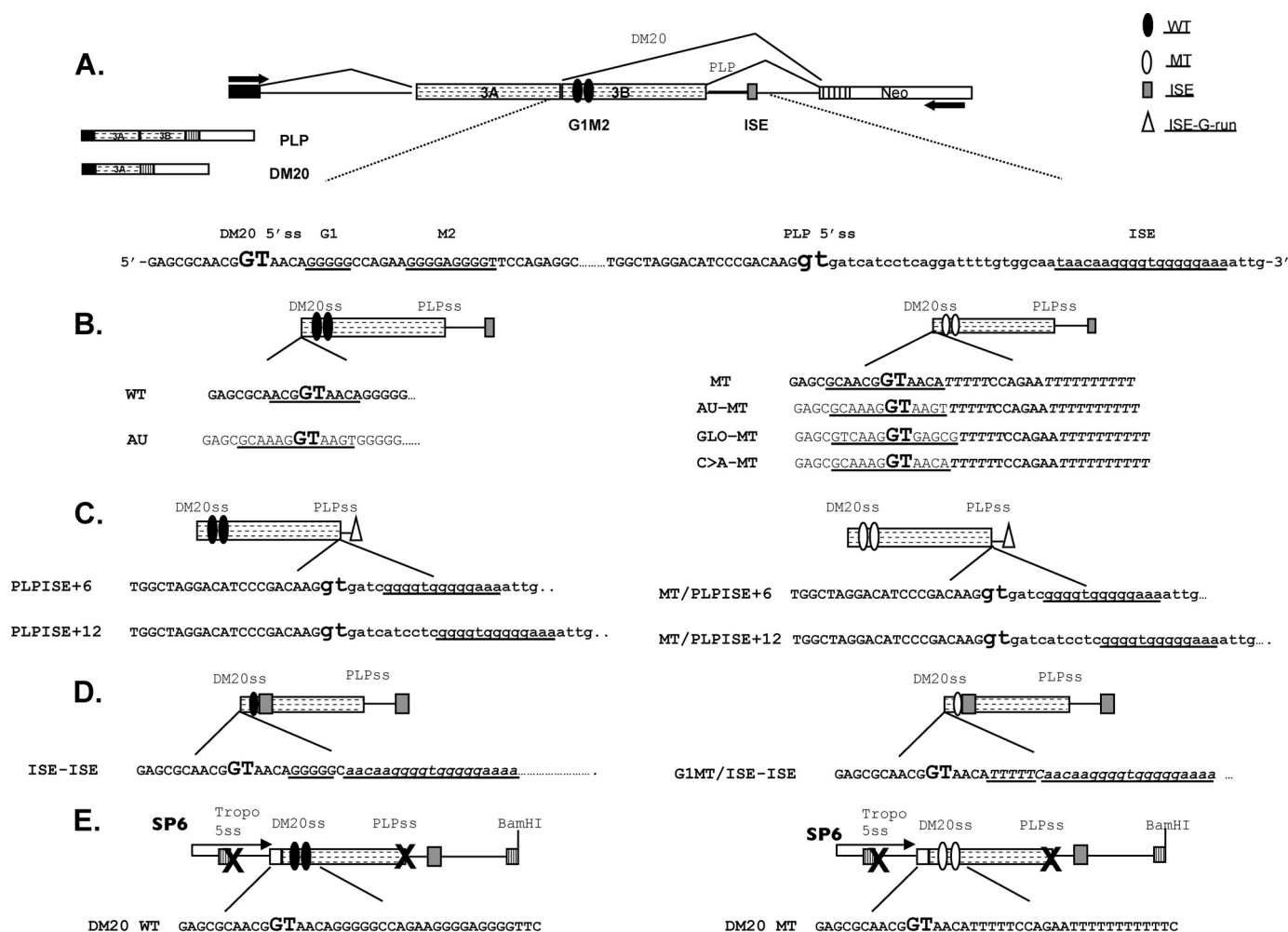
FIGURE 1. PLP constructs. A, schematic of the PLP-neo splicing minigene construct. The arrows indicate the position of the PCR primers. The PLP and DM20 PCR products and partial sequences of PLP exon 3B (uppercase letters) and intron 3 (lowercase letters) in PLP-neo (WT) are shown; DM20 and PLP 5' splice site are enlarged and in bold type; and G1, M2, and ISE are underlined. The filled ovals represent the wild type G1M2, empty ovals represent the G1M2 mutated to polyT, the shaded rectangle is the ISE, and the empty triangle represents the G runs of the ISE. B, schematics and sequences of the constructs in which the DM20 5' ss has been mutated to a stronger 5' ss: AU (canonical), GLO ( \alpha -globin), and C \rightarrow A (disease-associated mutation (28)). The sequences of natural DM20 5' ss and the strong 5' ss are underlined. C, schematics and sequences of the constructs in which the G runs of the ISE (empty triangle) are moved 6 nucleotides (PLPISE+6) and 12 nucleotides (PLPISE+12) downstream of the PLP 5' ss. The sequence of the ISE is underlined. D, schematics and sequences of the constructs in which the ISE replaces the M2. The G1, G1MT, and ISE sequences are underlined. E, schematics and sequences of the PY7 constructs generated for in vitro splicing and spliceosomal assembly (see "Experimental Procedures" for details). PLP exon 3A last 10 nucleotides, exon 3B, and intron 3 are cloned into the tropomyosin ( Tropo ) gene. The X indicates that the 5' ss of tropomyosin exon 2 and PLP 5' ss are mutated. DM20 WT contains the natural exon 3B sequences, whereas DM20 MT contains G1M2 mutated to poly Ts. SP6 refers to the promoter that drives in vitro transcription.
