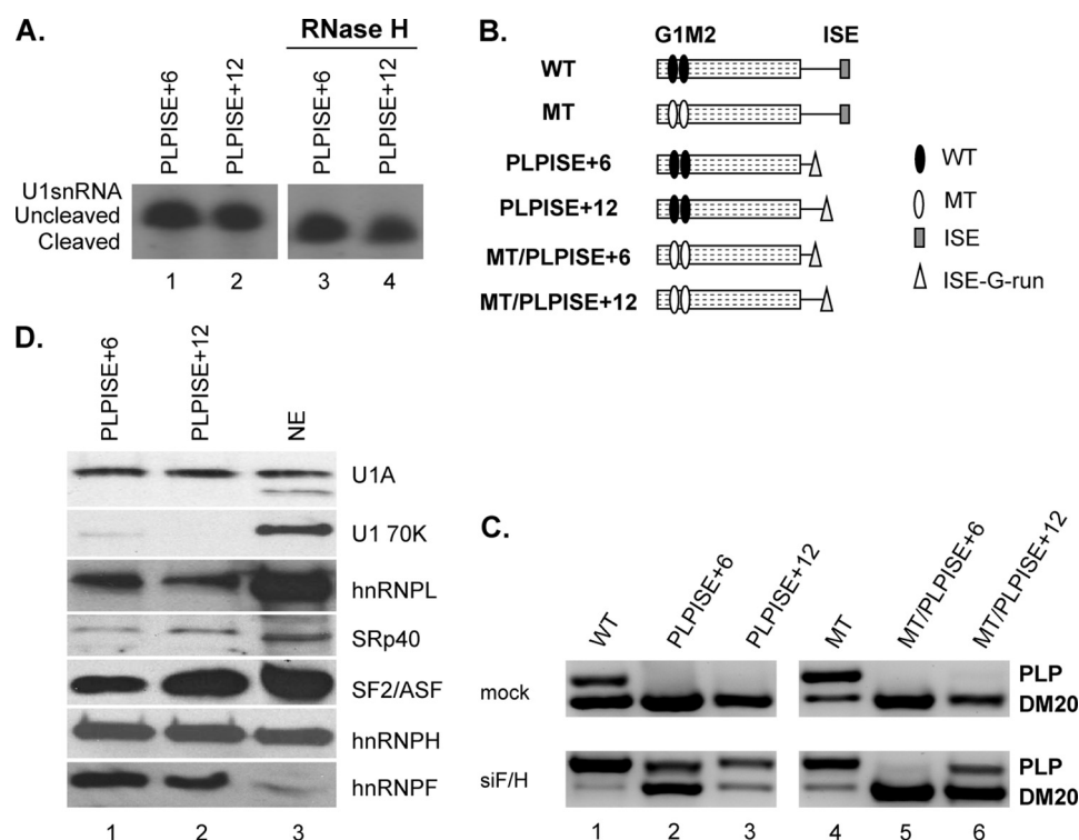
FIGURE 8. The function of the ISE is dependent on context and distance from the PLP 5' splice site. A, representative primer extension analysis of U1snRNA bound to the PLP RNAs. Untreated (lanes 1 and 2) and RNase H-treated (lanes 3 and 4) HeLa nuclear extracts were incubated with the biotinylated RNA templates indicated (sequences in Table 1). The RNA was extracted from the streptavidin bead precipitates and assayed by reverse transcription with a primer complementary to loop 2 of the U1sn RNA ( n = 2 ). The extension products from cleaved and uncleaved U1snRNA are shown. B, schematic representation of all constructs (see also Fig. 1). C, representative RT-PCR analysis of PLP and DM20 products amplified in RNA isolated from Oli-neu cells transfected with WT, PLP/ISE+6, PLP/ISE+12, MT, MT/PLP/ISE+6, and MT/PLP/ISE+12 and treated with siF/H ( n = 3 ) (30 PCR cycles). Mock are cells transfected with the same plasmids and treated with scrambled siRNA (30 PCR cycles). D, representative Western blot analysis of RNA affinity precipitates of PLP/ISE+6 and PLP/ISE+12 (lanes 1 and 2, respectively) (sequences in Table 1) incubated with untreated HeLa nuclear extract ( n = 2 ). Lane 3 is the HeLa nuclear extract. The precipitates were separated by SDS-PAGE, blotted, and probed with antibodies to U1A, U170K, SF2/ASF, SRp40, hnRNPL, hnRNPH, and hnRNPF.
