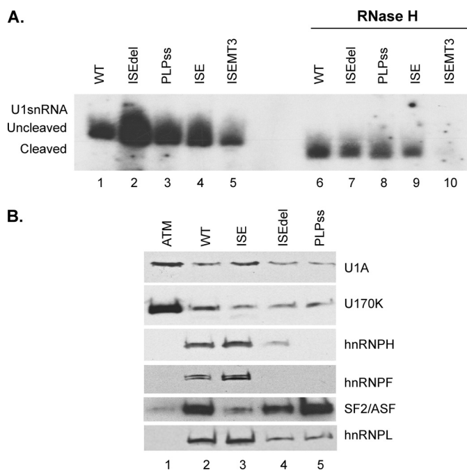
FIGURE 6. The PLP U1snRNP-pre-mRNA complex does not require the ISE. A, representative primer extension analysis of U1snRNA bound to PLP RNAs. Untreated (lanes 1–5) and RNase H-treated (lanes 6–10). HeLa nuclear extracts were incubated with the biotinylated RNA templates indicated (sequences in Table 1). The RNA was extracted from the streptavidin bead precipitates and assayed by reverse transcription with a primer complementary to loop 2 of the U1sn RNA ( n = 3 ). The extension products from cleaved and uncleaved U1snRNA are shown. B, representative Western blot analysis of RNA affinity precipitates of the indicated RNA templates (sequences in Table 1) incubated with untreated HeLa nuclear extracts ( n = 2 ). The precipitates were separated by SDS-PAGE, blotted, and probed with antibodies to U1A, U170K, SF2/ASF, hnRNPH, hnRNPF, and hnRNPL.
