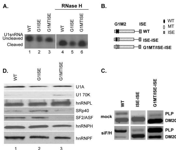
FIGURE 7. The ISE recruits U1snRNA to the DM20 5' splice site and is a strong enhancer of DM20 splicing. A, representative primer extension analysis of U1snRNA bound to the RNAs. Untreated (lanes 1–3) and RNase H-treated (lanes 4–6) HeLa nuclear extracts were incubated with the biotinylated RNA templates indicated (sequences in Table 1). The RNA was extracted from the streptavidin bead precipitates and assayed by reverse transcription with a primer complementary to loop 2 of the U1sn RNA ( n = 3 ). The extension products from cleaved and uncleaved U1snRNA are shown. B, schematic representation of minigene constructs (see also Fig. 1). C, representative RT-PCR analysis of PLP and DM20 products amplified in RNA isolated from Oli-neu cells transfected with WT, ISE-ISE, G1MT/ISE-ISE, and treated with siF/H ( n = 3 ) (30 PCR cycles). Mock are cells transfected with the same plasmids and treated with scrambled siRNA (30 PCR cycles). D, representative Western blot analysis of RNA affinity precipitates of WT (lane 1), G1ISE (lane 2), and G1MTISE (lane 3) RNAs (sequence is shown in Table 1) incubated with untreated HeLa nuclear extract ( n = 2 ). The precipitates were separated by SDS-PAGE, blotted, and probed with antibodies to U1A, U170K, SF2/ASF, SRp40, hnRNPL, hnRNPH, and hnRNPF.
