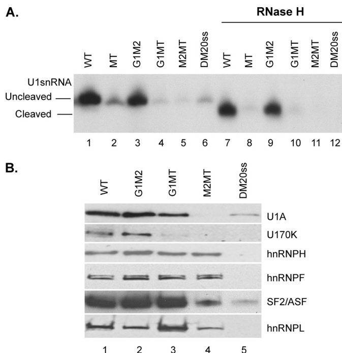
FIGURE 3. G1M2 recruits U1snRNA to the DM20 5' splice site. A, representative primer extension analysis of U1snRNA bound to DM20 RNAs. Untreated (lanes 1–6) and RNase H-treated (lanes 7–12) HeLa splicing extracts were incubated with the biotinylated RNA templates indicated (sequences in Table 1). The RNA was extracted from the streptavidin bead precipitates and assayed by reverse transcription with a primer complementary to loop 2 of the U1snRNA. The extension products from cleaved and uncleaved U1snRNA are shown ( n = 2 ). B, representative Western blot analysis of RNA affinity precipitates with the indicated RNA templates (sequences in Table 1) incubated with untreated HeLa nuclear extracts ( n = 2 ). The precipitates were separated by SDS-PAGE, blotted, and probed with antibodies to U1A, U170K, SF2/ASF, hnRNPH, hnRNPF, and hnRNPL.
