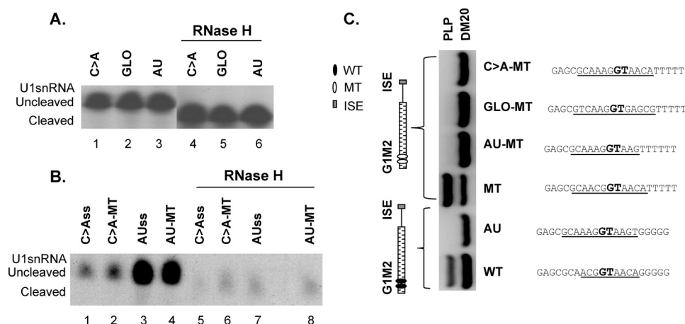
FIGURE 4. Functional relationship of G1M2 with the strength of the 5' splice site. A and B, representative primer extension analysis of U1snRNA bound by RNAs in which the DM20 5'ss is replaced by strong 5'ss. Untreated (A, lanes 1–3, and B, lanes 1–4) and RNase H-treated (A, lanes 4–6, and B, lanes 5–8) HeLa splicing extracts were incubated with the biotinylated RNA templates indicated (sequences in Table 1). The RNA was extracted from the streptavidin bead precipitates and assayed by reverse transcription with a primer complementary to loop 2 of the U1snRNA. The extension products from cleaved and uncleaved U1snRNA are shown ( n = 2 ). C, schematic representation of the constructs. The sequences of the 5'ss: AU, C → A, and GLO that replace the natural DM20 5'ss are shown. The GT is indicated in bold type . Representative RT-PCR analysis of PLP and DM20 products amplified in RNA isolated from Oli-neu cells transfected with WT, AU, MT, AU-MT, GLO-MT, and C → A-MT ( n = 2 ) (30 PCR cycles).
