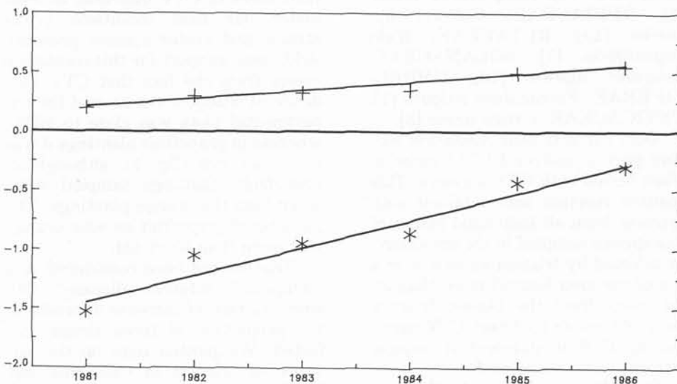
Fig. 2. Progress of tristeza in a grapefruit plot in Southern Valencia (Spain). Per unit incidence of tristeza (x) plotted as \ln x/1-x (*) and as \ln 1/1-x (+).
