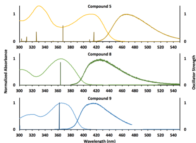
Fig. 2 UV-visible absorption and fluorescence spectroscopic traces of Compounds 5 (top), 8 (middle), and 9 (bottom) superimposed upon their respective calculated optical transitions.
