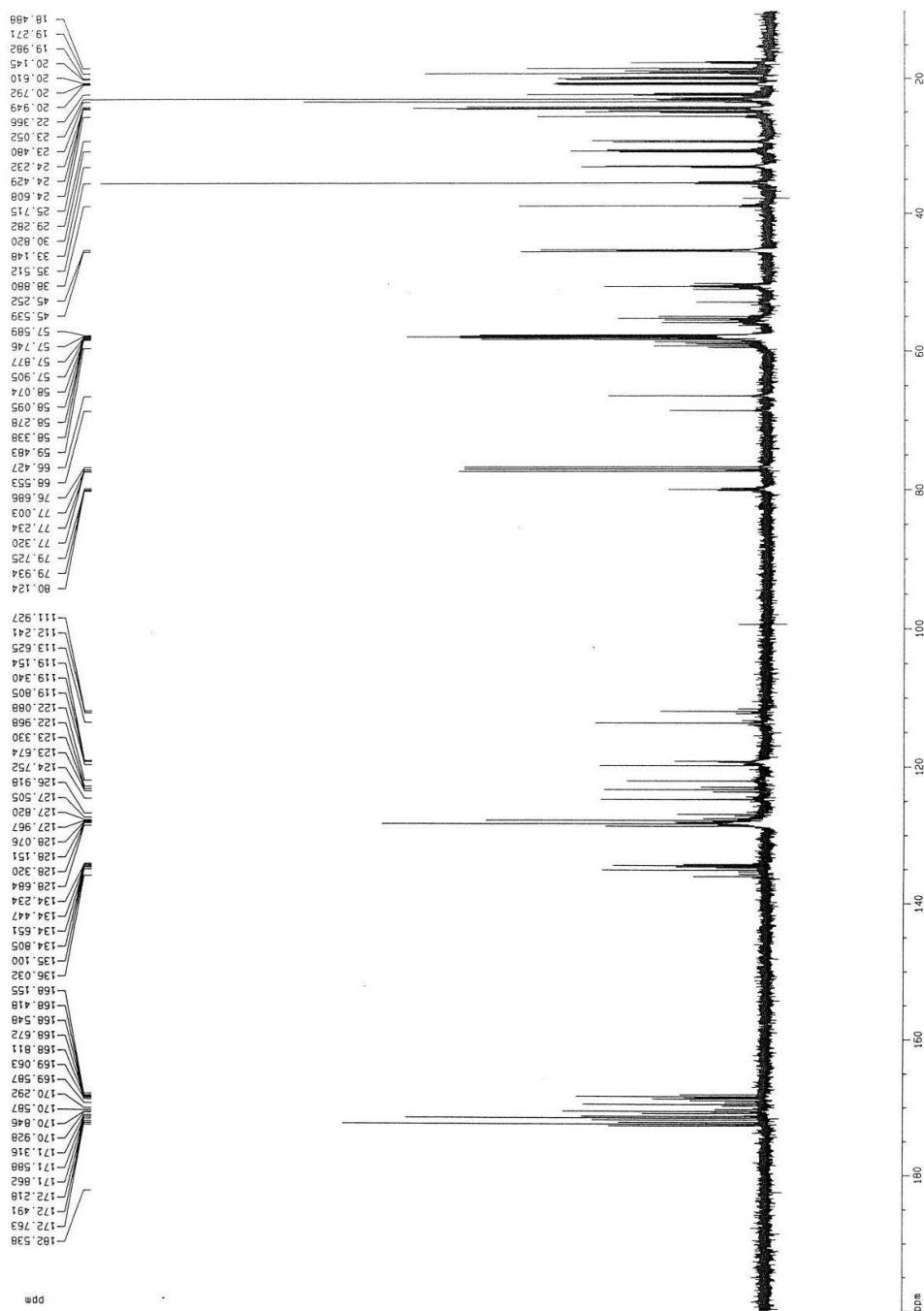
Appendix Figure 2.S8: ^{13}\text{C} spectrum of cyclamarin A from [\text{U-}^{13}\text{C}_6] glucose feeding (1a) in \text{CDCl}_3
