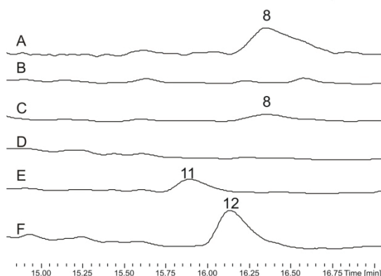
Appendix Figure 3.S1: Analysis of relative yield of cyclomarin analogs in Salinispora arenicola CNS-205 wild type and cymD - mutant. Trace A: Wild type S. arenicola CNS-205. Trace B-F, S. arenicola cymD - mutant. Traces C-F represent cultures supplemented with 80 mg/L tryptophan analogs. Trace C: N -(1,1-dimethyl-1-allyl)-tryptophan, D: tryptophan, E: N -(1-methyl)-tryptophan, F: N -(1-propargyl)-tryptophan. Chromatograms recorded at 210 nm. Note similar production levels of cyclomarin M ( 11 , trace E) and cyclomarin P ( 12 , trace F) in comparison to cyclomarin A ( 8 ) in trace A and C. Desprenylcyclomarin C ( 10 , RT=15.2 min) is produced at levels below the detection limit of this analysis in the cymD - mutant (trace B), and did not increase to a detectable level with the addition of tryptophan (trace D).
