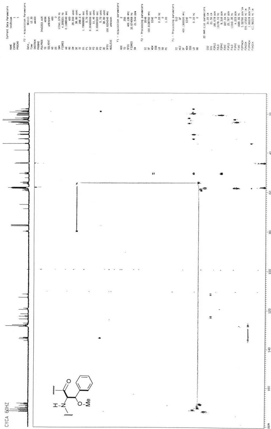
Appendix figure 2.S16: 2D INADEQUATE NMR spectrum of 1a in \text{CDCl}_3 showing \beta -OMe-Phe residue couplings
