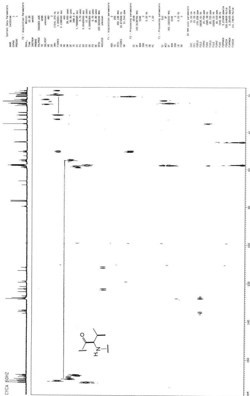
Appendix figure 2.S18: 2D INADEQUATE NMR spectrum of 1a in \text{CDCl}_3 showing Val residue couplings
