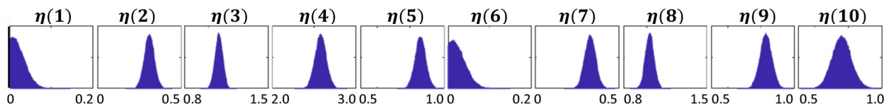
Figure 4. Marginal distributions of the population-level hyperparameters \eta . See Table 3 for correspondence with PTM parameters.
