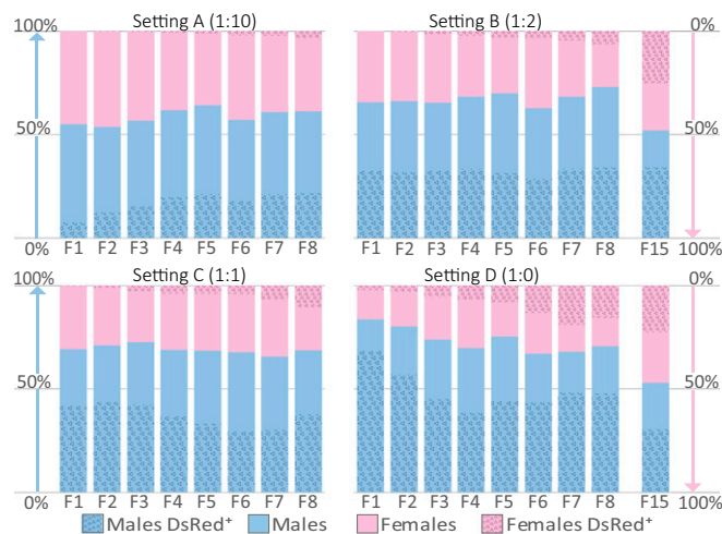
Fig. 3. Dynamics of sex ratio and indicated resistance allele spread in population experiments. w^{-} virgins were crossed with various ratios of CHE ( tra^{nCHE}/+ ) and wild-type ( w^{-} ) males (settings A–D). For each setting five replicates were carried out (SI Appendix, Fig. S6). Progeny were screened for sex and the presence of the DsRed eye marker for up to 15 generations. In setting D, where only tra^{nCHE} males were used, a sex ratio of over 80% males was achieved within one generation, indicating the collapse potential of this forced male offspring-only system. In XX embryos, tra^{nCHE} attacks the wild-type tra locus in somatic cells, resulting in intersex individuals (SI Appendix, Fig. S2). Thus, only females carrying nonfunctional defective tra^{nCHE} or drive-resistant functional tra^{Rst} alleles can show the DsRed marker. Therefore, the DsRed marker serves as an indicator for the presence of the tra^{Rst} allele in females, and the rise in the percentage of DsRed females indicates the spread of resistance in the population. Screening the F 15 progeny in settings B and D showed that the populations adapted to the presence of the tra^{nCHE} homing allele with the female sex ratio returning to about 50% (SI Appendix, Fig. S6).
