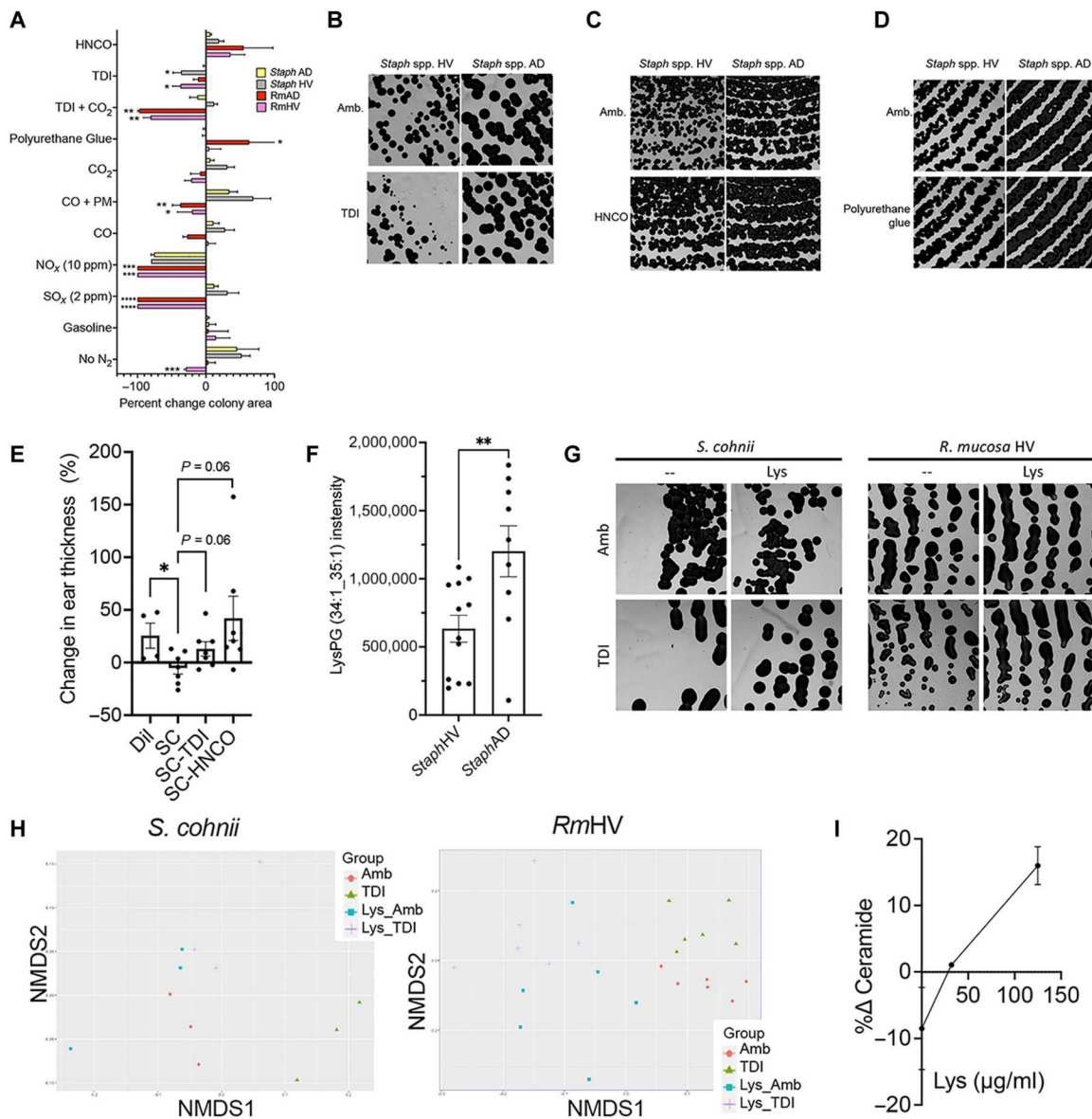
Fig. 8. TDI and HNCO disrupt beneficial pathways in S. cohnii . (A) Percent change in growth area for RmHV 1-3, RmAD 1-3, Staph HV1-3, and Staph AD1-3 as quantified from images shown in Figs. 1I, 2C, 4D, 5 (A, E, F, and I), and 8 (B to D and G). Significance is indicated versus Staph AD group. Impacts of NO x on Staph taken from (62). (B to D) Representative image of Staph HV1-3 and Staph AD1-3 cultured with TDI (B), HNCO (C), or polyurethane-containing glue (D). (E) Change in mouse ear thickness in MC903 mouse model after treatment with S. cohnii grown under ambient conditions or with exposure to TDI or HNCO. (F) Intensity levels of LysPG identified by mass/charge ratio and collisional cross section for the three isolates of Staph HV and three isolates from Staph AD. (G and H) Representative images (G) and non-metric multi-dimensional scaling (NMDS) plots (H) for S. cohnii and RmHV 1 exposed to TDI with and without pretreatment with lysine (Lys) supplementation. (I) Change in total annotated ceramides with exposure to TDI versus ambient for RmHV with and without Lys supplementation pretreatment. All images were taken at \times 1.25 magnification. Data are representative of two or more independent experiments and are displayed as means \pm SEM. * P < 0.05 , ** P < 0.01 , and *** P < 0.001 as determined by ANOVA.
