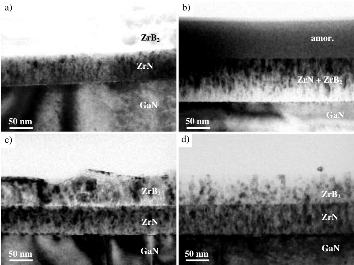
Fig.1. XTEM micrographs of \text{ZrN}/\text{ZrB}_2 bilayers deposited on GaN MOCVD layers: (a) as-deposited structure, (b) structure annealed under \text{O}_2 flow for 5min at 800^\circ\text{C} and (c), (d) structures annealed under \text{N}_2 flow for 5min at 800^\circ\text{C} and 30s at 1000^\circ\text{C} , respectively.
