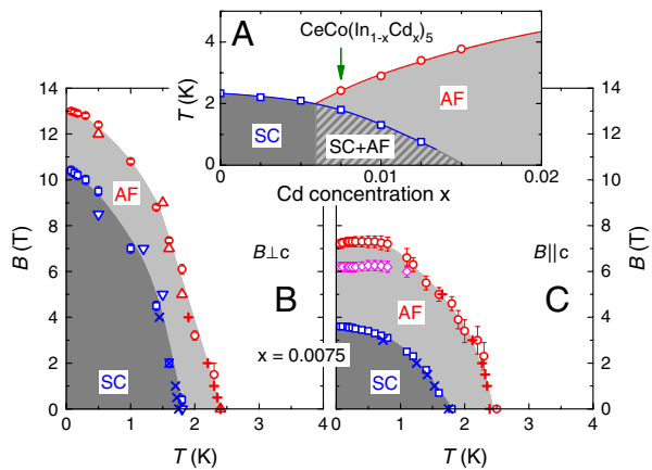
Fig. 1. (A) Doping x dependence of AF and superconducting (SC) transition temperatures in \text{CeCo}(\text{In}_{1-x}\text{Cd}_x)_5 for Cd-content x \leq 0.02 (after ref. 7). The crystals investigated here (arrow) exhibit both transitions. (B) B - T phase diagram of \text{CeCo}(\text{In}_{0.9925}\text{Cd}_{0.0075})_5 obtained from magnetotransport (circle, square), neutron scattering (triangle, upside-down triangle) and heat capacity (+, x) measurements with B \perp c . (C) B - T diagram for B \parallel c from magnetotransport and heat capacity. Indications of a transition within the AF phase are found (diamond).
