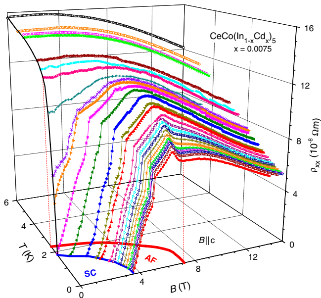
Figure 4. (A) Magnetic field dependence of the resistivity \rho_{xx} as measured in \text{CeCo}(\text{In}_{0.9925}\text{Cd}_{0.0075})_5 at different temperatures with B \parallel c . The phase boundaries associated with superconductivity and antiferromagnetism are marked.
