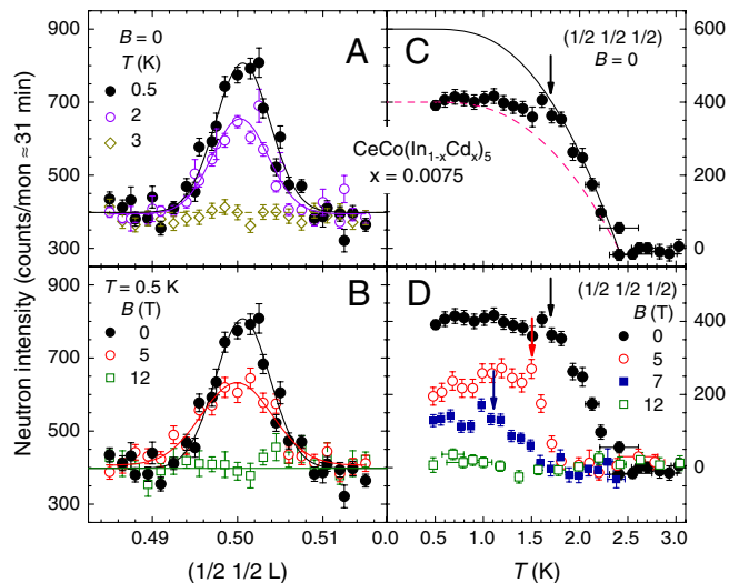
Fig. 2. Elastic neutron scattering scans in \text{CeCo}(\text{In}_{0.9925}\text{Cd}_{0.0075})_5 along [001] and across (\frac{1}{2}, \frac{1}{2}, \frac{1}{2}) : (A) at different temperatures in zero magnetic field and (B) for several magnetic fields at T = 0.5 K. Solid lines indicate fits with Gaussian lineshape to the data. (C) Temperature dependence of the magnetic intensity at (\frac{1}{2}, \frac{1}{2}, \frac{1}{2}) in B = 0 along with fits from mean-field expectations to the data (solid and dashed lines, see text). (D) Same as (C) in addition with data for several magnetic fields. The paramagnetic background contribution was subtracted from data in (C) and (D).
