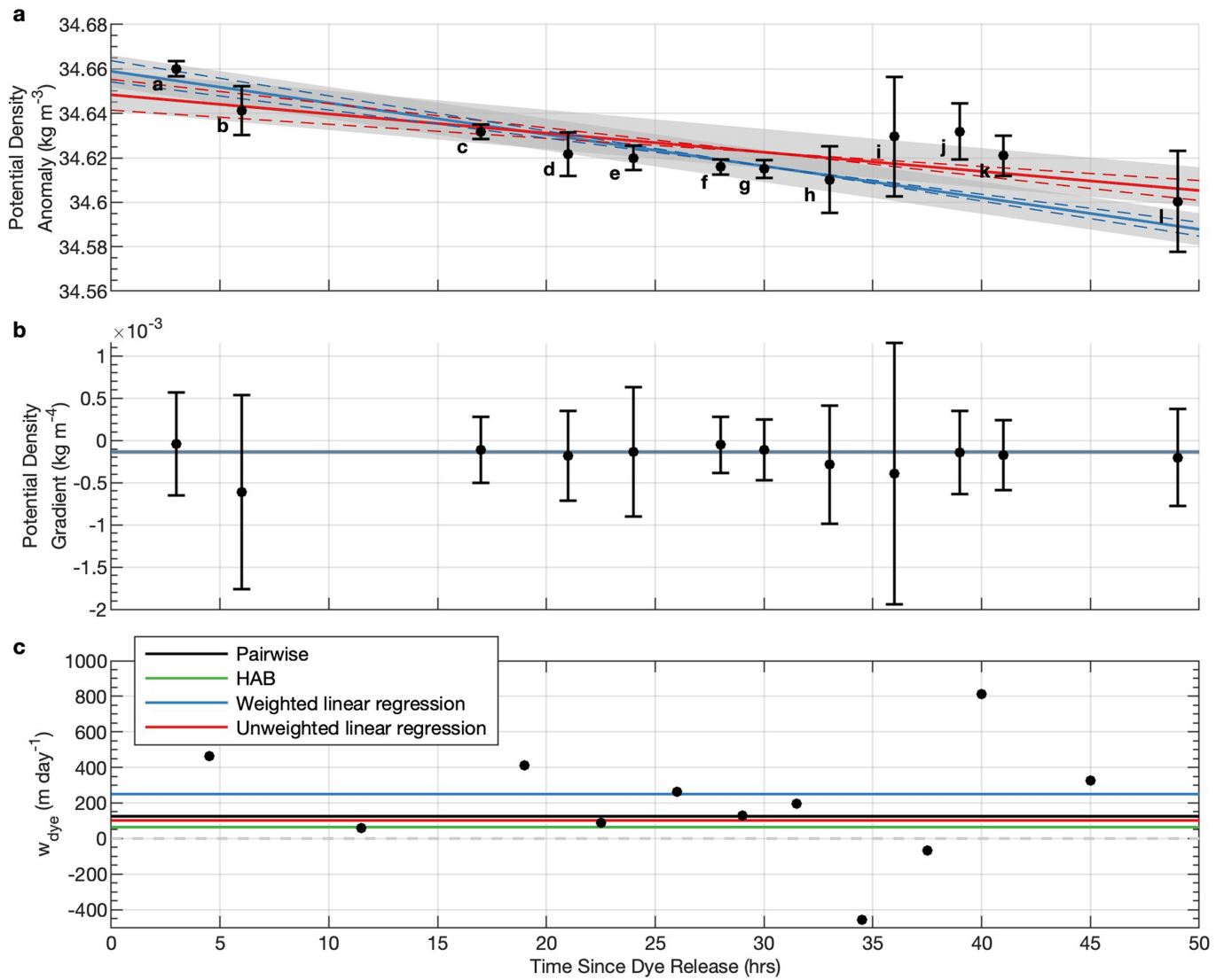
Extended Data Fig. 7 | Linear regression of the centres of mass of potential density anomaly, the gradient of potential density anomaly over time and estimates of upwelling velocity. (a) Weighed linear regression (solid blue line) and unweighted linear regression (solid red line) of the centres of mass in potential density anomaly space (black circles). Error bars show standard deviations of dye-weighted density for each transect. The residual standard error of the fit is denoted by the shaded region. Dashed lines show the fits given the standard error on the slope and intercept. The coefficient of determination R^2 for the weighted fit is 0.852 and for the unweighted fit is 0.587. (b) Centres of mass in potential density anomaly gradient space (black circles) and standard
