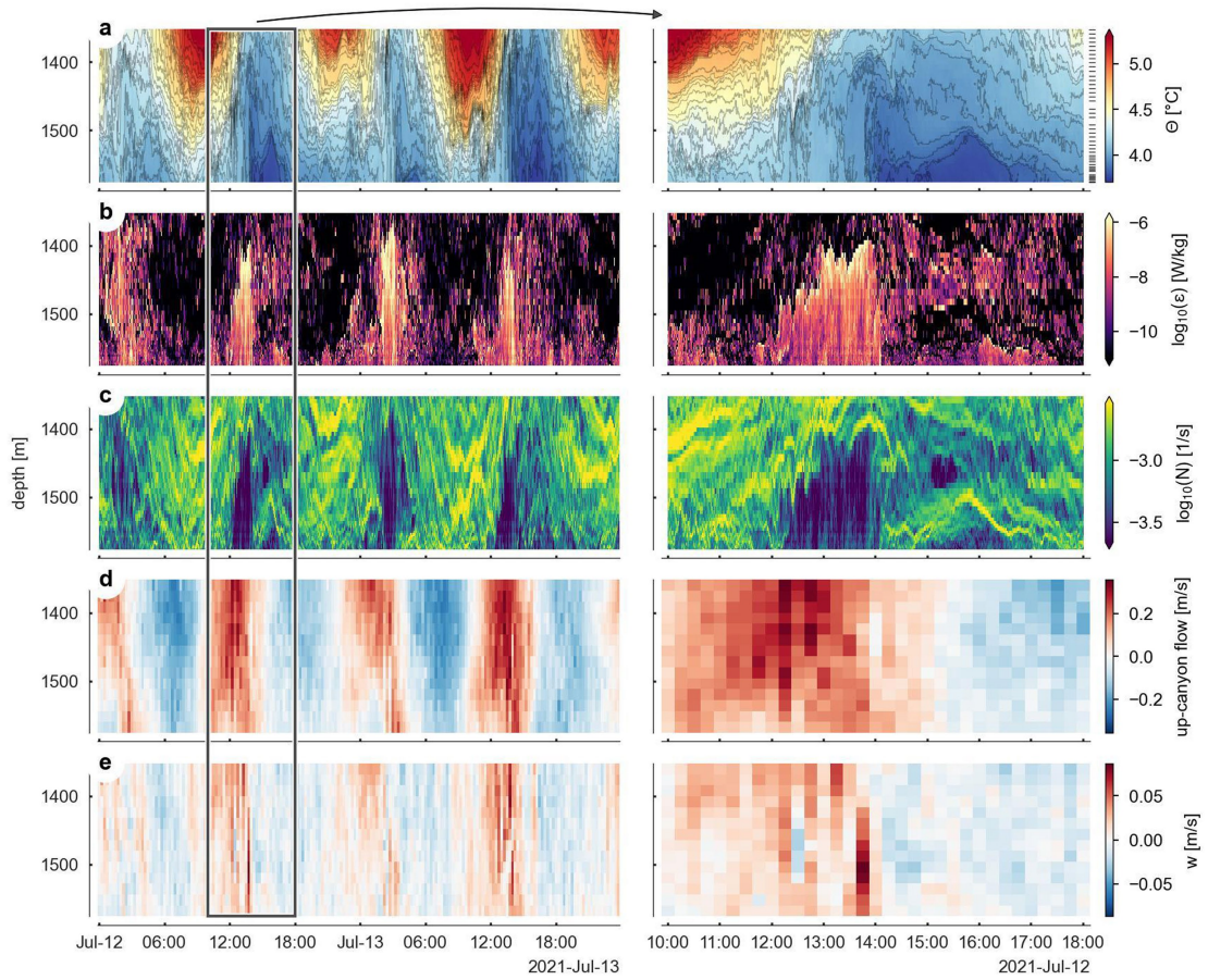
Extended Data Fig. 1 | Two-day snapshot and 8-hour zoom of flow conditions at MAVS1. (a) Potential temperature ( \theta ), (b) turbulent dissipation rate of kinetic energy ( \epsilon ) estimated from the sorting distance when sorting profiles into stable
