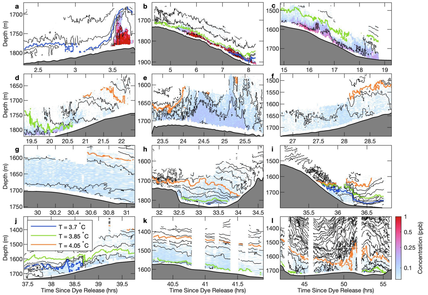
Extended Data Fig. 5 | All transects from the FCTD survey of the dye. (a)-(l) Dye concentration is shown on a logarithmic scale in parts per billion (ppb) in colour, isotherms every 0.05°C are shown with black contours, and
