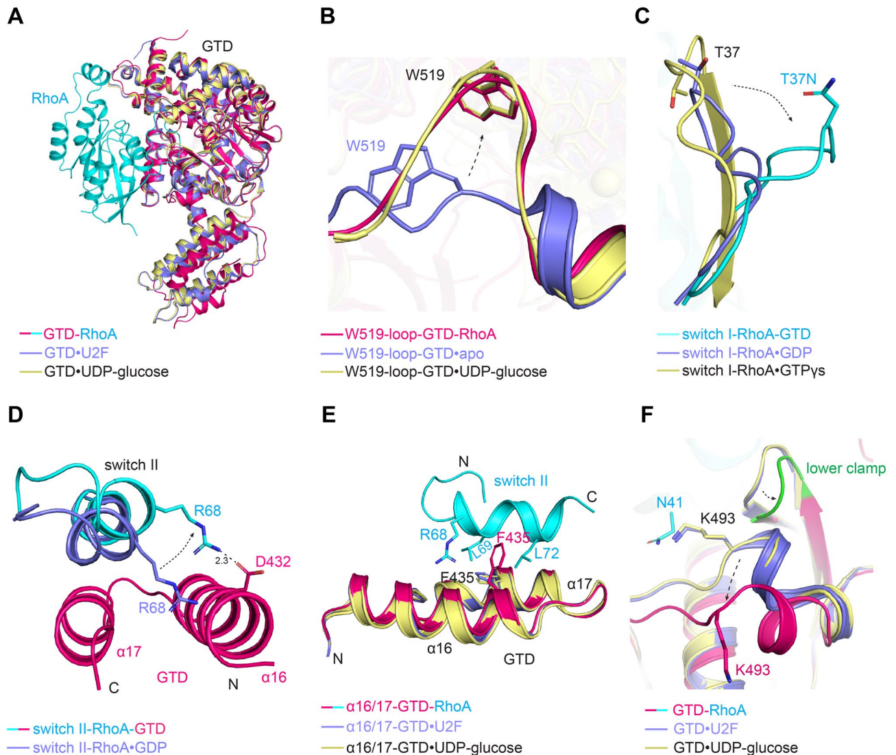
Figure 2. Conformational changes on GTD TcdA and RhoA induced by complex formation. (A) Structural superposition of the GTD TcdA -RhoA (hot pink and cyan, respectively) complex, GTD TcdA .U2F (slate, PDB code: 5UQL), and GTD TcdA .UDP-glucose (pale yellow, PDB code: 3SRZ) based on the GTD. (B) The W519-loop of GTD TcdA adopts a similar conformation in the GTD TcdA .UDP-glucose-RhoA complex (hot pink) and GTD TcdA .UDP-glucose (pale yellow), which is drastically different from that of the apo GTD TcdA (slate, PDB code: 4DMV). (C) Comparing the conformations of the switch I of RhoA in the GTD TcdA -RhoA-GDP complex (cyan), RhoA-GTPys (pale yellow, PDB code: 1A2B), and RhoA-GDP (slate, PDB code: 1FTN). (D) Comparing the conformations of the switch II of RhoA in the GTD TcdA -RhoA-GDP complex (cyan) and RhoA-GDP (slate, PDB code: 1FTN). (E) Superposition of RhoA-bound GTD TcdA .UDP-glucose (hot pink), GTD TcdA .U2F (slate) and GTD TcdA .UDP-glucose (pale yellow) focusing on the α16/17 helices. (F) GTD TcdA adopts conformational changes to accommodate the pre-switch I and switch I of RhoA when compared to the GTD TcdA .U2F (slate) and GTD TcdA .UDP-glucose (pale yellow) structures.
