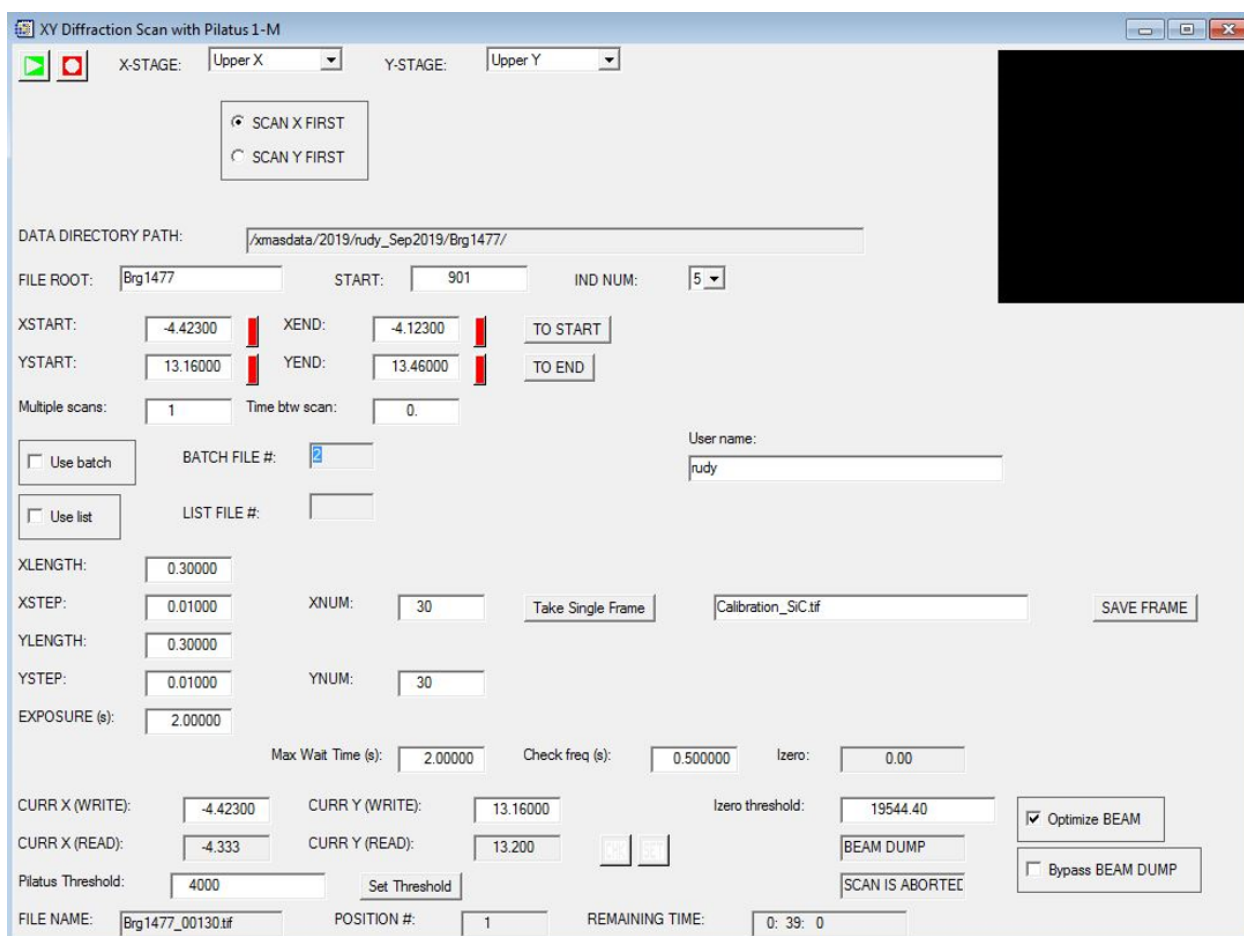
Figure 3.8: XY Diffraction Scan with Pilatus window used to program scan parameters
