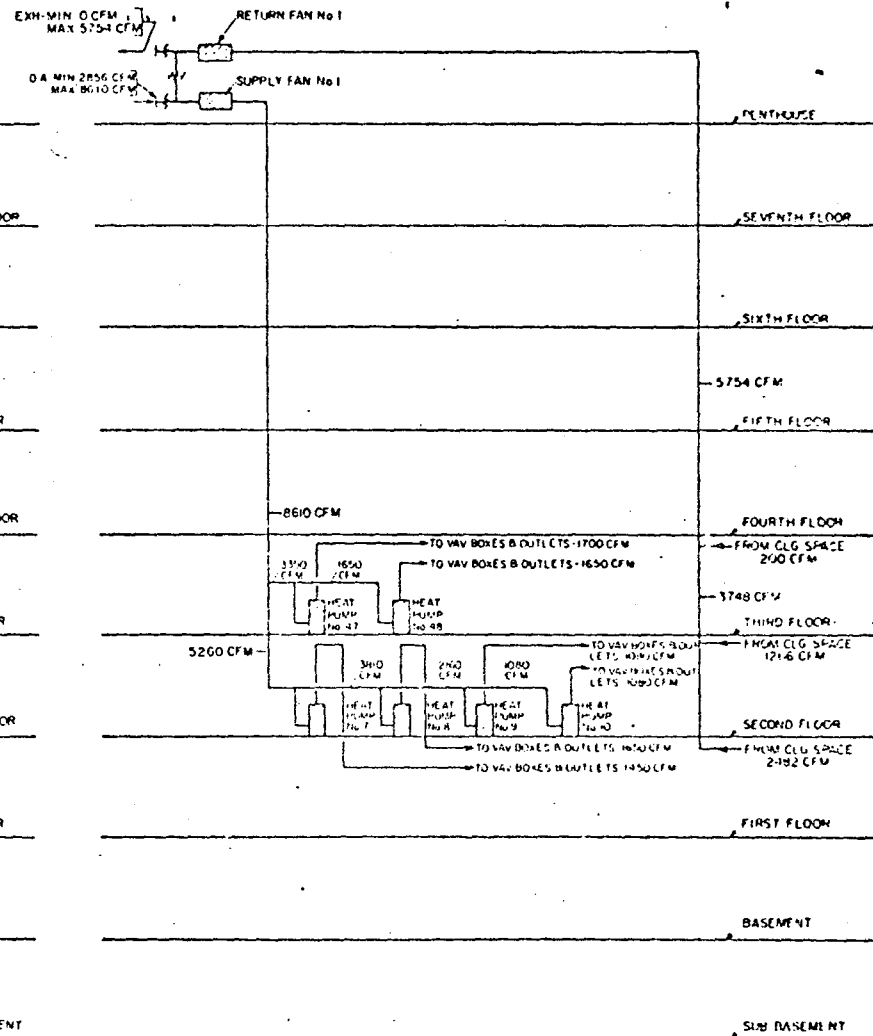
INTERIOR ZONE HEAT PUMP DUCT FLOW DIAGRAM NO SCALE
