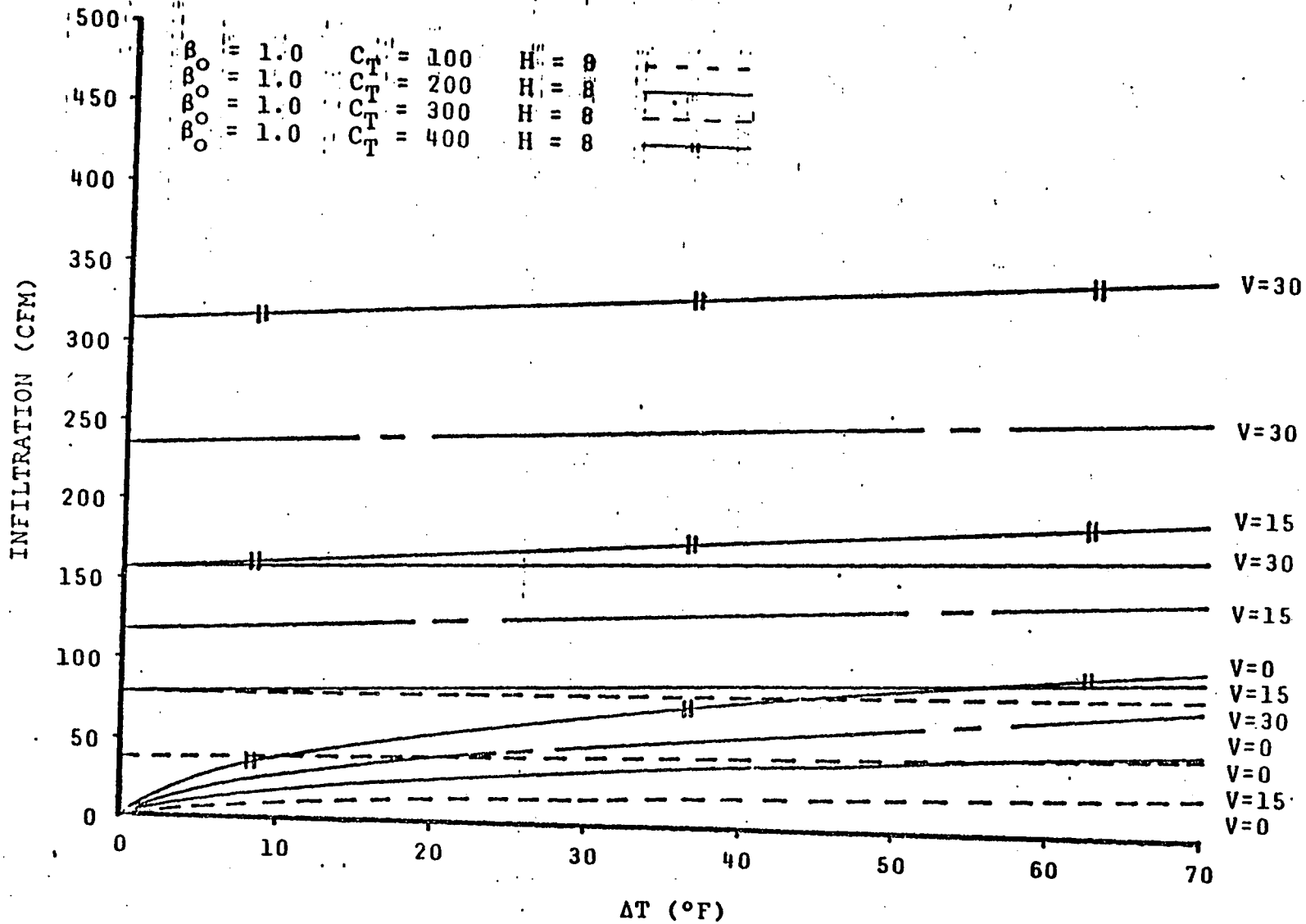
FIGURE 9.5.5: GENERAL CHARACTERISTICS OF MODE P12
