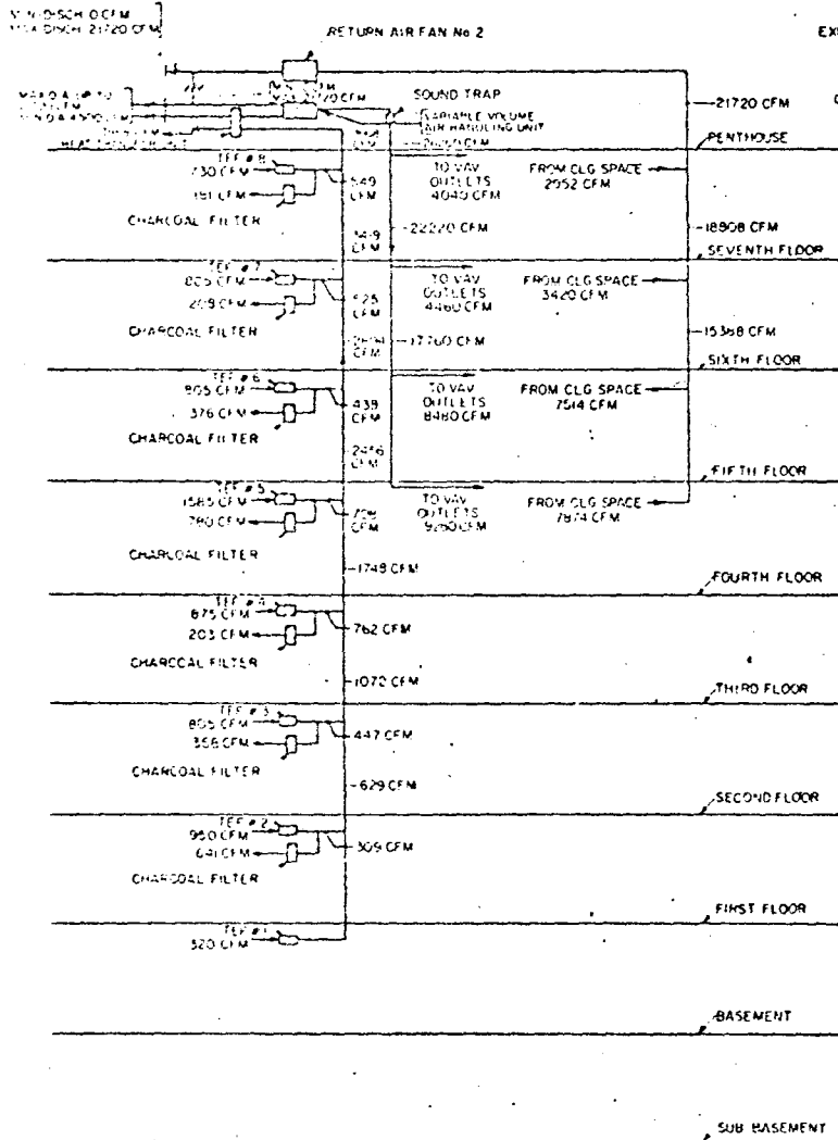
DUCT FLOW DIAGRAM CENTRAL VAV SYSTEM NO SCALE
