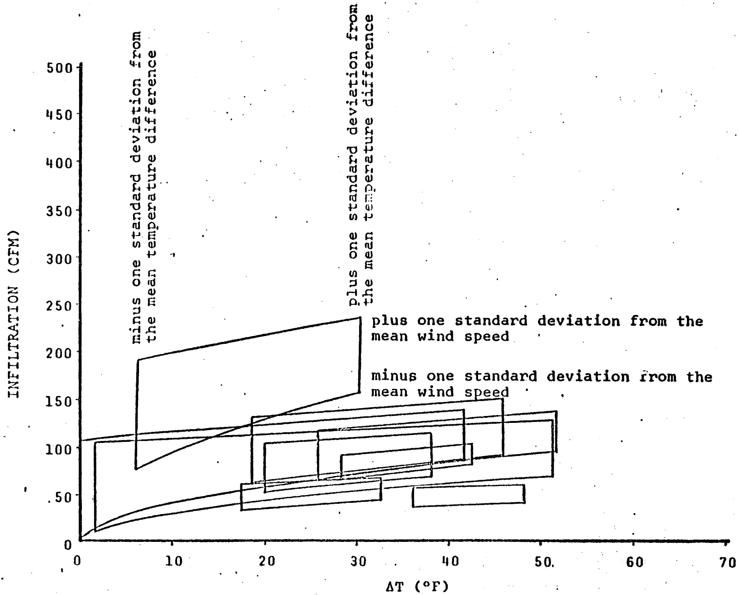
FIGURE 9.5.4.: COMPOSITE OVERLAY OF THE MEASURED DATA RANGES
