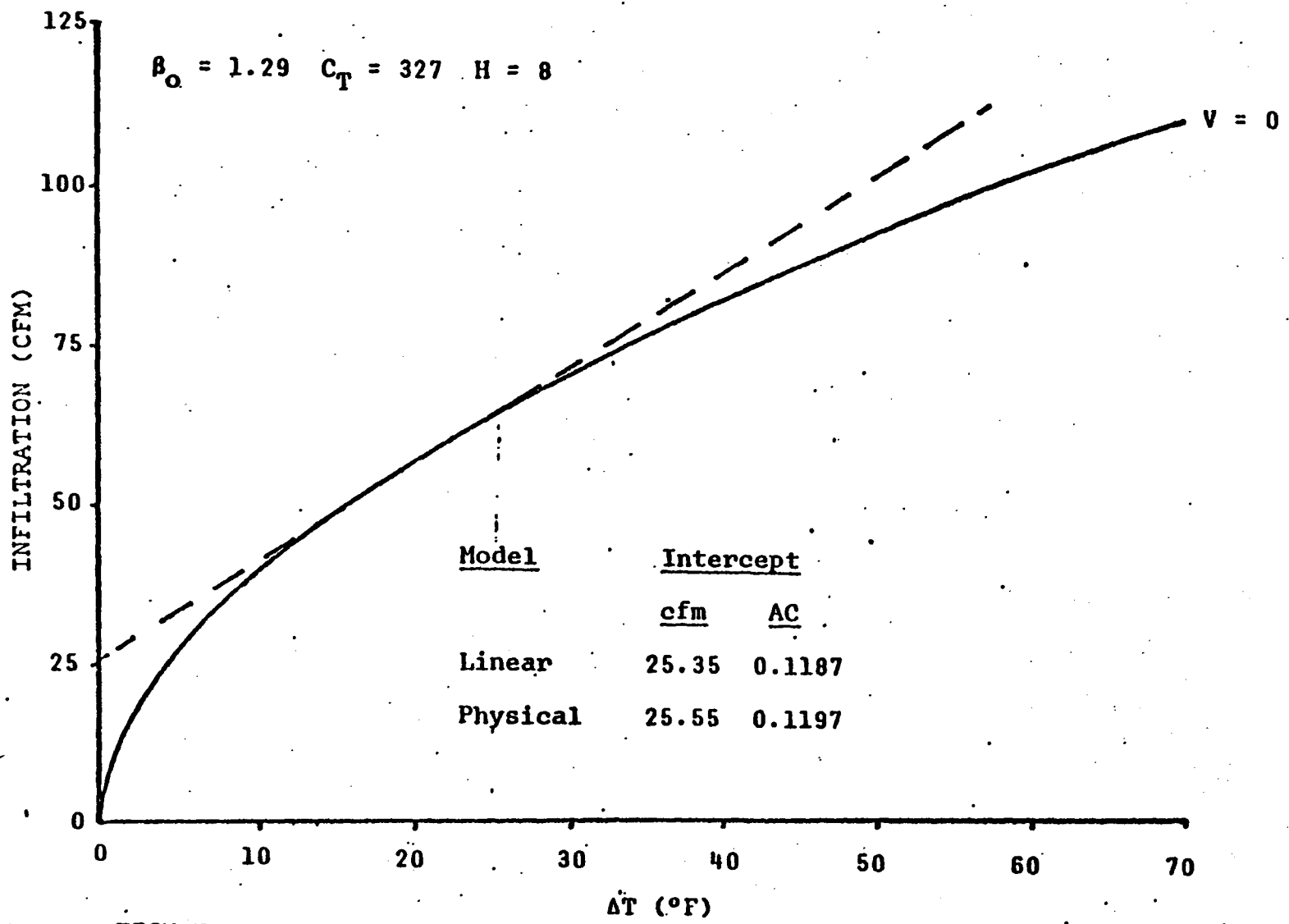
FIGURE 9.5.6: PHYSICAL VS LINEAR MODEL TEMPERATURE EFFORTS
