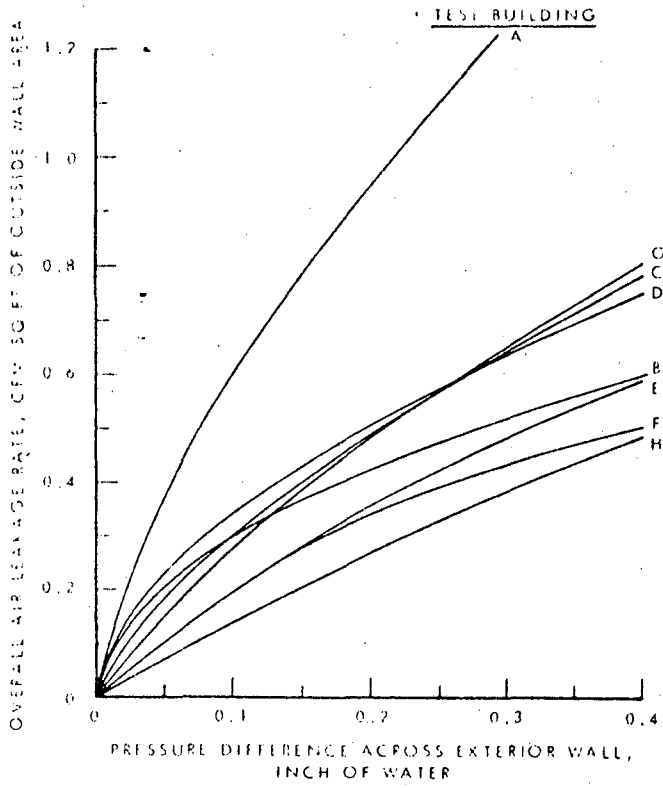
Fig. 2 Over-all air leakage rates of pressurized enclosure
