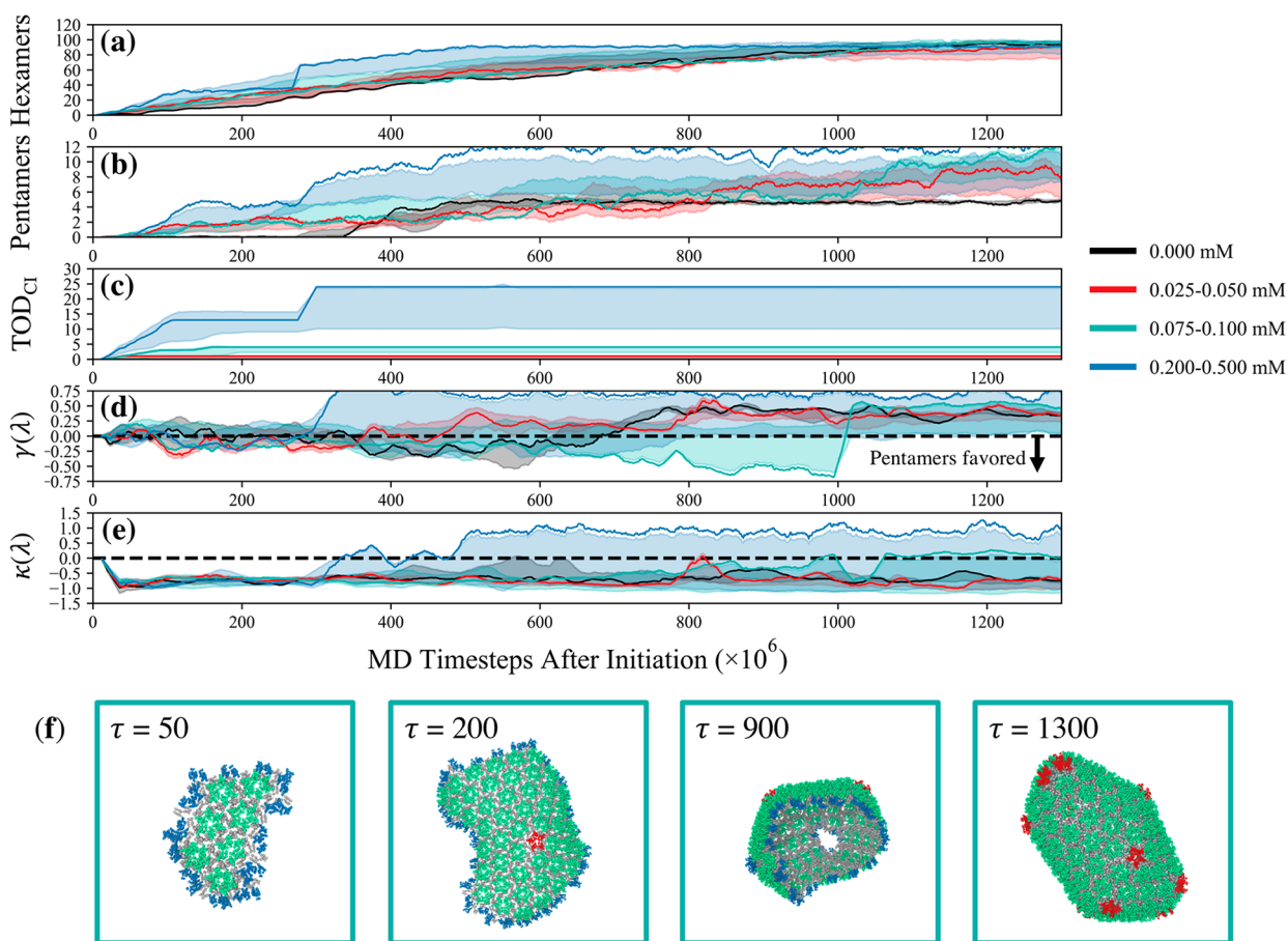
Figure 3. Assembly time-series plots that depict (a) the number of assembled hexamers, (b) the number of assembled pentamers, (c) the number of incorporated inhibitor-bound TODs ( \text{TOD}_{\text{CI}} ), and the (d) skew ( \gamma(\lambda) ) and (e) kurtosis ( \kappa(\lambda) ) of the distribution of eccentricities ( \lambda ) throughout the assembled lattice as a function of CG MD time step (shifted with respect to the onset of lattice growth) for each system within the listed concentration of capsid inhibitors (CIs). We find accelerated assembly, especially with respect to pentamers, in the CI-present simulations, which appear to be commensurate with negative \gamma(\lambda) and \kappa(\lambda) , i.e., a descriptor that indicates anisotropic edge growth in the protein lattice. The shaded region depicts the standard deviation around the mean from four trajectories within the listed range of concentrations while the solid line depicts a single trajectory. In (f), molecular snapshots of the protein lattice for the 0.100 mM case (green line in (a)–(e)) at the listed MD time step ( \tau \times 10^6 ) are shown; green, red, and blue NTD domains in capsomers indicate hexamers, pentamers, and incomplete capsomers, respectively.
