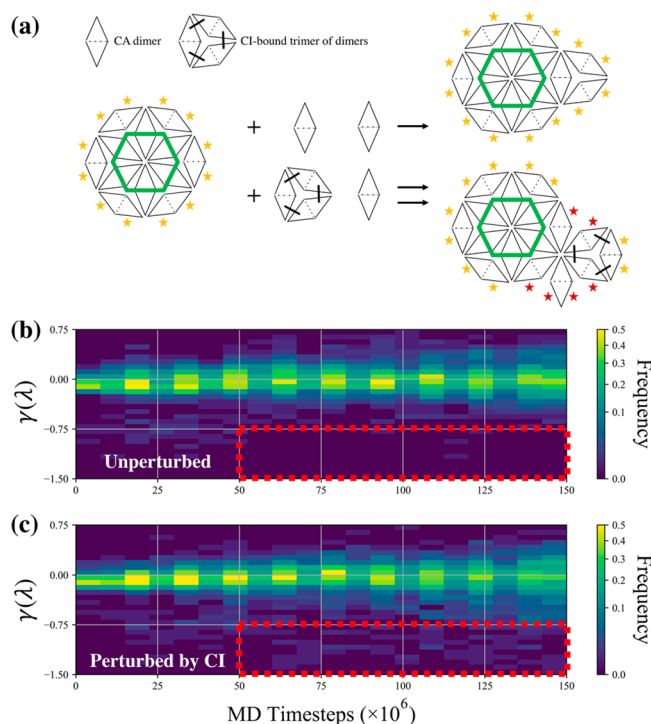
Figure 4. (a) Schematic of the canonical assembly pathway (top) through the dual association of CA dimers and accelerated assembly pathway (bottom) through the association of a trimer of dimers (TOD) that is stabilized by capsid inhibitors (CIs) and a CA dimer. The stars represent potential binding interfaces; yellow stars indicate the need for an adjacent CA dimer to associate nearly simultaneously, while red stars indicate sites that are energetically satisfied by a single CA dimer. The topological character of an assembling lattice over time is quantified by the skew of its eccentricities ( \gamma(\lambda) ) with distributions calculated from a swarm of 50 trajectories in the (b) absence and (c) presence of CIs. Here, \gamma(\lambda) \approx 0 is suggestive of an open isotropic lattice, \gamma(\lambda) < 0 is suggestive of an open anisotropic lattice, and \gamma(\lambda) > 0 is suggestive of a uniform and oblong lattice (such as in closed mature capsids). These results suggest the preference of isotropic (emergence of anisotropic) lattice growth during canonical (CI-perturbed) assembly, which is highlighted in the region bound by the dashed red box. Each trajectory was discretized into 20 equal bins before histograms were computed ( n = 375 per histogram).
