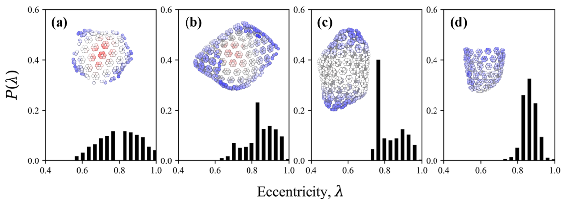
Figure 2. Topology of the assembled CA lattice is assessed by the eccentricity ( \lambda ) of each vertex (i.e., each CA monomer) in a graph representation of the lattice. We show the distribution of \lambda ( P(\lambda) ) at select points during one trajectory of [\text{CA}^+]_{\text{CI}} = 0.100 mM for demonstrative purposes: at (a) 1 \times 10^8 , (b) 7 \times 10^8 , and (c) 14 \times 10^8 MD timesteps. The same analysis is performed in (d) using half of the lattice from (c), i.e., after cleavage by a plane perpendicular to the long axis of the capsid. Representative lattices are depicted as insets in (a-d) with each monomer shown as a sphere colored by its \lambda from red ( \lambda = 0.5 ) to blue ( \lambda = 1.0 ). The topology of the lattice can be qualitatively characterized by the skew of the distribution of \lambda ( \gamma(\lambda) ) in which (a,d) zero skew is indicative of an open lattice with isotropic edges, (b) negative skew is indicative of an open anisotropic lattice, and (c) positive skew is indicative of a closed, non-spherical lattice.
