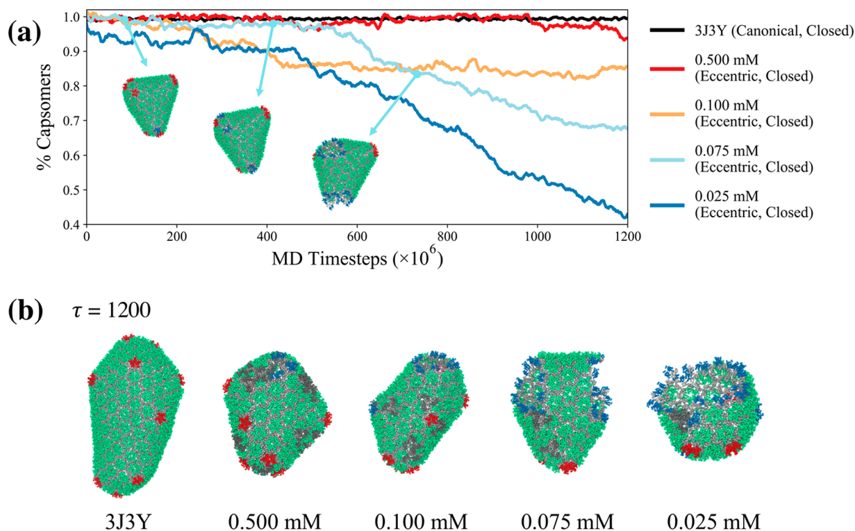
Figure 5. (a) Disassembly time-series plot that depicts the fraction of remaining hexamers and pentamers (with respect to the initial size of the mature capsid core) for the five listed systems as a function of MD time step. All four of the eccentric cases exhibit spontaneous disassembly, which appear to be initiated at sites with large pentamer density. Molecular snapshots of the protein lattice for the 0.075 mM case (cyan line in (a)) at the indicated points are shown; green, red, and blue capsomers indicate hexamers, pentamers, and incomplete capsomers, respectively. (b) Molecular snapshots from each trajectory at the indicated MD time step ( \tau \times 10^6 ) are shown. The inhibitor-bound TODs are represented as gray capsomers. This data suggests that capsid inhibitors promote the formation of “leaky” mature cores that spontaneously open at regions of high curvature (or high pentamer density), and represents one failure mechanism that suppresses infectivity.
