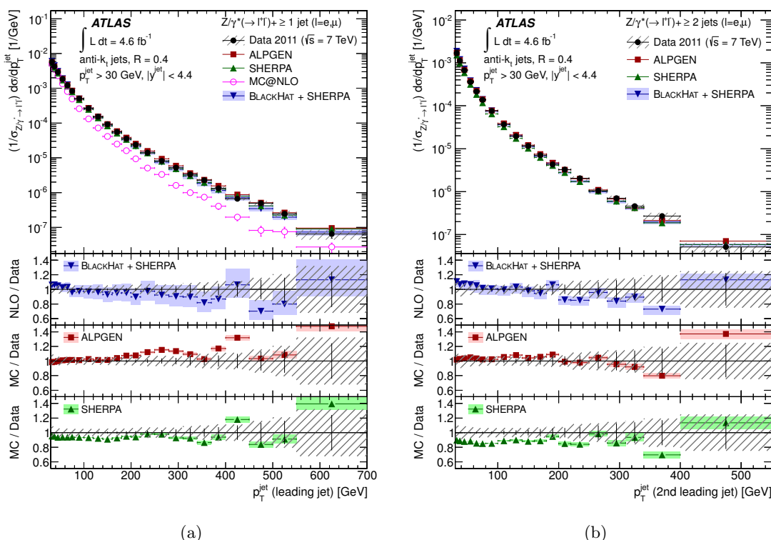
Figure 5. (a) Measured cross section for Z(\rightarrow \ell\ell) + jets as a function of the transverse momentum, p_T^{jet} , of the leading jet for events with at least one jet with p_T^{jet} > 30 GeV and |y^{jet}| < 4.4 in the final state and (b) as a function of p_T^{jet} of the second leading jet for events with at least two jets. The cross sections are normalized to the inclusive Z(\rightarrow \ell\ell) cross section. The other details are as in figure 2.
