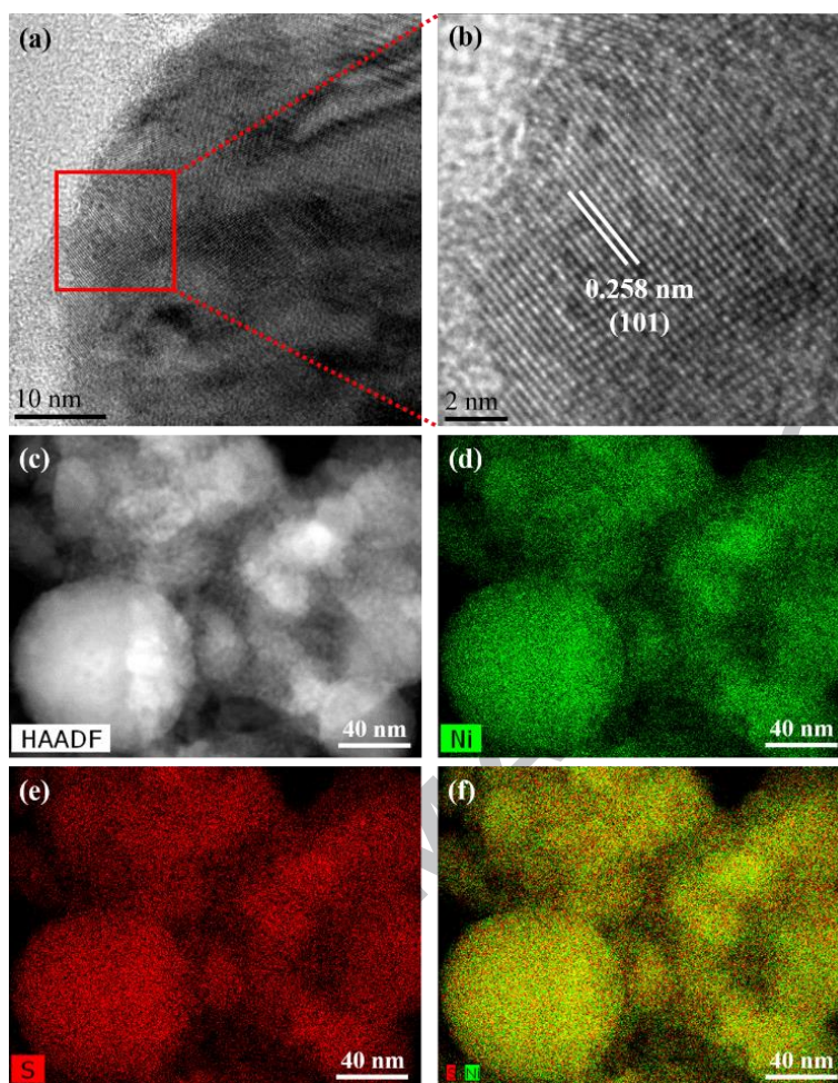
Fig. 2. (a) High-resolution TEM micrograph, (b) lattice fringe, (c) HAADF-STEM image and (d)-(f) corresponding EDX elemental maps of NiS-4h. Scale bars of (a), (b) and (c)-(f) are 10 nm, 2 nm and 40 nm, respectively.
