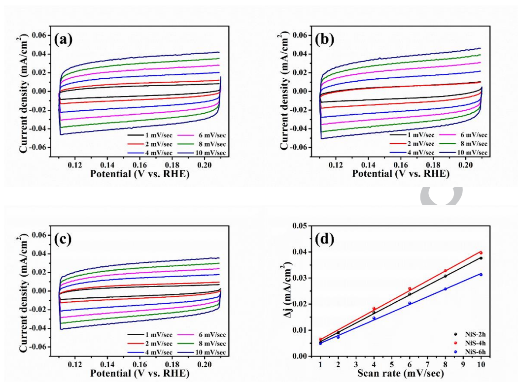
Fig. 5. Cyclic voltammograms of (a) NiS-2h, (b) NiS-4h and (c) NiS-6h recorded in 0.11 - 0.21 V vs. RHE at scan rates from 1 to 10 mV/sec in N_2 -saturated 1 M KOH electrolyte. (d) Scan rate dependence of the current densities of NiS-2h ( \bullet ), NiS-4h ( \bullet ) and NiS-6h ( \bullet ) at 0.16 V vs. RHE and their corresponding linear fittings (solid lines).
