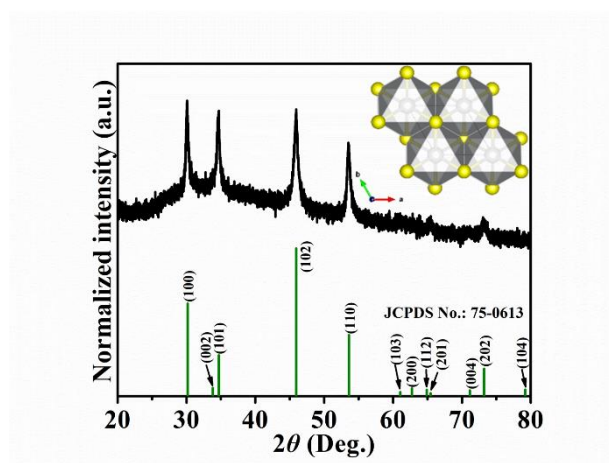
Fig. 1. XRD pattern of NiS-4h, the inset illustrates the corresponding crystal structure.
