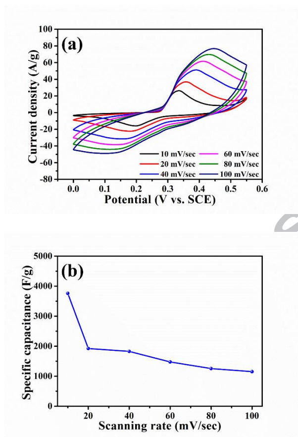
Fig. 6. (a) Cyclic voltammograms and (b) average specific capacitances of NiS-4h recorded in 0 - 0.55 V vs. SCE at scan rates from 10 to 100 mV/sec in N 2 -saturated 6 M KOH electrolyte.
