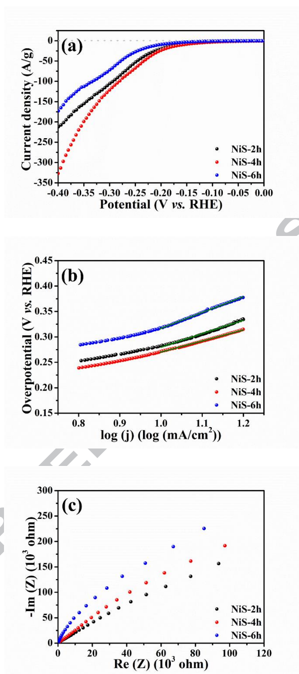
Fig. 4. (a) Linear sweep voltammograms, (b) Tafel plots and (c) electrochemical impedance spectra of NiS-2h (•), NiS-4h (•) and NiS-6h (•) collected in a \text{N}_2 -saturated 1 M KOH electrolyte.
