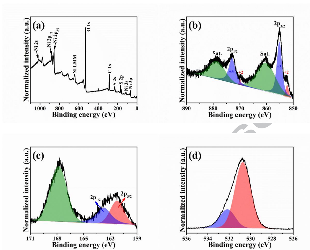
Fig. 3. XPS analysis of NiS-4h: (a) Full-range survey and high-resolution (b) Ni 2p, (c) S 2p, and (d) O 1s spectra. The green, blue and red peaks in (b) are the shark-up satellites, Ni 3+ and Ni 2+ signals, respectively. The green, blue and red peaks of (c) represent the sulfate, S 2p 1/2 and S 2p 3/2 peaks. The blue and red peaks in (d) correspond to the Ni 3+ OOH and Ni 2+ SO 4 .
